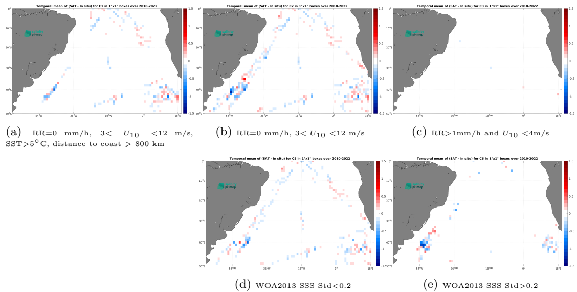
Figure 12: Temporal mean gridded over spatial boxes of size 1^\circ \times 1^\circ of \Delta SSS (CCI SSS L4 Merged-OI v4.4 - 30-day running (ESA) - TSG (Polarstern)) for 5 different subdatasets corresponding to:RR=0 mm/h, 3 < U_{10} < 12 m/s, SST >5^\circ\text{C} , distance to coast > 800 km (a), RR=0 mm/h, 3 < U_{10} < 12 m/s (b), RR >1 mm/h and U_{10} < 4 m/s (c), WOA2013 SSS Std <0.2 (d), WOA2013 SSS Std >0.2 (e).
