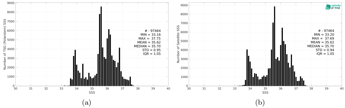
Figure 2: Histograms of SSS from TSG (Polarstern) (a) and CCI SSS L4 Merged-OI v4.4 - 30-day running (ESA) (b) considering all match-up pairs per bins of 0.1 over the South Atlantic Ocean Pi-MEP region and for the full satellite product period.
