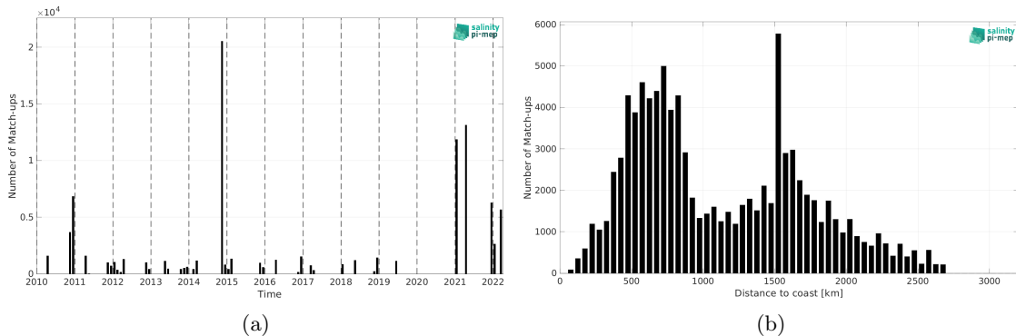
Figure 1: Number of match-ups between TSG (Polarstern) and CCI SSS L4 Merged-OI v4.4 - 30-day running (ESA) SSS as a function of time (a) and as function of the distance to coast (b) over the South Atlantic Ocean Pi-MEP region and for the full satellite product period.
