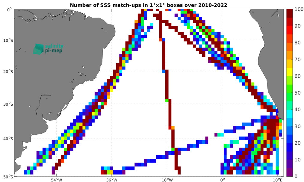
Figure 4: Number of SSS match-ups between TSG (Polarstern) SSS and the CCI SSS L4 Merged-OI v4.4 - 30-day running (ESA) SSS product for the South Atlantic Ocean Pi-MEP region over 1^\circ \times 1^\circ boxes and for the full satellite product period.
