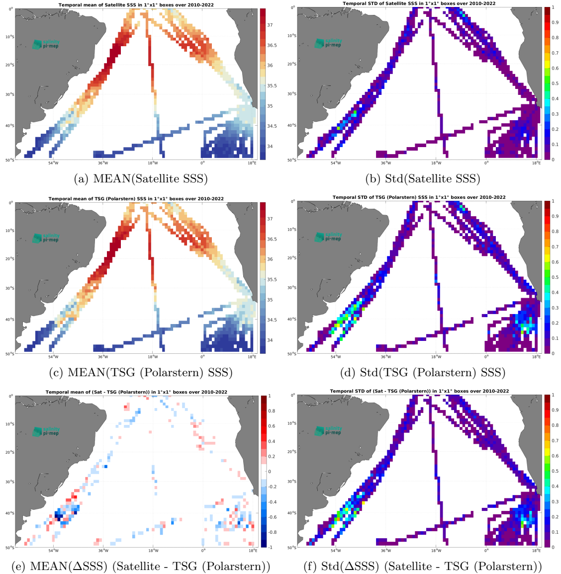
Figure 6: Temporal mean (left) and Std (right) of SSS from CCI SSS L4 Merged-OI v4.4 - 30-day running (ESA) (top), TSG (Polarstern) (middle), and of \Delta SSS (Satellite - TSG (Polarstern)). Only match-up pairs are used to generate these maps.
