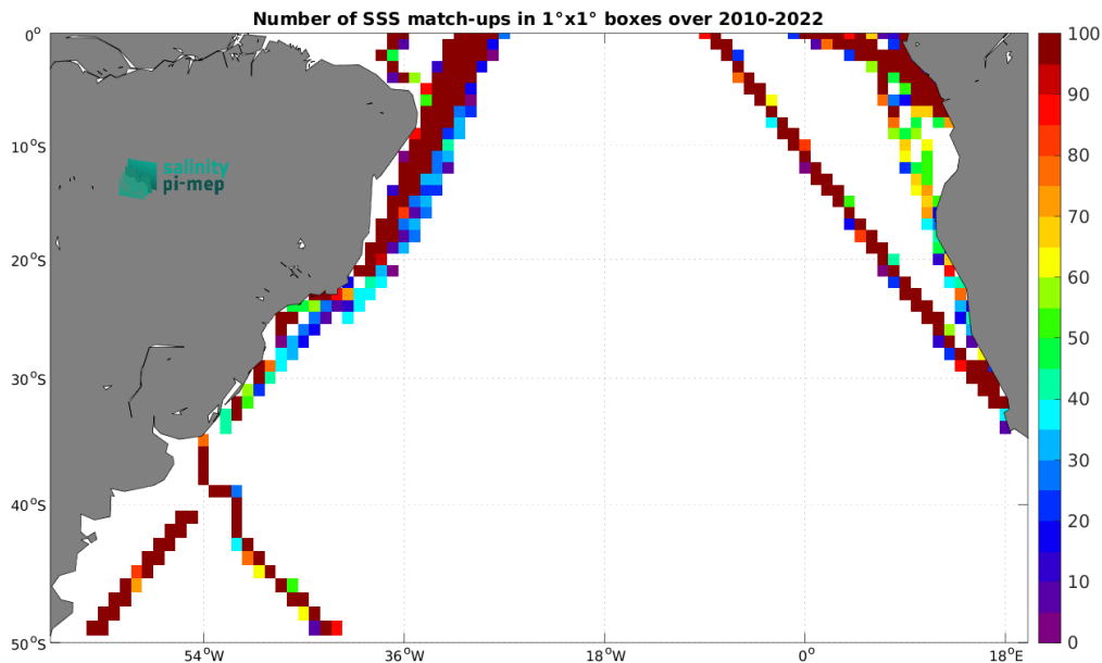
Figure 4: Number of SSS match-ups between TSG (LEGOS-DM) SSS and the CCI SSS L4 Merged-OI v4.4 - 30-day running (ESA) SSS product for the South Atlantic Ocean Pi-MEP region over 1^\circ \times 1^\circ boxes and for the full satellite product period.
