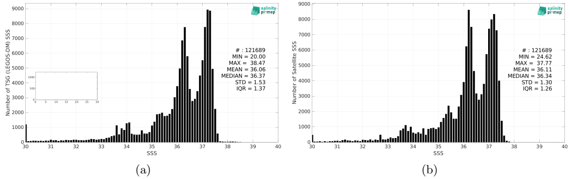
Figure 2: Histograms of SSS from TSG (LEGOS-DM) (a) and CCI SSS L4 Merged-OI v4.4 - 30-day running (ESA) (b) considering all match-up pairs per bins of 0.1 over the South Atlantic Ocean Pi-MEP region and for the full satellite product period.
