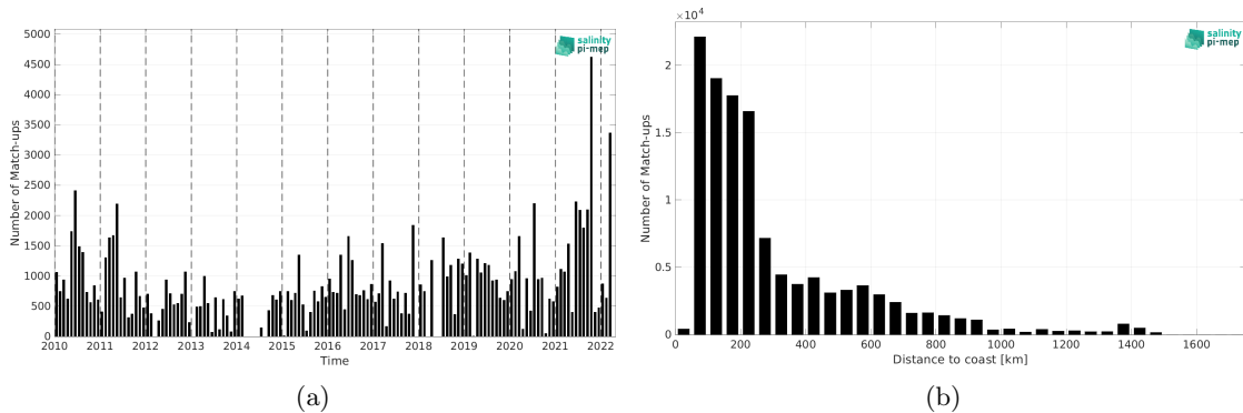
Figure 1: Number of match-ups between TSG (LEGOS-DM) and CCI SSS L4 Merged-OI v4.4 - 30-day running (ESA) SSS as a function of time (a) and as function of the distance to coast (b) over the South Atlantic Ocean Pi-MEP region and for the full satellite product period.
