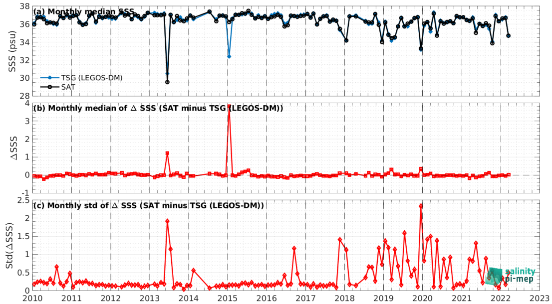
Figure 7: Time series of the monthly median SSS (top), median of \Delta\text{SSS} (Satellite - TSG (LEGOS-DM)) and Std of \Delta\text{SSS} (Satellite - TSG (LEGOS-DM)) over the South Atlantic Ocean Pi-MEP region considering all match-ups collected by the Pi-MEP.
