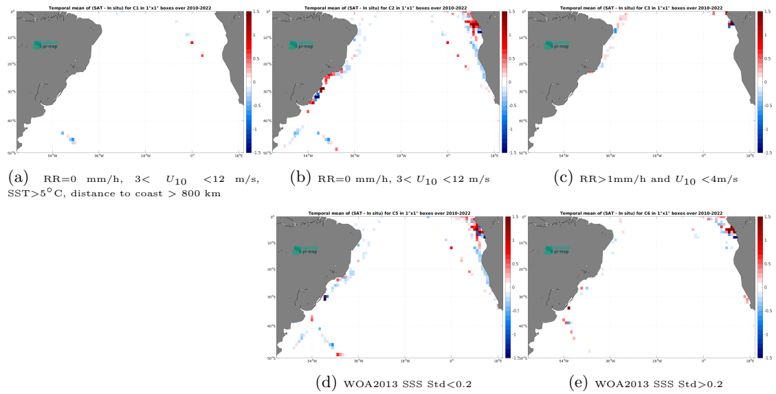
Figure 12: Temporal mean gridded over spatial boxes of size 1^\circ \times 1^\circ of \Delta SSS (CCI SSS L4 Merged-OI v4.4 - 30-day running (ESA) - TSG (LEGOS-DM)) for 5 different subdatasets corresponding to:RR=0 mm/h, 3 < U_{10} < 12 m/s, SST >5^\circ\text{C} , distance to coast > 800 km (a), RR=0 mm/h, 3 < U_{10} < 12 m/s (b), RR >1 mm/h and U_{10} < 4 m/s (c), WOA2013 SSS Std <0.2 (d), WOA2013 SSS Std >0.2 (e).
