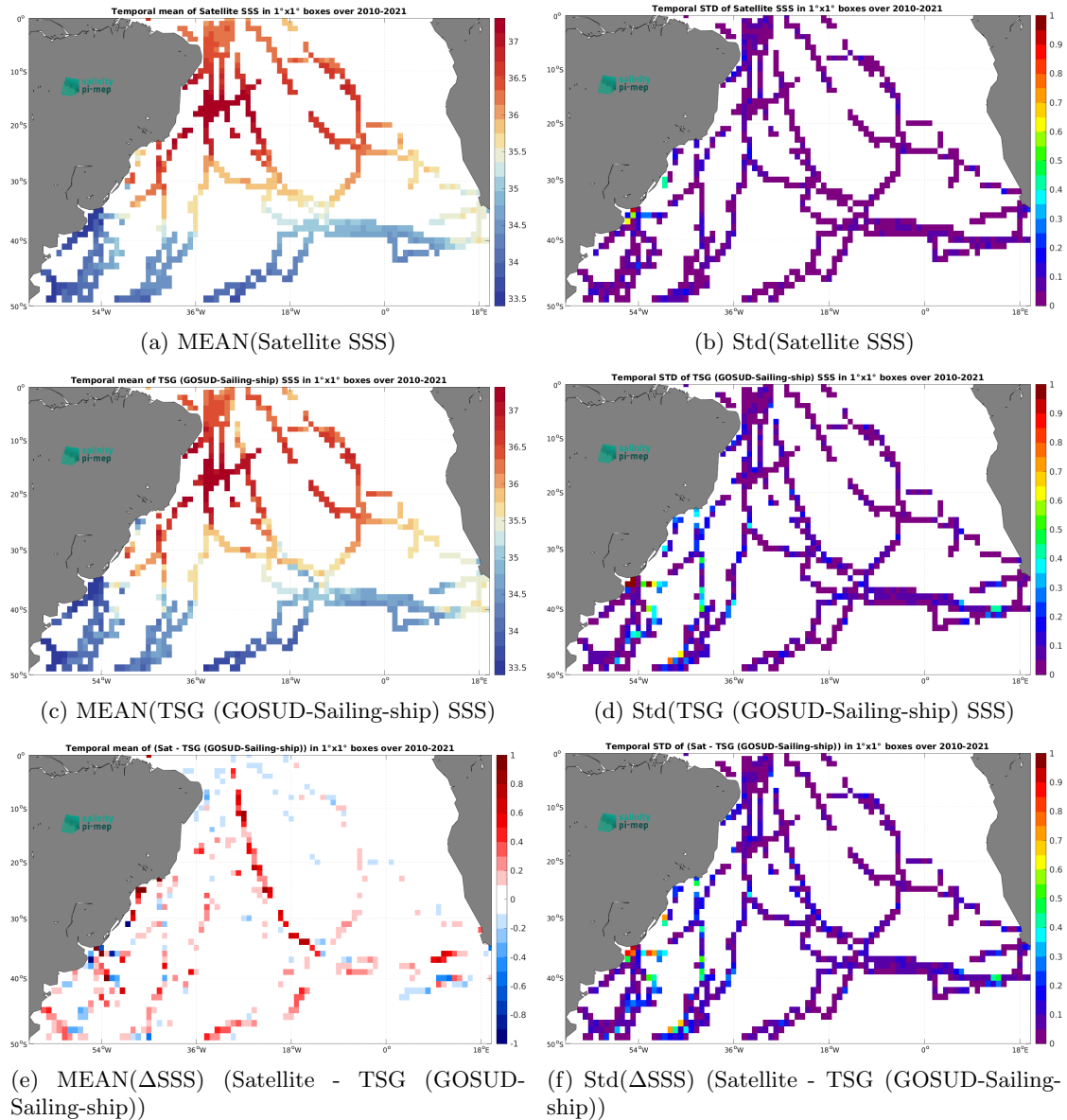
Figure 6: Temporal mean (left) and Std (right) of SSS from CCI SSS L4 Merged-OI v4.4 - 30-day running (ESA) (top), TSG (GOSUD-Sailing-ship) (middle), and of \Delta SSS (Satellite - TSG (GOSUD-Sailing-ship)). Only match-up pairs are used to generate these maps.
