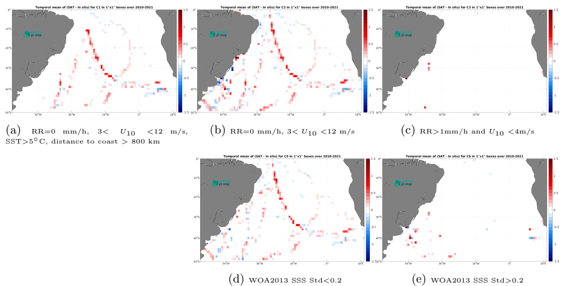
Figure 12: Temporal mean gridded over spatial boxes of size 1^\circ \times 1^\circ of \Delta SSS (CCI SSS L4 Merged-OI v4.4 - 30-day running (ESA) - TSG (GOSUD-Sailing-ship)) for 5 different subdatasets corresponding to:RR=0 mm/h, 3 < U_{10} < 12 m/s, SST >5^\circ\text{C} , distance to coast > 800 km (a), RR=0 mm/h, 3 < U_{10} < 12 m/s (b), RR >1 mm/h and U_{10} < 4 m/s (c), WOA2013 SSS Std <0.2 (d), WOA2013 SSS Std >0.2 (e).
