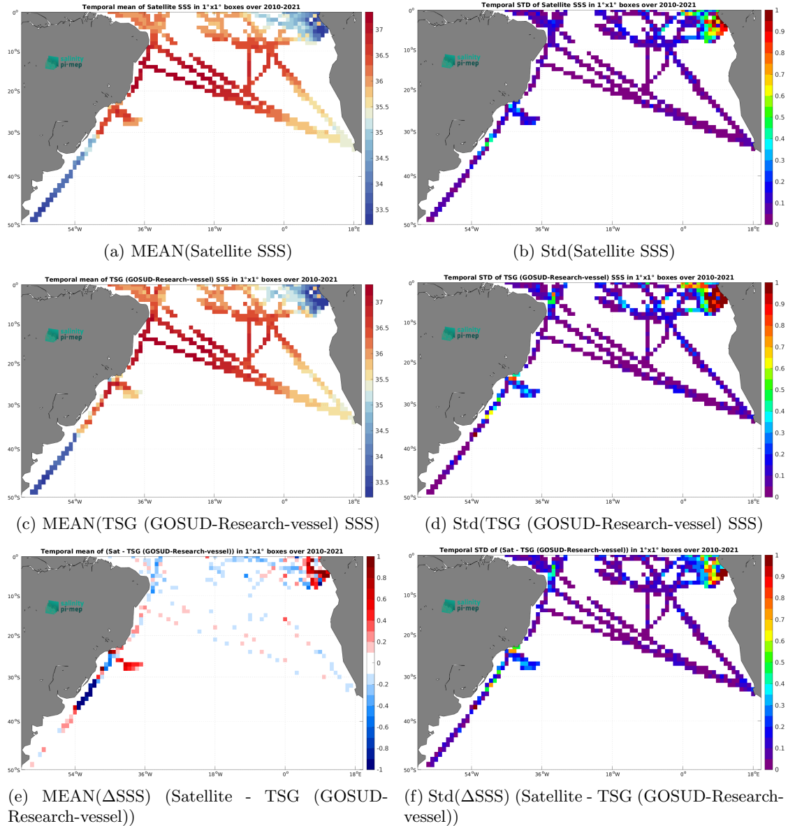
Figure 6: Temporal mean (left) and Std (right) of SSS from CCI SSS L4 Merged-OI v4.4 - 30-day running (ESA) (top), TSG (GOSUD-Research-vessel) (middle), and of \Delta SSS (Satellite - TSG (GOSUD-Research-vessel)). Only match-up pairs are used to generate these maps.
