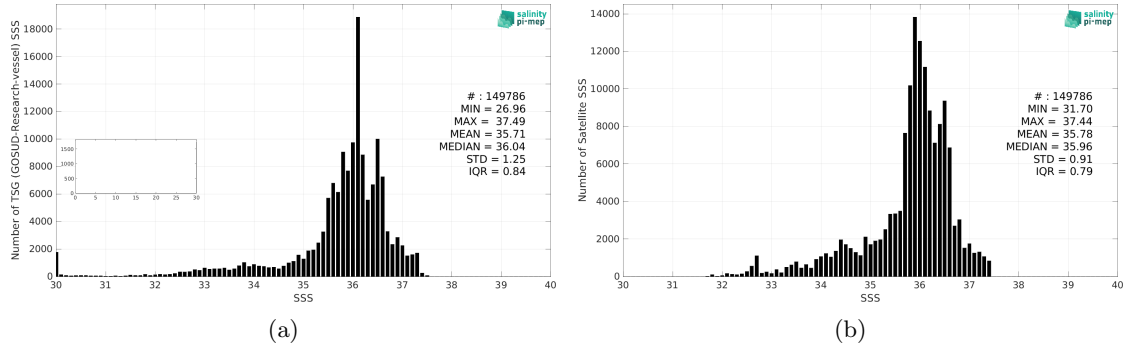
Figure 2: Histograms of SSS from TSG (GOSUD-Research-vessel) (a) and CCI SSS L4 Merged-OI v4.4 - 30-day running (ESA) (b) considering all match-up pairs per bins of 0.1 over the South Atlantic Ocean Pi-MEP region and for the full satellite product period.
