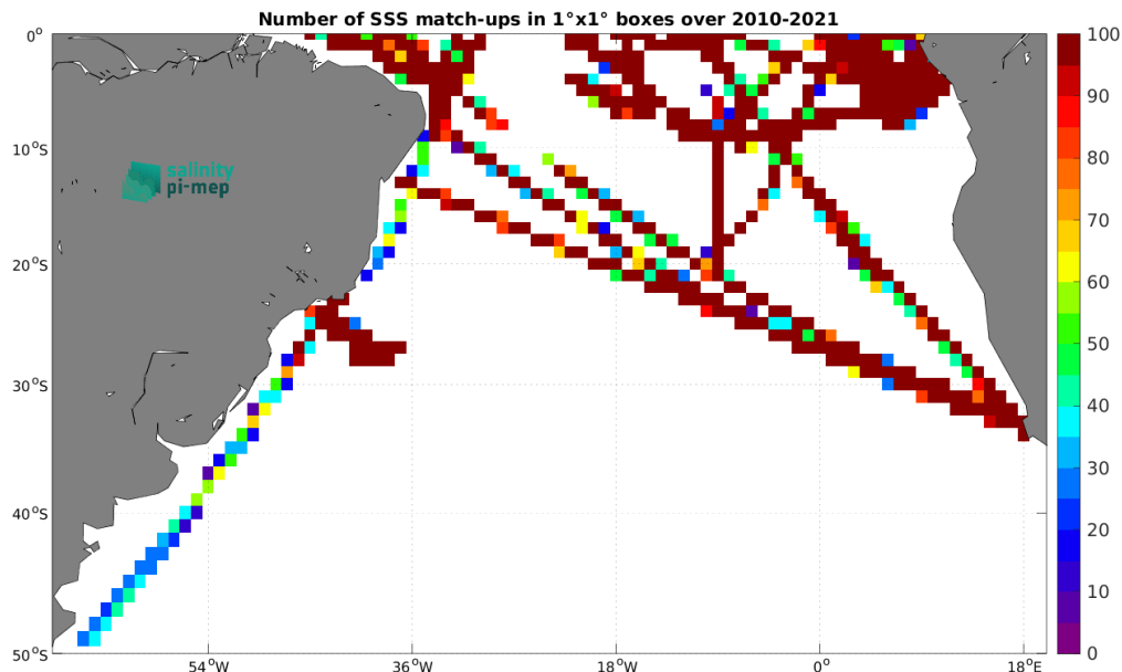
Figure 4: Number of SSS match-ups between TSG (GOSUD-Research-vessel) SSS and the CCI SSS L4 Merged-OI v4.4 - 30-day running (ESA) SSS product for the South Atlantic Ocean Pi-MEP region over 1^\circ \times 1^\circ boxes and for the full satellite product period.
