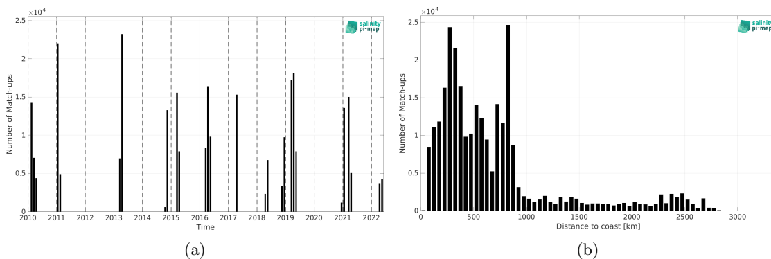
Figure 1: Number of match-ups between TSG (CSIC-UTM) and CCI SSS L4 Merged-OI v4.4 - 30-day running (ESA) SSS as a function of time (a) and as function of the distance to coast (b) over the South Atlantic Ocean Pi-MEP region and for the full satellite product period.
