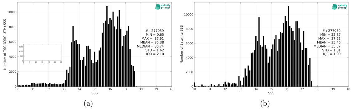
Figure 2: Histograms of SSS from TSG (CSIC-UTM) (a) and CCI SSS L4 Merged-OI v4.4 - 30-day running (ESA) (b) considering all match-up pairs per bins of 0.1 over the South Atlantic Ocean Pi-MEP region and for the full satellite product period.
