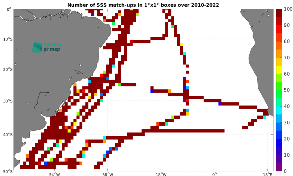
Figure 4: Number of SSS match-ups between TSG (CSIC-UTM) SSS and the CCI SSS L4 Merged-OI v4.4 - 30-day running (ESA) SSS product for the South Atlantic Ocean Pi-MEP region over 1^\circ \times 1^\circ boxes and for the full satellite product period.
