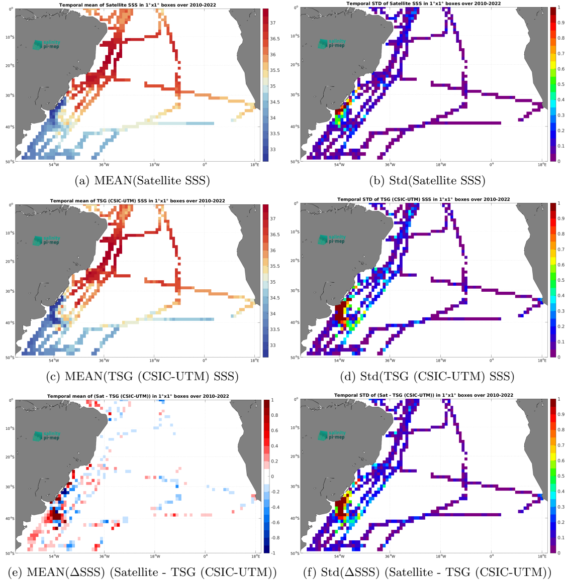
Figure 6: Temporal mean (left) and Std (right) of SSS from CCI SSS L4 Merged-OI v4.4 - 30-day running (ESA) (top), TSG (CSIC-UTM) ( in situ ) dataset (middle), and of \Delta SSS (Satellite - TSG (CSIC-UTM)). Only match-up pairs are used to generate these maps.
