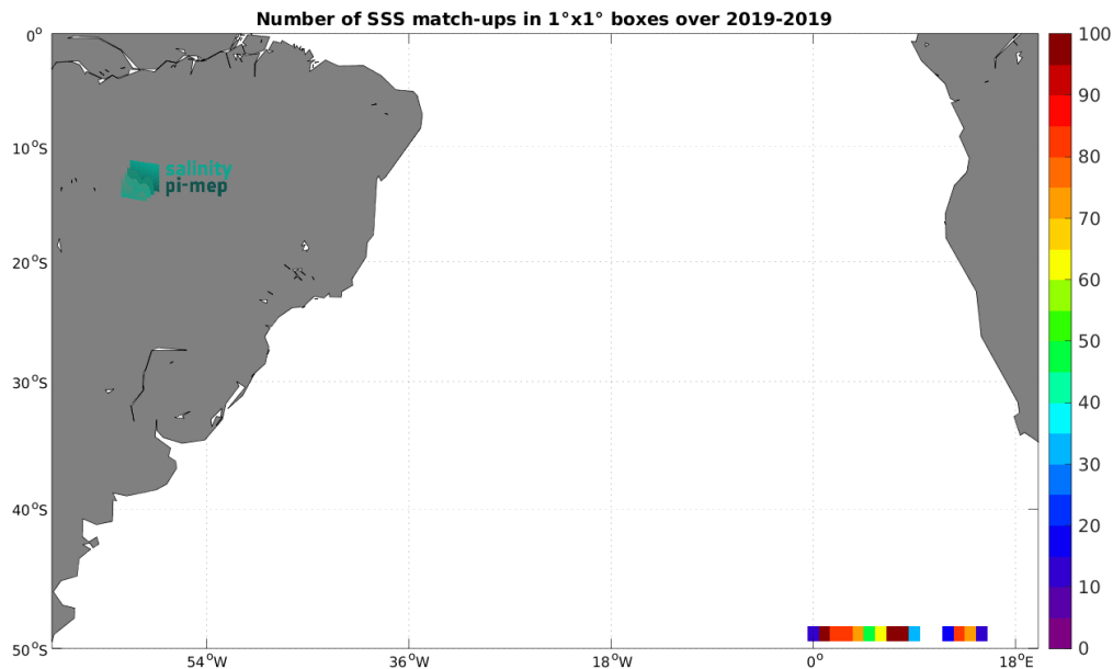
Figure 4: Number of SSS match-ups between Saildrone SSS and the CCI SSS L4 Merged-OI v4.4 - 30-day running (ESA) SSS product for the South Atlantic Ocean Pi-MEP region over 1^\circ \times 1^\circ boxes and for the full satellite product period.
