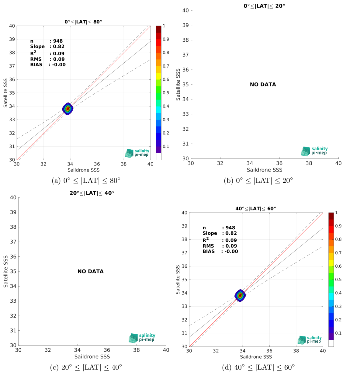
Figure 9: Contour maps of the concentration of CCI SSS L4 Merged-OI v4.4 - 30-day running (ESA) SSS (y-axis) versus Saildrone SSS (x-axis) at match-up pairs for different latitude bands. For each plot, the red line shows x=y . The black thin and dashed lines indicate a linear fit through the data cloud and the \pm 95\% confidence levels, respectively. The number match-up pairs n , the slope and R^2 coefficient of the linear fit, the root mean square (RMS) and the mean bias between satellite and in situ data are indicated for each latitude band in each plots.
