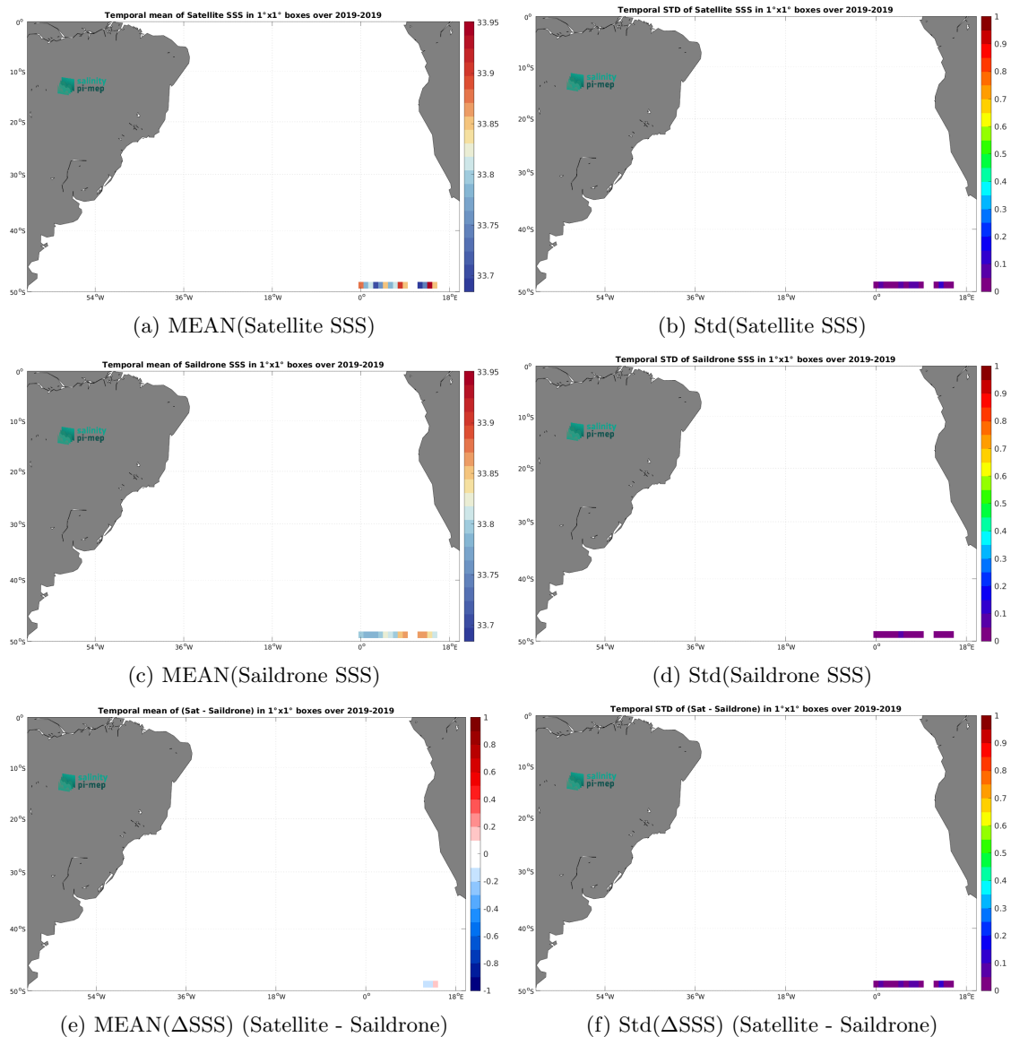
Figure 6: Temporal mean (left) and Std (right) of SSS from CCI SSS L4 Merged-OI v4.4 - 30-day running (ESA) (top), Saildrone (middle), and of \Delta SSS (Satellite - Saildrone). Only match-up pairs are used to generate these maps.
