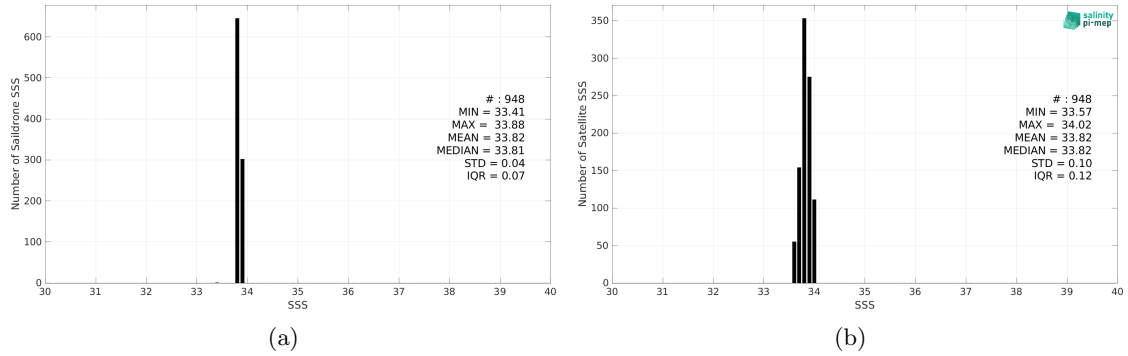
Figure 2: Histograms of SSS from Saildrone (a) and CCI SSS L4 Merged-OI v4.4 - 30-day running (ESA) (b) considering all match-up pairs per bins of 0.1 over the South Atlantic Ocean Pi-MEP region and for the full satellite product period.
