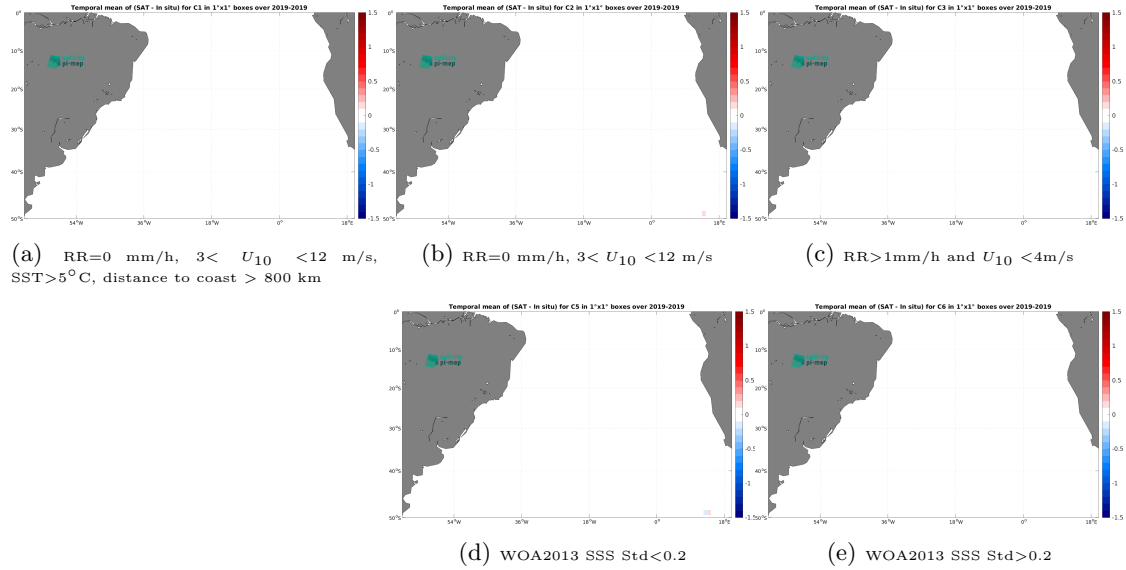
Figure 12: Temporal mean gridded over spatial boxes of size 1^{\circ}\times 1^{\circ} of \Delta\text{SSS} (CCI SSS L4 Merged-OI v4.4 - 30-day running (ESA) - Saildrone) for 5 different subdatasets corresponding to:RR=0 mm/h, 3 < U_{10} < 12 m/s, SST >5^{\circ}\text{C} , distance to coast > 800 km (a), RR=0 mm/h, 3 < U_{10} < 12 m/s (b), RR >1 mm/h and U_{10} < 4 m/s (c), WOA2013 SSS Std <0.2 (d), WOA2013 SSS Std >0.2 (e).
