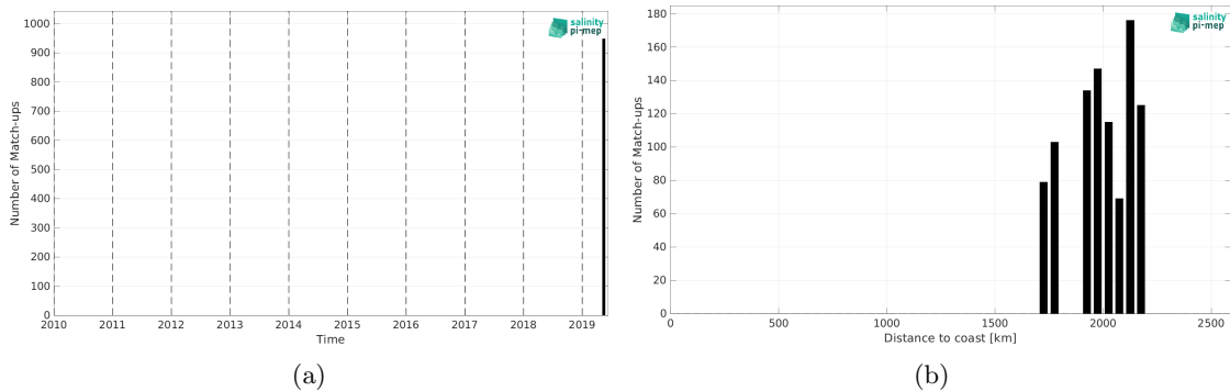
Figure 1: Number of match-ups between Saildrone and CCI SSS L4 Merged-OI v4.4 - 30-day running (ESA) SSS as a function of time (a) and as function of the distance to coast (b) over the South Atlantic Ocean Pi-MEP region and for the full satellite product period.
