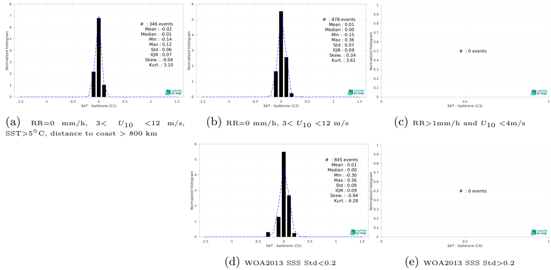
Figure 13: Normalized histogram of \Delta SSS (CCI SSS L4 Merged-OI v4.4 - 30-day running (ESA) - Saildrone) for 5 different subdatasets corresponding to: RR=0 mm/h, 3 < U_{10} < 12 m/s, SST >5^{\circ} C, distance to coast > 800 km (a), RR=0 mm/h, 3 < U_{10} < 12 m/s (b), RR >1 mm/h and U_{10} < 4 m/s (c), WOA2013 SSS Std <0.2 (d), WOA2013 SSS Std >0.2 (e).
