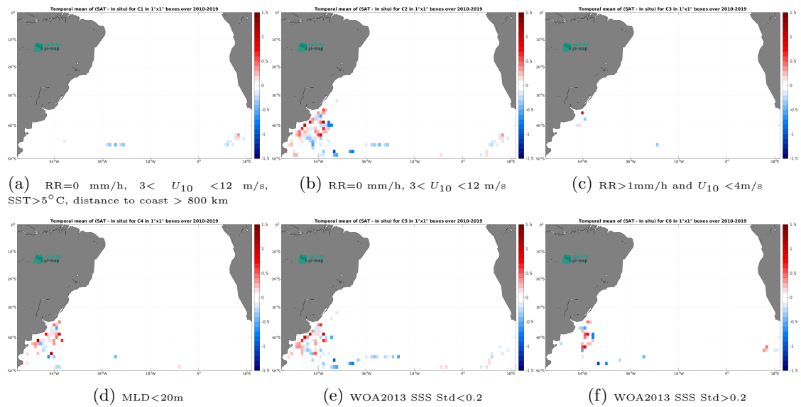
Figure 12: Temporal mean gridded over spatial boxes of size 1^\circ \times 1^\circ of \Delta SSS (CCI SSS L4 Merged-OI v4.4 - 30-day running (ESA) - Marine mammals) for 6 different subdatasets corresponding to:RR=0 mm/h, 3 < U_{10} < 12 m/s, SST >5^\circ C, distance to coast > 800 km (a), RR=0 mm/h, 3 < U_{10} < 12 m/s (b), RR >1 mm/h and U_{10} < 4 m/s (c),MLD <20 m (d),WOA2013 SSS Std <0.2 (e),WOA2013 SSS Std >0.2 (f).
