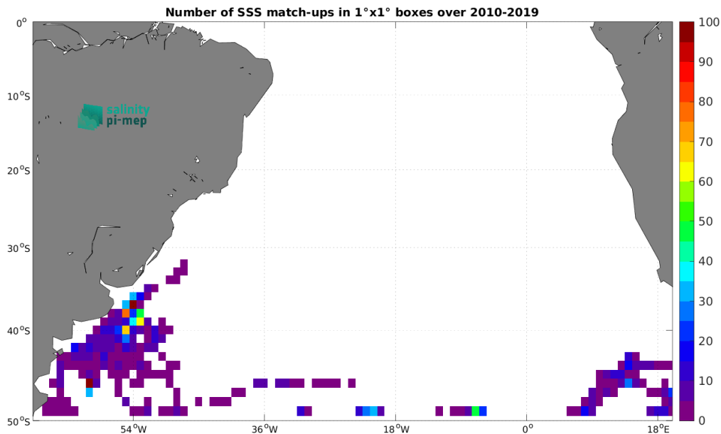
Figure 4: Number of SSS match-ups between Marine mammals SSS and the CCI SSS L4 Merged-OI v4.4 - 30-day running (ESA) SSS product for the South Atlantic Ocean Pi-MEP region over 1^\circ \times 1^\circ boxes and for the full satellite product period.
