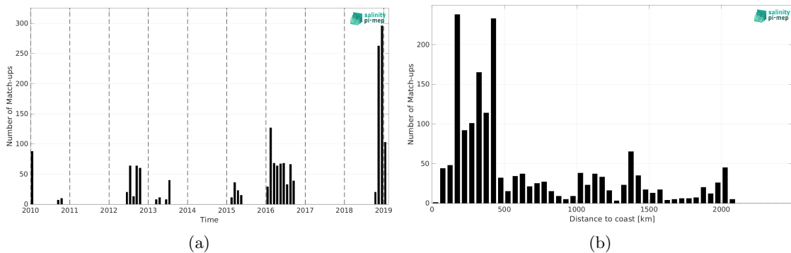
Figure 1: Number of match-ups between Marine mammals and CCI SSS L4 Merged-OI v4.4 - 30-day running (ESA) SSS as a function of time (a) and as function of the distance to the coast (b) over the South Atlantic Ocean Pi-MEP region and for the full satellite product period.
