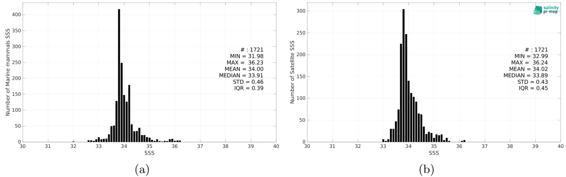
Figure 2: Histograms of SSS from Marine mammals (a) and CCI SSS L4 Merged-OI v4.4 - 30-day running (ESA) (b) considering all match-up pairs per bins of 0.1 over the South Atlantic Ocean Pi-MEP region and for the full satellite product period.
