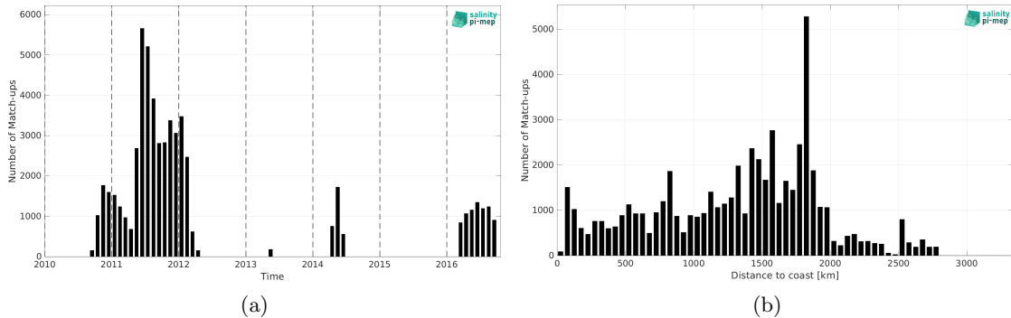
Figure 1: Number of match-ups between Surface drifters and CCI SSS L4 Merged-OI v4.4 - 30-day running (ESA) SSS as a function of time (a) and as function of the distance to coast (b) over the South Atlantic Ocean Pi-MEP region and for the full satellite product period.
