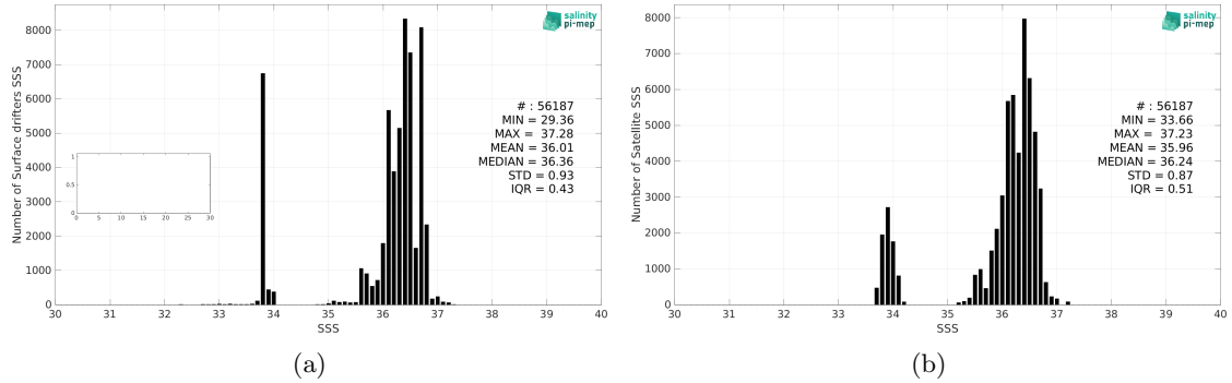
Figure 2: Histograms of SSS from Surface drifters (a) and CCI SSS L4 Merged-OI v4.4 - 30-day running (ESA) (b) considering all match-up pairs per bins of 0.1 over the South Atlantic Ocean Pi-MEP region and for the full satellite product period.
