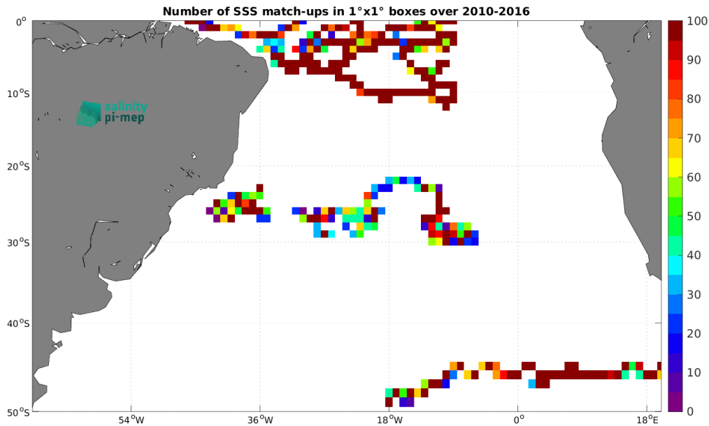
Figure 3: Number of SSS match-ups between Surface drifters SSS and the CCI SSS L4 Merged-OI v4.4 - 30-day running (ESA) SSS product for the South Atlantic Ocean Pi-MEP region over 1^\circ \times 1^\circ boxes and for the full satellite product period.
