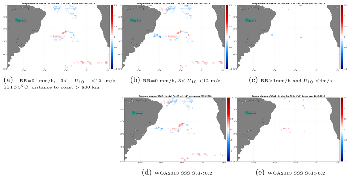
Figure 11: Temporal mean gridded over spatial boxes of size 1^\circ \times 1^\circ of \Delta SSS (CCI SSS L4 Merged-OI v4.4 - 30-day running (ESA) - Surface drifters) for 5 different subdatasets corresponding to:RR=0 mm/h, 3 < U_{10} < 12 m/s, SST >5^\circ C, distance to coast > 800 km (a), RR=0 mm/h, 3 < U_{10} < 12 m/s (b), RR >1 mm/h and U_{10} < 4 m/s (c), WOA2013 SSS Std <0.2 (d), WOA2013 SSS Std >0.2 (e).
