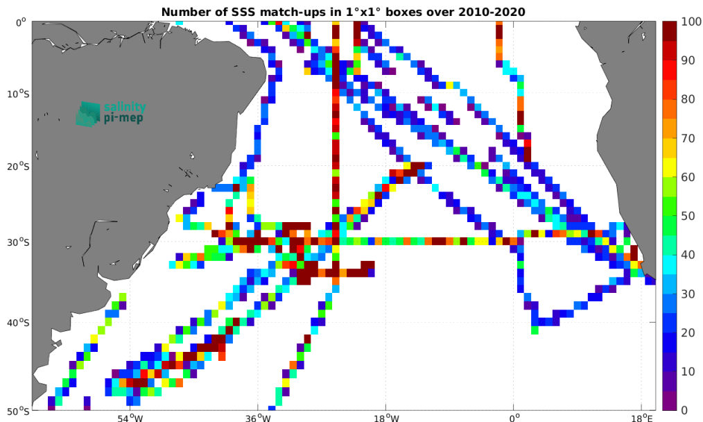
Figure 4: Number of SSS match-ups between TSG (SAMOS) SSS and the CCI SSS L4 Merged-OI v3.2 - 7-day running (ESA) SSS product for the South Atlantic Ocean Pi-MEP region over 1^\circ \times 1^\circ boxes and for the full satellite product period.
