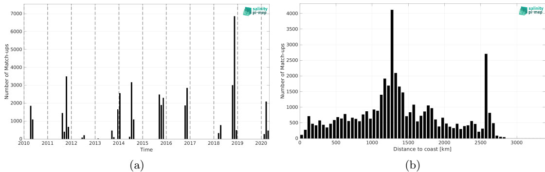
Figure 1: Number of match-ups between TSG (SAMOS) and CCI SSS L4 Merged-OI v3.2 - 7-day running (ESA) SSS as a function of time (a) and as function of the distance to coast (b) over the South Atlantic Ocean Pi-MEP region and for the full satellite product period.
