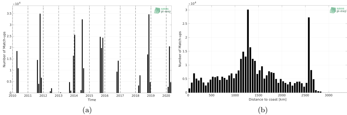
Figure 1: Number of match-ups between TSG (SAMOS) and CCI SSS L4 Merged-OI v3.2 - 7-day running (ESA) SSS as a function of time (a) and as function of the distance to coast (b) over the South Atlantic Ocean Pi-MEP region and for the full satellite product period.
