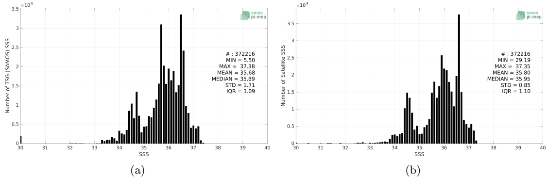
Figure 2: Histograms of SSS from TSG (SAMOS) (a) and CCI SSS L4 Merged-OI v3.2 - 7-day running (ESA) (b) considering all match-up pairs per bins of 0.1 over the South Atlantic Ocean Pi-MEP region and for the full satellite product period.
