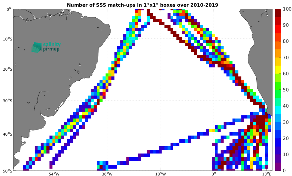
Figure 4: Number of SSS match-ups between TSG (Polarstern) SSS and the CCI SSS L4 Merged-OI v3.2 - 7-day running (ESA) SSS product for the South Atlantic Ocean Pi-MEP region over 1^\circ \times 1^\circ boxes and for the full satellite product period.
