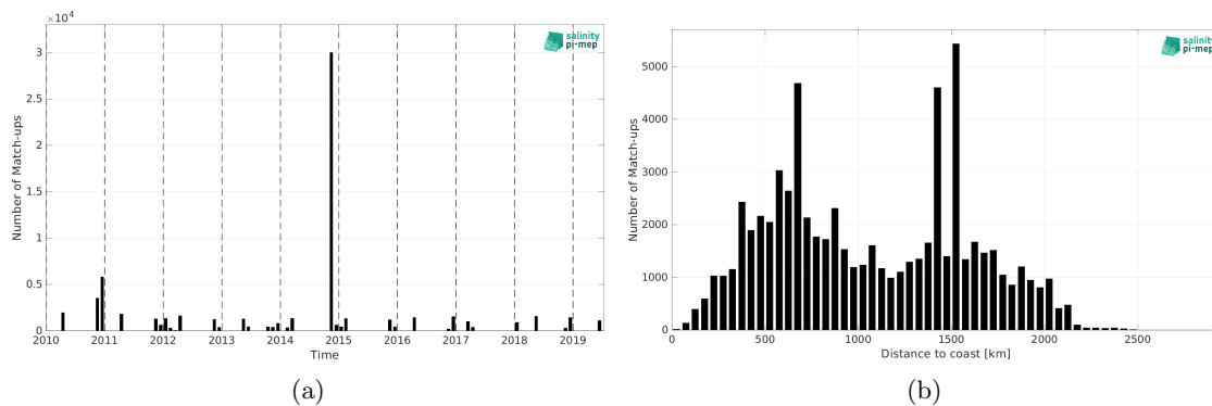
Figure 1: Number of match-ups between TSG (Polarstern) and CCI SSS L4 Merged-OI v3.2 - 7-day running (ESA) SSS as a function of time (a) and as function of the distance to coast (b) over the South Atlantic Ocean Pi-MEP region and for the full satellite product period.
