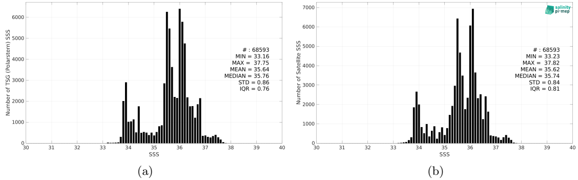
Figure 2: Histograms of SSS from TSG (Polarstern) (a) and CCI SSS L4 Merged-OI v3.2 - 7-day running (ESA) (b) considering all match-up pairs per bins of 0.1 over the South Atlantic Ocean Pi-MEP region and for the full satellite product period.
