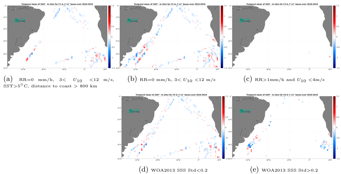
Figure 12: Temporal mean gridded over spatial boxes of size 1^\circ \times 1^\circ of \Delta\text{SSS} (CCI SSS L4 Merged-OI v3.2 - 7-day running (ESA) - TSG (Polarstern)) for 5 different subdatasets corresponding to:RR=0 mm/h, 3 < U_{10} < 12 m/s, SST >5^\circ\text{C} , distance to coast > 800 km (a), RR=0 mm/h, 3 < U_{10} < 12 m/s (b), RR >1 mm/h and U_{10} < 4 m/s (c), WOA2013 SSS Std <0.2 (d), WOA2013 SSS Std >0.2 (e).
