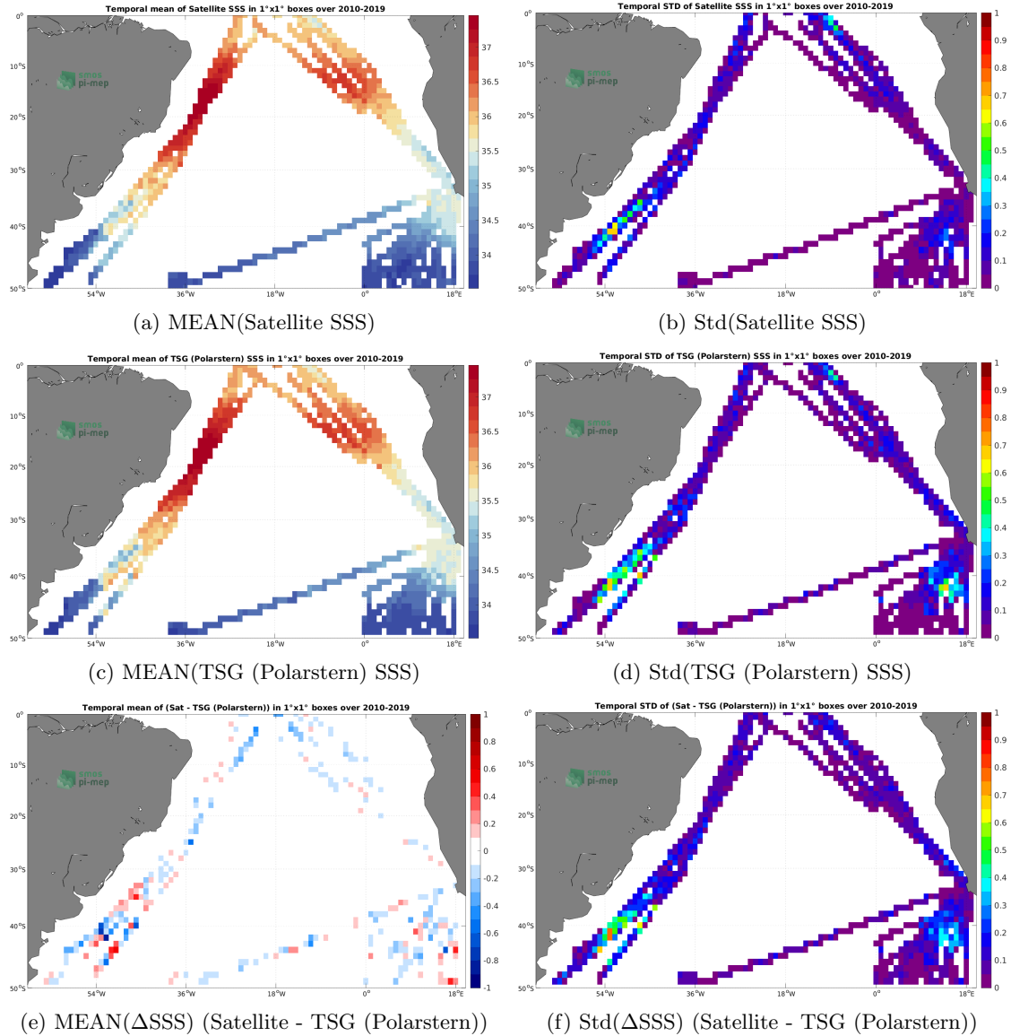
Figure 6: Temporal mean (left) and Std (right) of SSS from CCI SSS L4 Merged-OI v3.2 - 7-day running (ESA) (top), TSG (Polarstern) (middle), and of \Delta SSS (Satellite - TSG (Polarstern)). Only match-up pairs are used to generate these maps.
