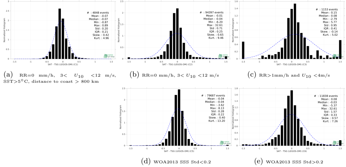
Figure 13: Normalized histogram of \Delta\text{SSS} (CCI SSS L4 Merged-OI v3.2 - 7-day running (ESA) - TSG (LEGOS-DM)) for 5 different subdatasets corresponding to: RR=0 mm/h, 3 < U_{10} < 12 m/s, SST>5°C, distance to coast > 800 km (a), RR=0 mm/h, 3 < U_{10} < 12 m/s (b), RR>1mm/h and U_{10} < 4 m/s (c), WOA2013 SSS Std<0.2 (d), WOA2013 SSS Std>0.2 (e).
