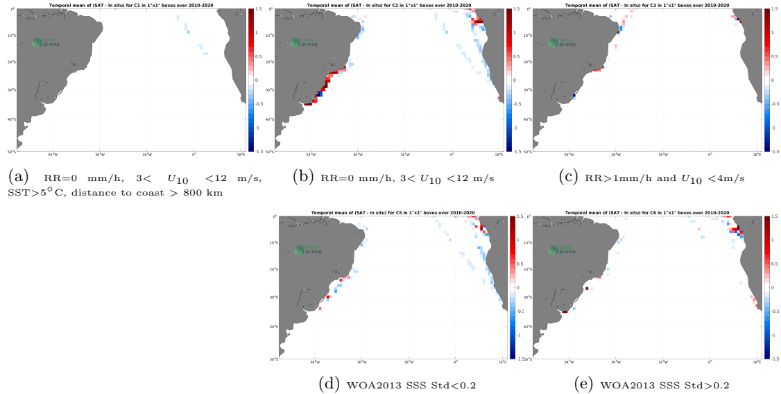
Figure 12: Temporal mean gridded over spatial boxes of size 1^{\circ}\times 1^{\circ} of \Delta\text{SSS} (CCI SSS L4 Merged-OI v3.2 - 7-day running (ESA) - TSG (LEGOS-DM)) for 5 different subdatasets corresponding to:RR=0 mm/h, 3 < U_{10} < 12 m/s, SST >5^{\circ}\text{C} , distance to coast > 800 km (a), RR=0 mm/h, 3 < U_{10} < 12 m/s (b), RR >1 mm/h and U_{10} < 4 m/s (c), WOA2013 SSS Std <0.2 (d), WOA2013 SSS Std >0.2 (e).
