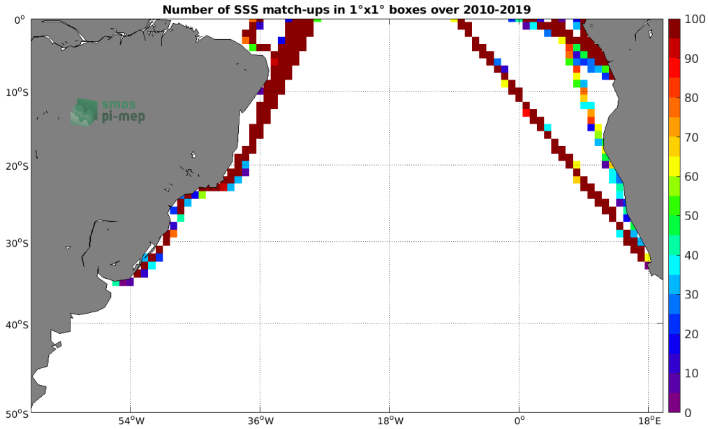
Figure 4: Number of SSS match-ups between TSG (LEGOS-DM) SSS and the CCI SSS L4 Merged-OI v3.2 - 7-day running (ESA) SSS product for the South Atlantic Ocean Pi-MEP region over 1°x1° boxes and for the full satellite product period.
