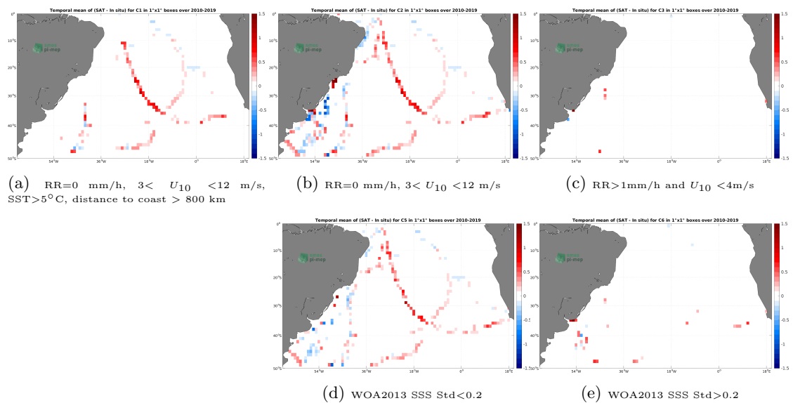
Figure 12: Temporal mean gridded over spatial boxes of size 1^\circ \times 1^\circ of \Delta\text{SSS} (CCI SSS L4 Merged-OI v3.2 - 7-day running (ESA) - TSG (GOSUD-Sailing-ship)) for 5 different subdatasets corresponding to:RR=0 mm/h, 3 < U_{10} < 12 m/s, SST>5°C, distance to coast > 800 km (a), RR=0 mm/h, 3 < U_{10} < 12 m/s (b), RR>1mm/h and U_{10} < 4 m/s (c), WOA2013 SSS Std<0.2 (d), WOA2013 SSS Std>0.2 (e).
