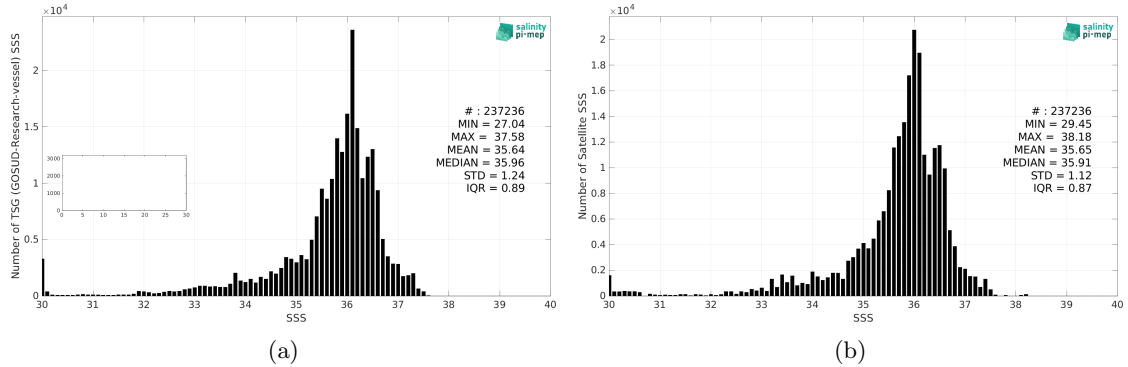
Figure 2: Histograms of SSS from TSG (GOSUD-Research-vessel) (a) and CCI SSS L4 Merged-OI v3.2 - 7-day running (ESA) (b) considering all match-up pairs per bins of 0.1 over the South Atlantic Ocean Pi-MEP region and for the full satellite product period.
