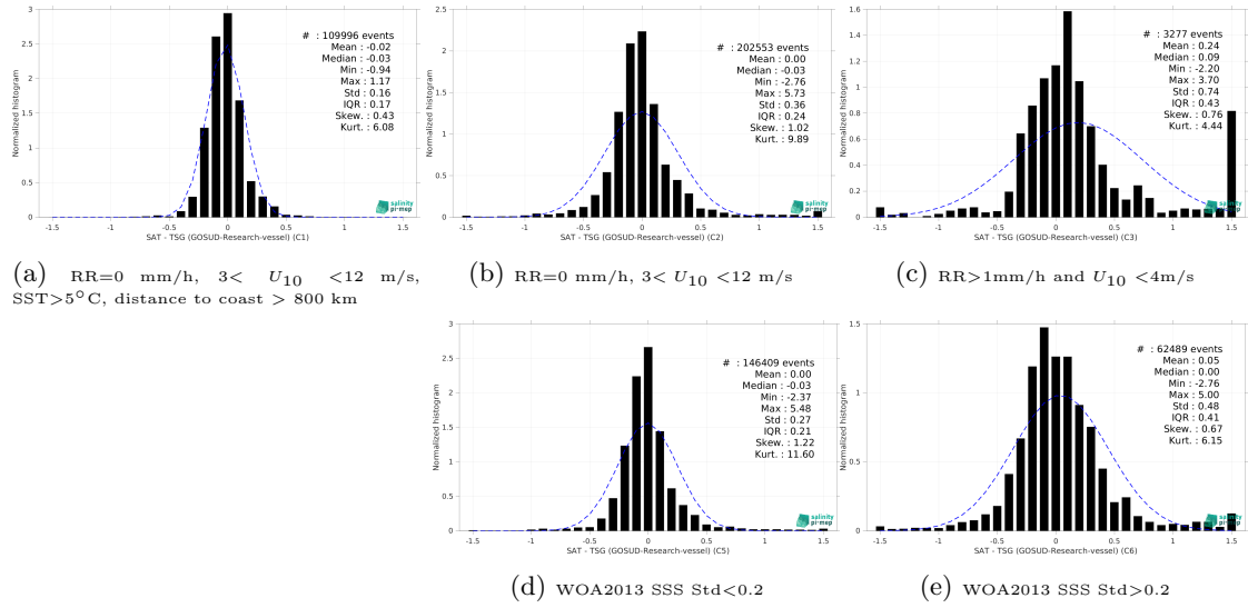
Figure 13: Normalized histogram of \Delta\text{SSS} (CCI SSS L4 Merged-OI v3.2 - 7-day running (ESA) - TSG (GOSUD-Research-vessel)) for 5 different subdatasets corresponding to: RR=0 mm/h, 3 < U_{10} < 12 m/s, SST>5°C, distance to coast > 800 km (a), RR=0 mm/h, 3 < U_{10} < 12 m/s (b), RR>1mm/h and U_{10} < 4 m/s (c), WOA2013 SSS Std<0.2 (d), WOA2013 SSS Std>0.2 (e).
