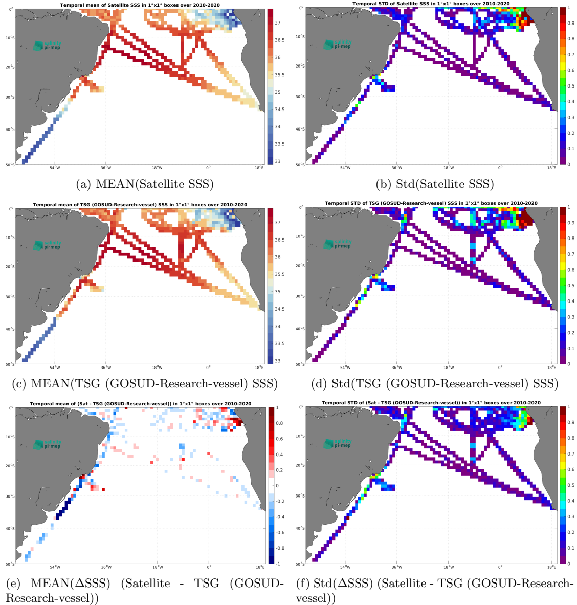
Figure 6: Temporal mean (left) and Std (right) of SSS from CCI SSS L4 Merged-OI v3.2 - 7-day running (ESA) (top), TSG (GOSUD-Research-vessel) (middle), and of \Delta SSS (Satellite - TSG (GOSUD-Research-vessel)). Only match-up pairs are used to generate these maps.
