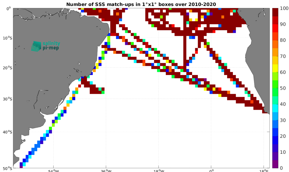
Figure 4: Number of SSS match-ups between TSG (GOSUD-Research-vessel) SSS and the CCI SSS L4 Merged-OI v3.2 - 7-day running (ESA) SSS product for the South Atlantic Ocean Pi-MEP region over 1^\circ \times 1^\circ boxes and for the full satellite product period.
