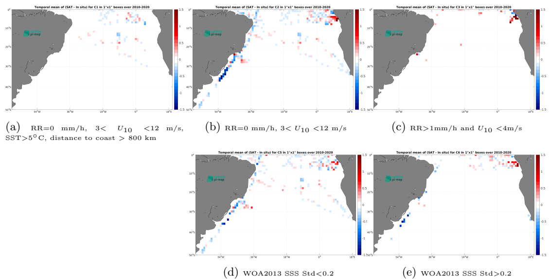
Figure 12: Temporal mean gridded over spatial boxes of size 1^\circ \times 1^\circ of \Delta\text{SSS} (CCI SSS L4 Merged-OI v3.2 - 7-day running (ESA) - TSG (GOSUD-Research-vessel)) for 5 different subdatasets corresponding to:RR=0 mm/h, 3 < U_{10} < 12 m/s, SST>5°C, distance to coast > 800 km (a), RR=0 mm/h, 3 < U_{10} < 12 m/s (b), RR>1mm/h and U_{10} < 4 m/s (c), WOA2013 SSS Std<0.2 (d), WOA2013 SSS Std>0.2 (e).
