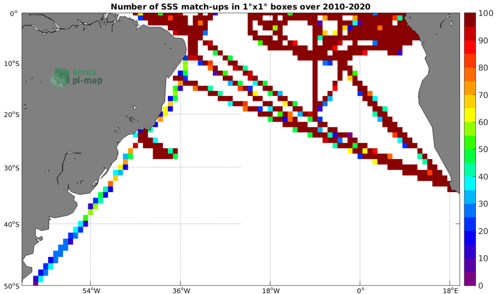
Figure 4: Number of SSS match-ups between TSG (GOSUD-Research-vessel) SSS and the CCI SSS L4 Merged-OI v3.2 - 7-day running (ESA) SSS product for the South Atlantic Ocean Pi-MEP region over 1^{\circ} \times 1^{\circ} boxes and for the full satellite product period.
