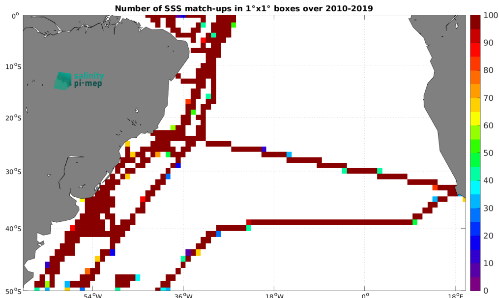
Figure 4: Number of SSS match-ups between TSG (CSIC-UTM) SSS and the CCI SSS L4 Merged-OI v3.2 - 7-day running (ESA) SSS product for the South Atlantic Ocean Pi-MEP region over 1^\circ \times 1^\circ boxes and for the full satellite product period.
