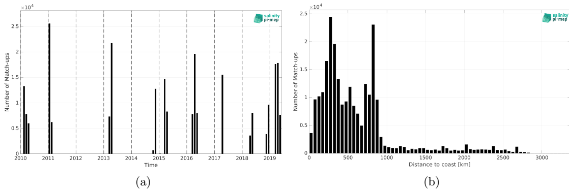
Figure 1: Number of match-ups between TSG (CSIC-UTM) and CCI SSS L4 Merged-OI v3.2 - 7-day running (ESA) SSS as a function of time (a) and as function of the distance to coast (b) over the South Atlantic Ocean Pi-MEP region and for the full satellite product period.
