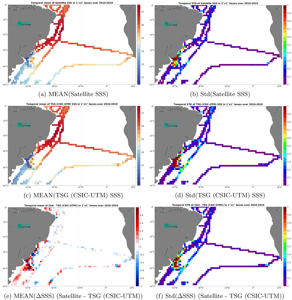
Figure 6: Temporal mean (left) and Std (right) of SSS from CCI SSS L4 Merged-OI v3.2 - 7-day running (ESA) (top), TSG (CSIC-UTM) ( in situ ) dataset (middle), and of \Delta SSS (Satellite - TSG (CSIC-UTM)). Only match-up pairs are used to generate these maps.
