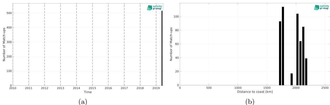
Figure 1: Number of match-ups between Saildrone and CCI SSS L4 Merged-OI v3.2 - 7-day running (ESA) SSS as a function of time (a) and as function of the distance to coast (b) over the South Atlantic Ocean Pi-MEP region and for the full satellite product period.
