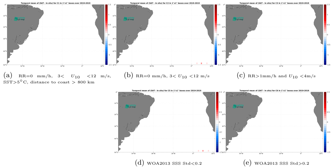
Figure 12: Temporal mean gridded over spatial boxes of size 1^{\circ}\times 1^{\circ} of \Delta\text{SSS} (CCI SSS L4 Merged-OI v3.2 - 7-day running (ESA) - Saildrone) for 5 different subdatasets corresponding to:RR=0 mm/h, 3 < U_{10} < 12 m/s, SST >5^{\circ}\text{C} , distance to coast > 800 km (a), RR=0 mm/h, 3 < U_{10} < 12 m/s (b), RR >1 mm/h and U_{10} < 4 m/s (c), WOA2013 SSS Std <0.2 (d), WOA2013 SSS Std >0.2 (e).
