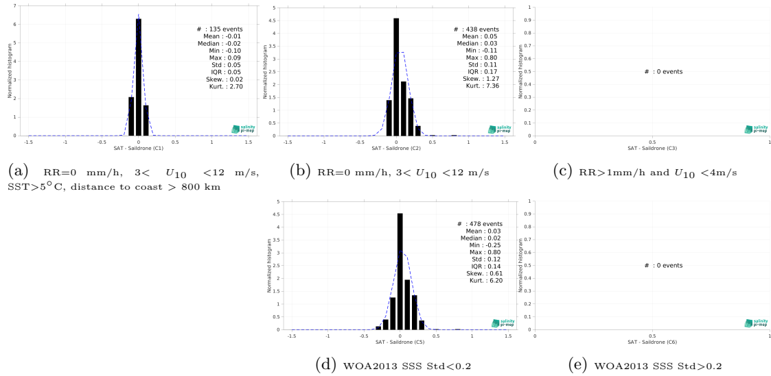
Figure 13: Normalized histogram of \Delta SSS (CCI SSS L4 Merged-OI v3.2 - 7-day running (ESA) - Saldrone) for 5 different subdatasets corresponding to: RR=0 mm/h, 3 < U_{10} < 12 m/s, SST > 5°C, distance to coast > 800 km (a), RR=0 mm/h, 3 < U_{10} < 12 m/s (b), RR > 1mm/h and U_{10} < 4 m/s (c), WOA2013 SSS Std < 0.2 (d), WOA2013 SSS Std > 0.2 (e).
