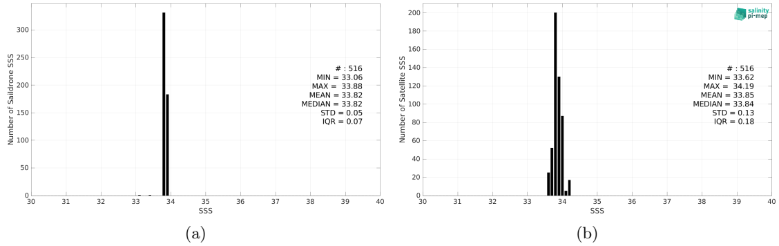
Figure 2: Histograms of SSS from Saildrone (a) and CCI SSS L4 Merged-OI v3.2 - 7-day running (ESA) (b) considering all match-up pairs per bins of 0.1 over the South Atlantic Ocean Pi-MEP region and for the full satellite product period.
