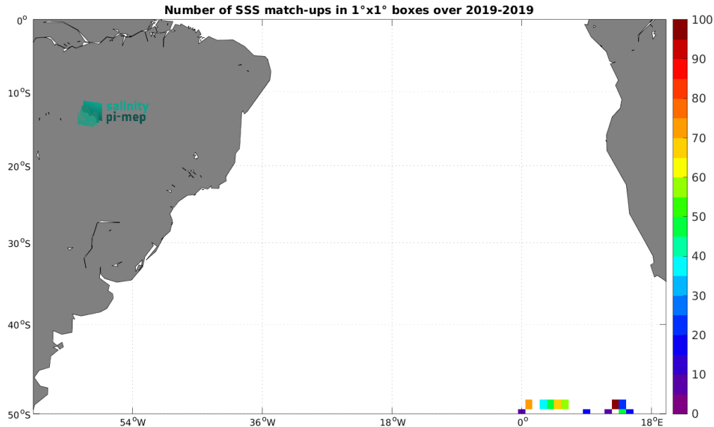
Figure 4: Number of SSS match-ups between Saildrone SSS and the CCI SSS L4 Merged-OI v3.2 - 7-day running (ESA) SSS product for the South Atlantic Ocean Pi-MEP region over 1^\circ \times 1^\circ boxes and for the full satellite product period.
