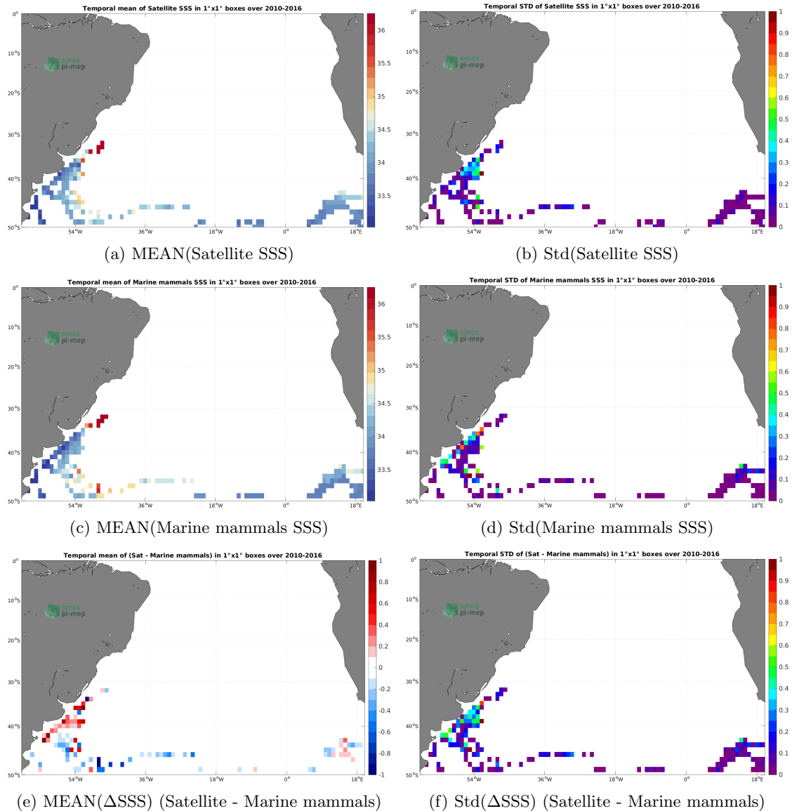
Figure 6: Temporal mean (left) and Std (right) of SSS from CCI SSS L4 Merged-OI v3.2 - 7-day running (ESA) (top), Marine mammals (middle), and of \Delta SSS (Satellite - Marine mammals). Only match-up pairs are used to generate these maps.
