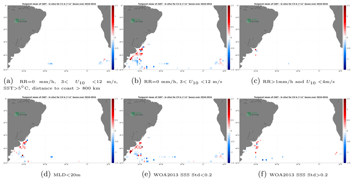
Figure 12: Temporal mean gridded over spatial boxes of size 1^\circ \times 1^\circ of \Delta SSS (CCI SSS L4 Merged-OI v3.2 - 7-day running (ESA) - Marine mammals) for 6 different subdatasets corresponding to:RR=0 mm/h, 3 < U_{10} < 12 m/s, SST >5^\circ C, distance to coast > 800 km (a), RR=0 mm/h, 3 < U_{10} < 12 m/s (b), RR >1 mm/h and U_{10} < 4 m/s (c),MLD <20 m (d),WOA2013 SSS Std <0.2 (e),WOA2013 SSS Std >0.2 (f).
