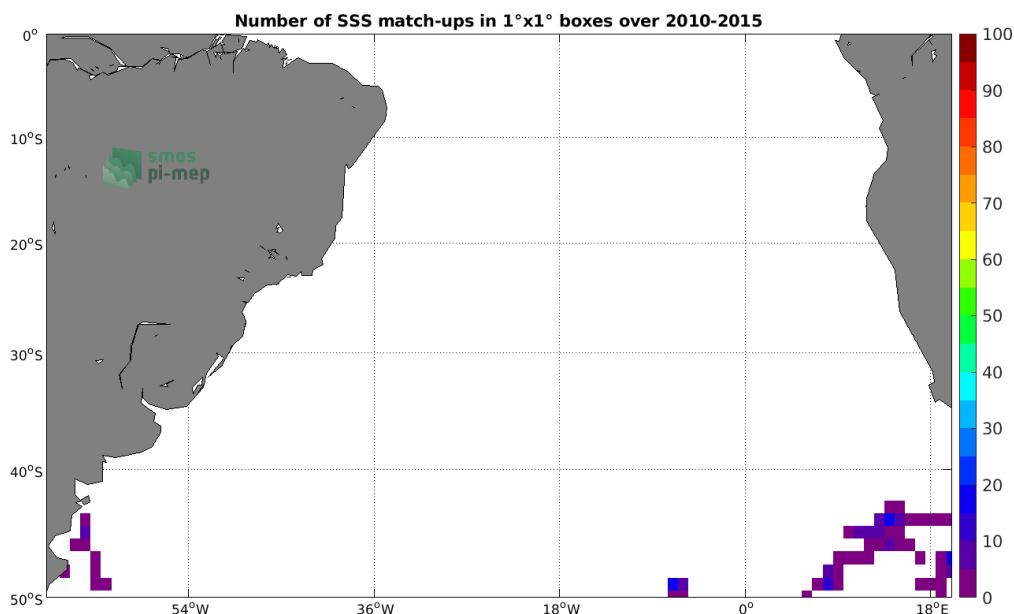
Figure 4: Number of SSS match-ups between Sea mammals SSS and the CCI SSS L4 Merged-OI v3.2 - 7-day running (ESA) SSS product for the South Atlantic Ocean Pi-MEP region over 1°x1° boxes and for the full satellite product period.
