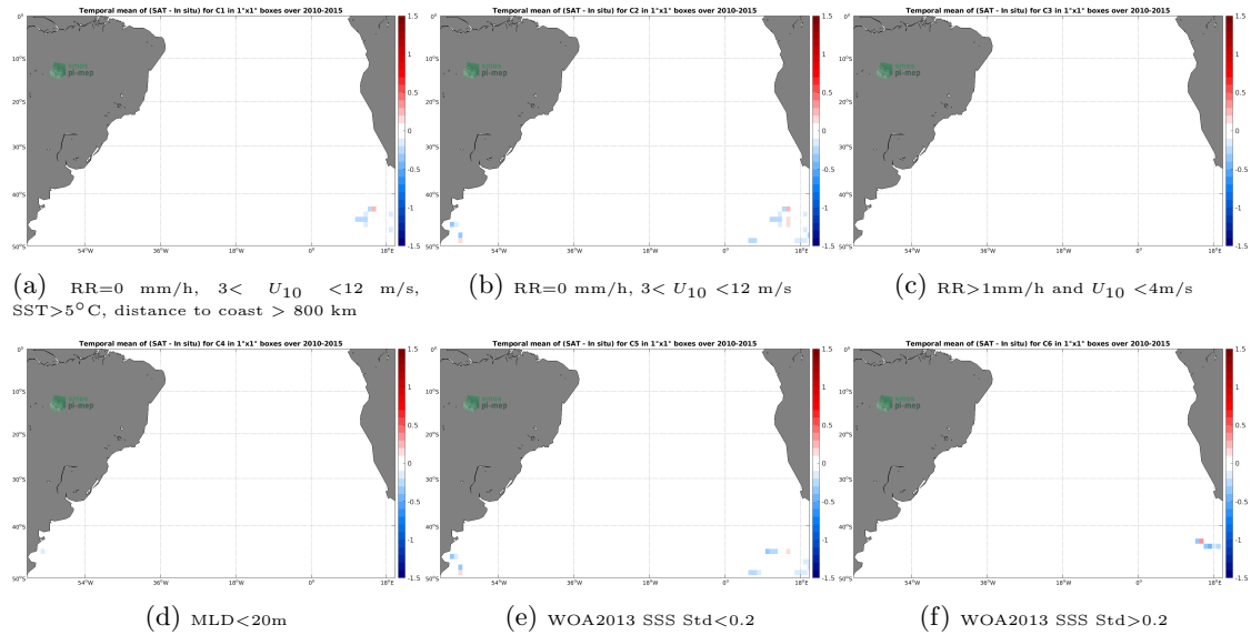
Figure 12: Temporal mean gridded over spatial boxes of size 1^{\circ}\times 1^{\circ} of \Delta\text{SSS} (CCI SSS L4 Merged-OI v3.2 - 7-day running (ESA) - Sea mammals) for 6 different subdatasets corresponding to:RR=0 mm/h, 3 < U_{10} < 12 m/s, SST >5^{\circ}\text{C} , distance to coast > 800 km (a), RR=0 mm/h, 3 < U_{10} < 12 m/s (b), RR >1 mm/h and U_{10} < 4 m/s (c),MLD <20 m (d),WOA2013 SSS Std <0.2 (e),WOA2013 SSS Std >0.2 (f).
