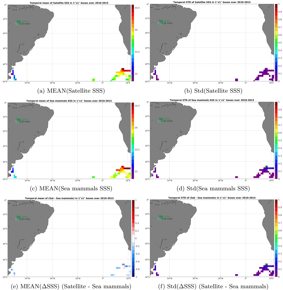
Figure 6: Temporal mean (left) and Std (right) of SSS from CCI SSS L4 Merged-OI v3.2 - 7-day running (ESA) (top), Sea mammals (middle), and of \Delta SSS (Satellite - Sea mammals). Only match-up pairs are used to generate these maps.
