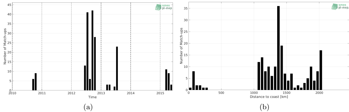
Figure 1: Number of match-ups between Sea mammals and CCI SSS L4 Merged-OI v3.2 - 7-day running (ESA) SSS as a function of time (a) and as function of the distance to coast (b) over the South Atlantic Ocean Pi-MEP region and for the full satellite product period.
