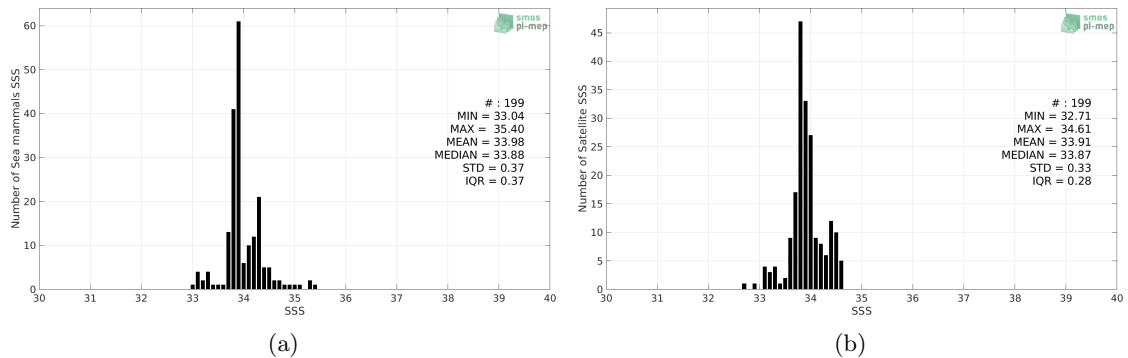
Figure 2: Histograms of SSS from Sea mammals (a) and CCI SSS L4 Merged-OI v3.2 - 7-day running (ESA) (b) considering all match-up pairs per bins of 0.1 over the South Atlantic Ocean Pi-MEP region and for the full satellite product period.
