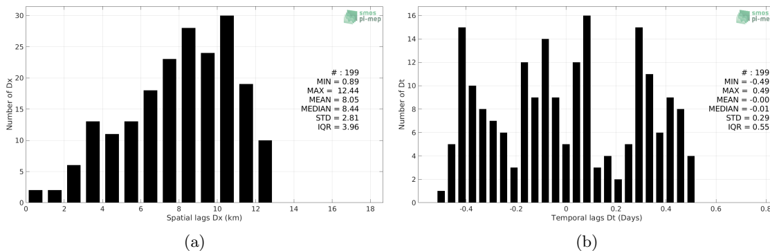
Figure 5: Histograms of the spatial (a) and temporal (b) lags between the location/time of the Sea mammals measurement and the date of the corresponding CCI SSS L4 Merged-OI v3.2 - 7-day running (ESA) SSS pixel.
