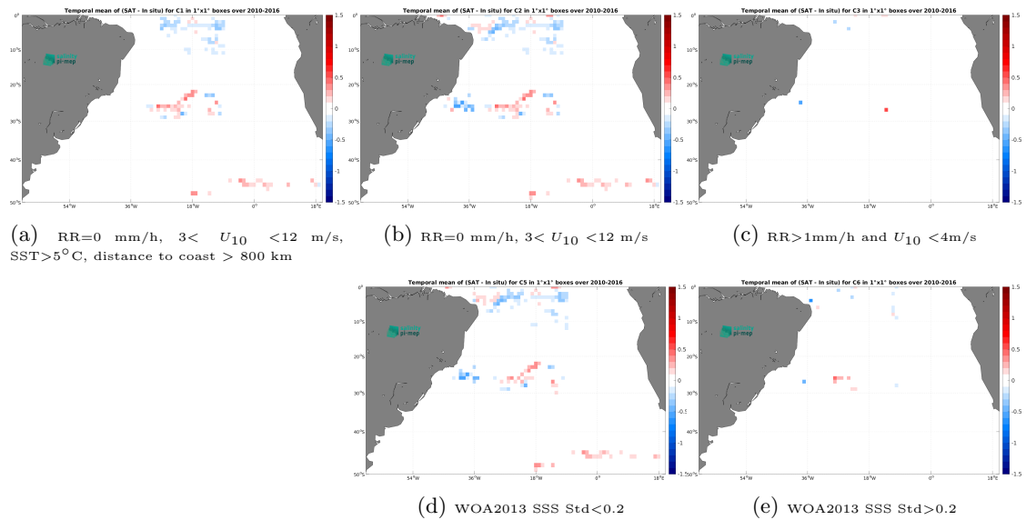
Figure 11: Temporal mean gridded over spatial boxes of size 1^\circ \times 1^\circ of \Delta SSS (CCI SSS L4 Merged-OI v3.2 - 7-day running (ESA) - Surface drifters) for 5 different subdatasets corresponding to:RR=0 mm/h, 3 < U_{10} < 12 m/s, SST >5^\circ C, distance to coast > 800 km (a), RR=0 mm/h, 3 < U_{10} < 12 m/s (b), RR >1 mm/h and U_{10} < 4 m/s (c), WOA2013 SSS Std <0.2 (d), WOA2013 SSS Std >0.2 (e).
