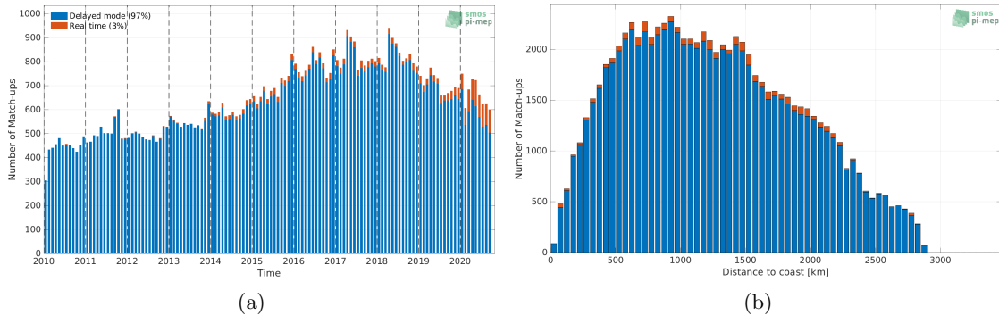
Figure 1: Number of match-ups between Argo and CCI SSS L4 Merged-OI v3.2 - 7-day running (ESA) SSS as a function of time (a) and as function of the distance to coast (b) over the South Atlantic Ocean Pi-MEP region and for the full satellite product period.
