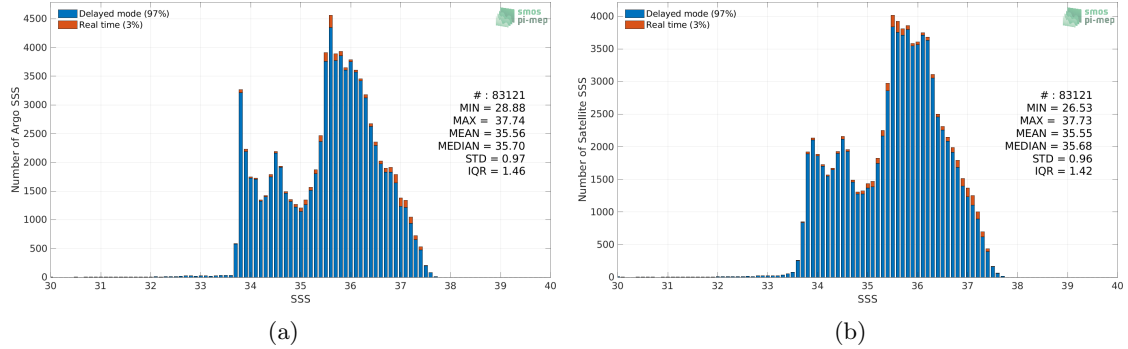
Figure 2: Histograms of SSS from Argo (a) and CCI SSS L4 Merged-OI v3.2 - 7-day running (ESA) (b) considering all match-up pairs per bins of 0.1 over the South Atlantic Ocean Pi-MEP region and for the full satellite product period.
