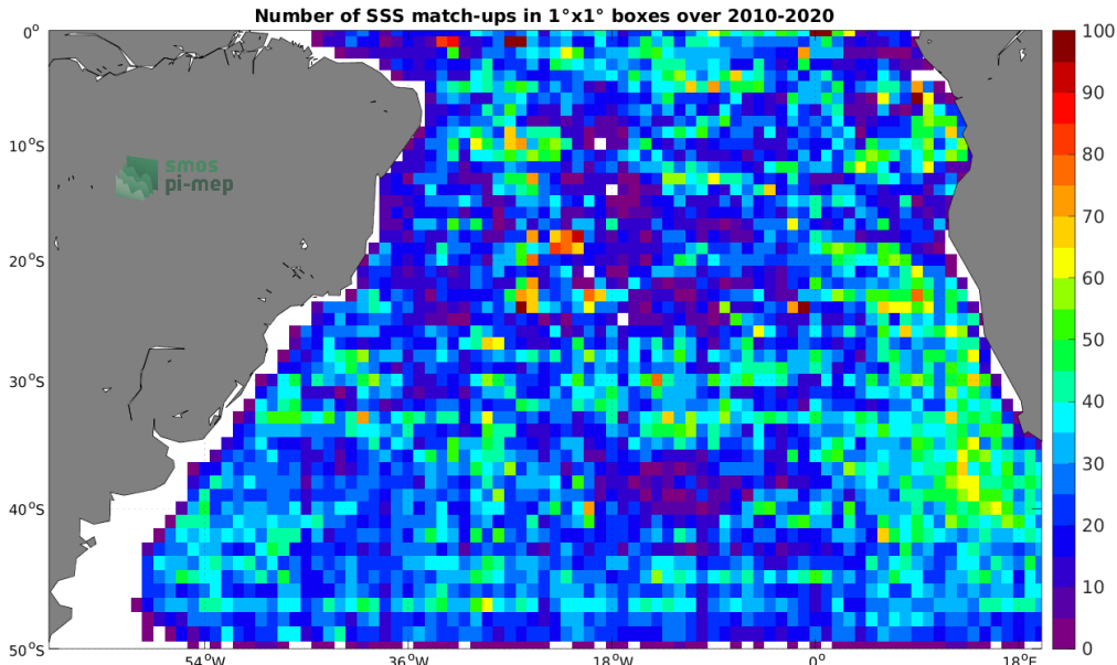
Figure 4: Number of SSS match-ups between Argo SSS and the CCI SSS L4 Merged-OI v3.2 - 7-day running (ESA) SSS product for the South Atlantic Ocean Pi-MEP region over 1^\circ \times 1^\circ boxes and for the full satellite product period.
