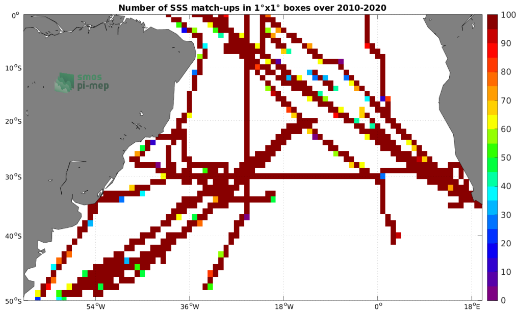
Figure 4: Number of SSS match-ups between TSG (SAMOS) SSS and the CCI SSS L4 Merged-OI v3.2 - 30-day running (ESA) SSS product for the South Atlantic Ocean Pi-MEP region over 1^\circ \times 1^\circ boxes and for the full satellite product period.
