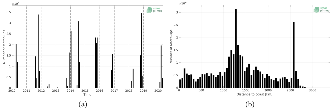
Figure 1: Number of match-ups between TSG (SAMOS) and CCI SSS L4 Merged-OI v3.2 - 30-day running (ESA) SSS as a function of time (a) and as function of the distance to coast (b) over the South Atlantic Ocean Pi-MEP region and for the full satellite product period.
