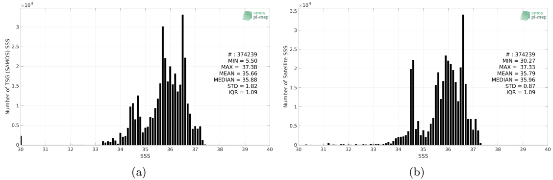
Figure 2: Histograms of SSS from TSG (SAMOS) (a) and CCI SSS L4 Merged-OI v3.2 - 30-day running (ESA) (b) considering all match-up pairs per bins of 0.1 over the South Atlantic Ocean Pi-MEP region and for the full satellite product period.
