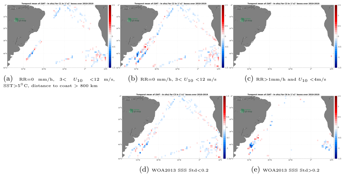
Figure 12: Temporal mean gridded over spatial boxes of size 1^\circ \times 1^\circ of \Delta\text{SSS} (CCI SSS L4 Merged-OI v3.2 - 30-day running (ESA) - TSG (Polarstern)) for 5 different subdatasets corresponding to:RR=0 mm/h, 3 < U_{10} < 12 m/s, SST >5^\circ\text{C} , distance to coast > 800 km (a), RR=0 mm/h, 3 < U_{10} < 12 m/s (b), RR >1 mm/h and U_{10} < 4 m/s (c), WOA2013 SSS Std <0.2 (d), WOA2013 SSS Std >0.2 (e).
