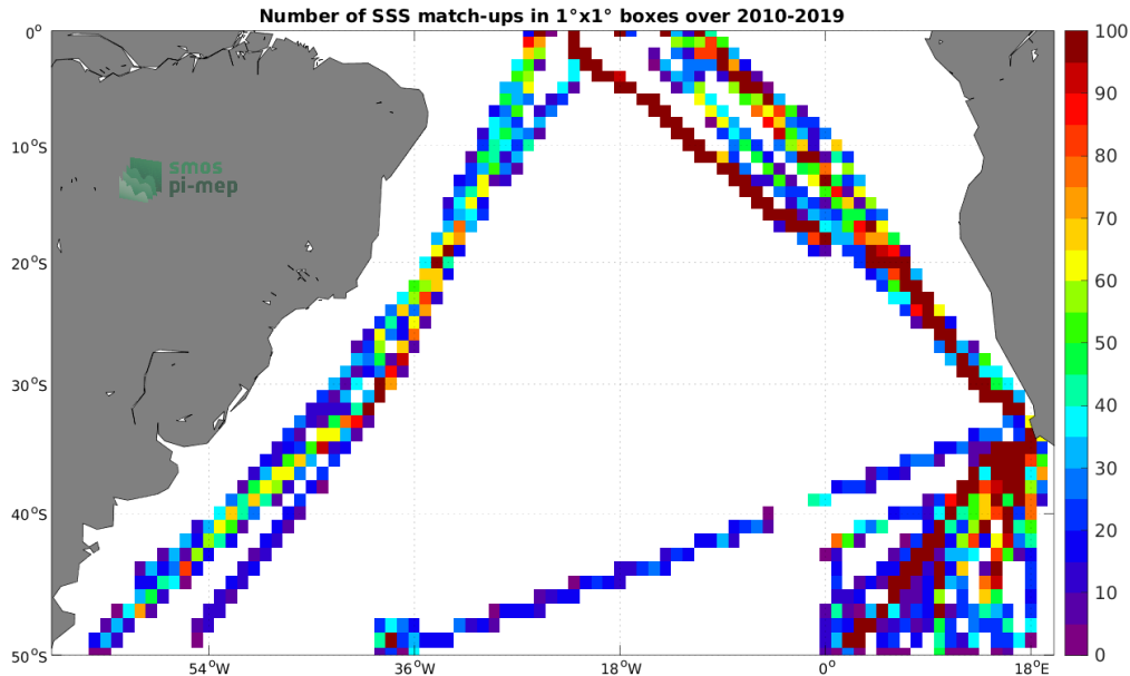
Figure 4: Number of SSS match-ups between TSG (Polarstern) SSS and the CCI SSS L4 Merged-OI v3.2 - 30-day running (ESA) SSS product for the South Atlantic Ocean Pi-MEP region over 1^\circ \times 1^\circ boxes and for the full satellite product period.
