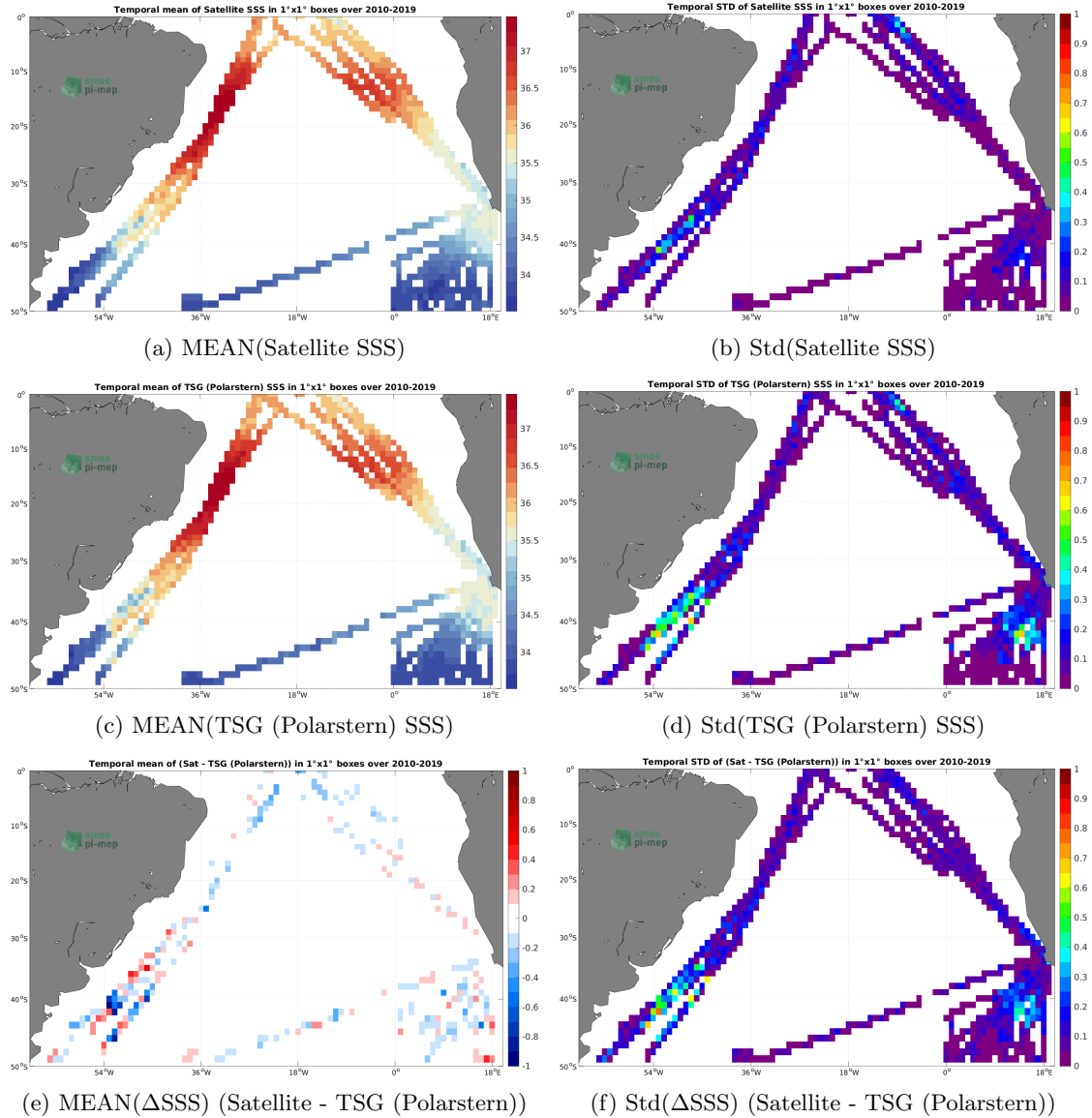
Figure 6: Temporal mean (left) and Std (right) of SSS from CCI SSS L4 Merged-OI v3.2 - 30-day running (ESA) (top), TSG (Polarstern) (middle), and of \Delta SSS (Satellite - TSG (Polarstern)). Only match-up pairs are used to generate these maps.
