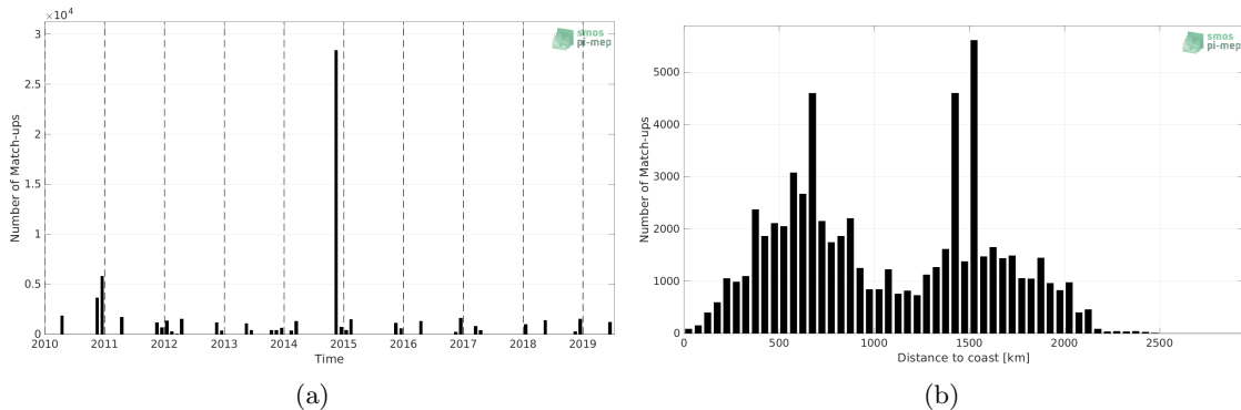
Figure 1: Number of match-ups between TSG (Polarstern) and CCI SSS L4 Merged-OI v3.2 - 30-day running (ESA) SSS as a function of time (a) and as function of the distance to coast (b) over the South Atlantic Ocean Pi-MEP region and for the full satellite product period.
