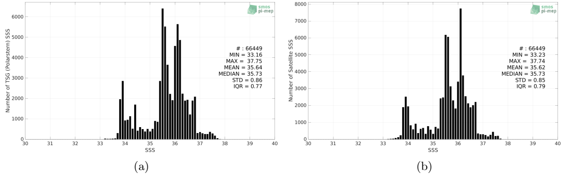
Figure 2: Histograms of SSS from TSG (Polarstern) (a) and CCI SSS L4 Merged-OI v3.2 - 30-day running (ESA) (b) considering all match-up pairs per bins of 0.1 over the South Atlantic Ocean Pi-MEP region and for the full satellite product period.
