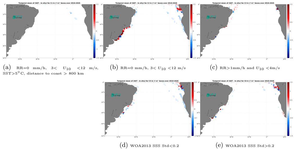
Figure 12: Temporal mean gridded over spatial boxes of size 1^\circ \times 1^\circ of \Delta\text{SSS} (CCI SSS L4 Merged-OI v3.2 - 30-day running (ESA) - TSG (LEGOS-DM)) for 5 different subdatasets corresponding to:RR=0 mm/h, 3 < U_{10} < 12 m/s, SST >5^\circ\text{C} , distance to coast > 800 km (a), RR=0 mm/h, 3 < U_{10} < 12 m/s (b), RR >1 mm/h and U_{10} < 4 m/s (c), WOA2013 SSS Std <0.2 (d), WOA2013 SSS Std >0.2 (e).
