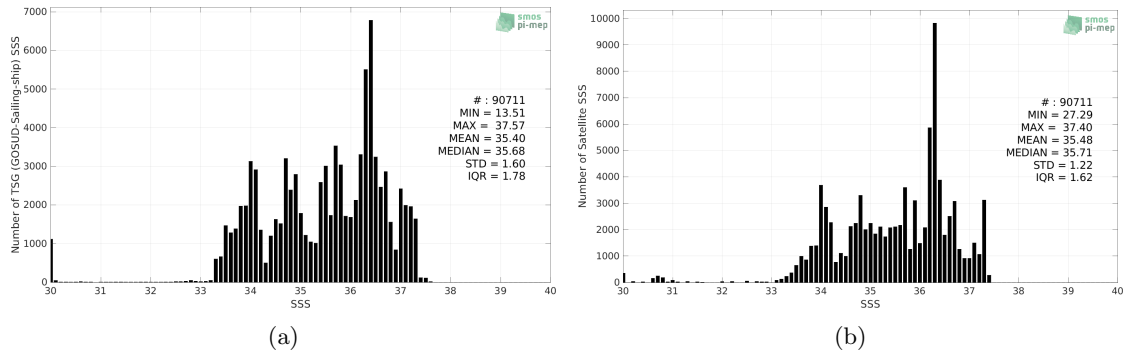
Figure 2: Histograms of SSS from TSG (GOSUD-Sailing-ship) (a) and CCI SSS L4 Merged-OI v3.2 - 30-day running (ESA) (b) considering all match-up pairs per bins of 0.1 over the South Atlantic Ocean Pi-MEP region and for the full satellite product period.
