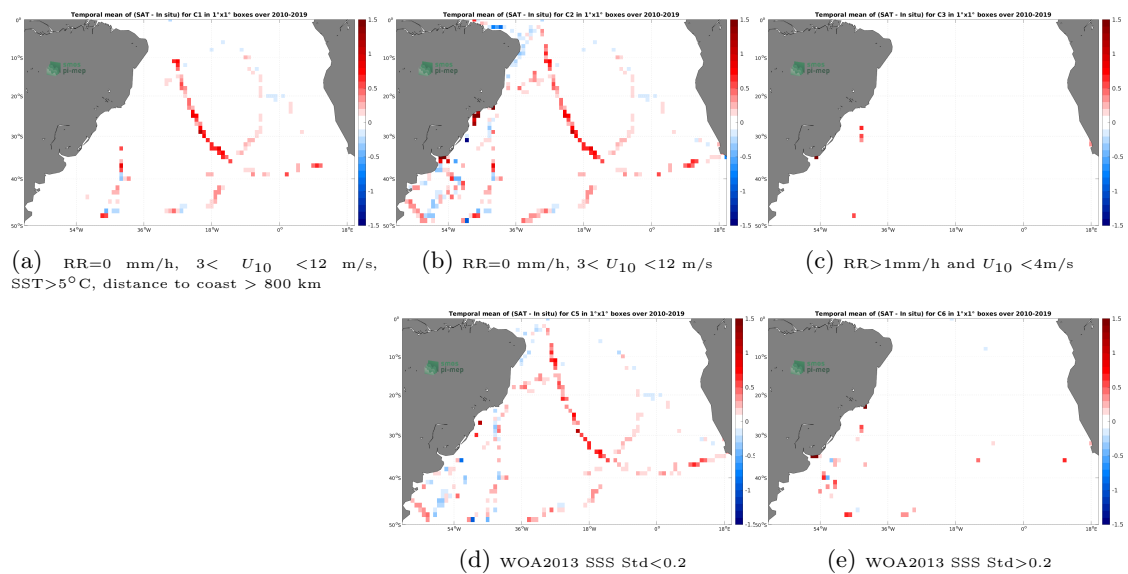
Figure 12: Temporal mean gridded over spatial boxes of size 1^\circ \times 1^\circ of \Delta\text{SSS} (CCI SSS L4 Merged-OI v3.2 - 30-day running (ESA) - TSG (GOSUD-Sailing-ship)) for 5 different subdatasets corresponding to:RR=0 mm/h, 3 < U_{10} < 12 m/s, SST >5^\circ\text{C} , distance to coast > 800 km (a), RR=0 mm/h, 3 < U_{10} < 12 m/s (b), RR >1 mm/h and U_{10} < 4 m/s (c), WOA2013 SSS Std <0.2 (d), WOA2013 SSS Std >0.2 (e).
