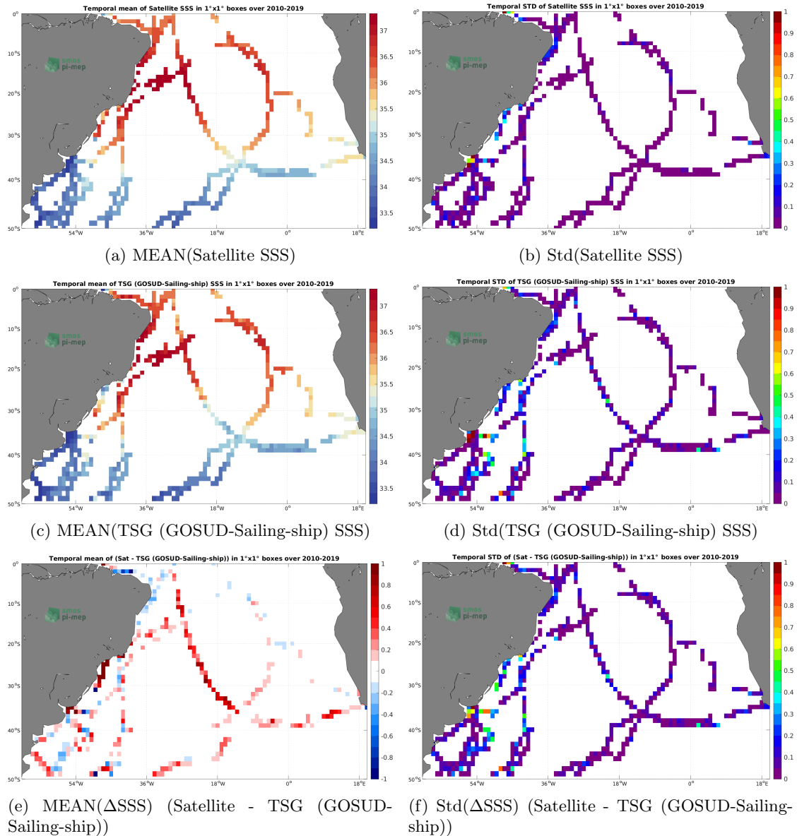
Figure 6: Temporal mean (left) and Std (right) of SSS from CCI SSS L4 Merged-OI v3.2 - 30-day running (ESA) (top), TSG (GOSUD-Sailing-ship) (middle), and of \Delta SSS (Satellite - TSG (GOSUD-Sailing-ship)). Only match-up pairs are used to generate these maps.
