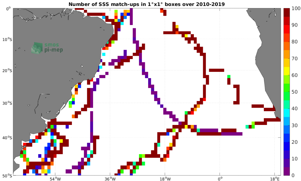
Figure 4: Number of SSS match-ups between TSG (GOSUD-Sailing-ship) SSS and the CCI SSS L4 Merged-OI v3.2 - 30-day running (ESA) SSS product for the South Atlantic Ocean Pi-MEP region over 1^\circ \times 1^\circ boxes and for the full satellite product period.
