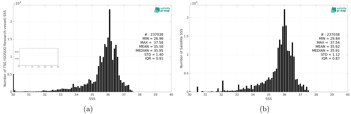
Figure 2: Histograms of SSS from TSG (GOSUD-Research-vessel) (a) and CCI SSS L4 Merged-OI v3.2 - 30-day running (ESA) (b) considering all match-up pairs per bins of 0.1 over the South Atlantic Ocean Pi-MEP region and for the full satellite product period.
