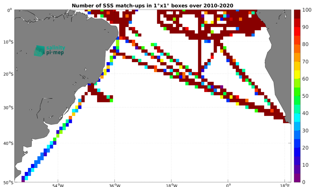
Figure 4: Number of SSS match-ups between TSG (GOSUD-Research-vessel) SSS and the CCI SSS L4 Merged-OI v3.2 - 30-day running (ESA) SSS product for the South Atlantic Ocean Pi-MEP region over 1^\circ \times 1^\circ boxes and for the full satellite product period.
