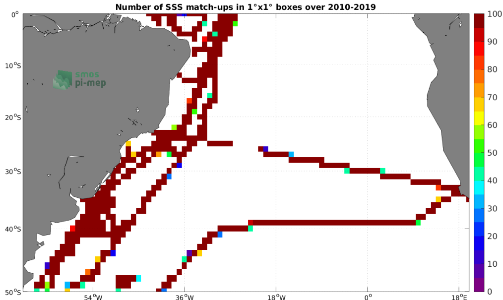
Figure 4: Number of SSS match-ups between TSG (CSIC-UTM) SSS and the CCI SSS L4 Merged-OI v3.2 - 30-day running (ESA) SSS product for the South Atlantic Ocean Pi-MEP region over 1^{\circ} \times 1^{\circ} boxes and for the full satellite product period.
