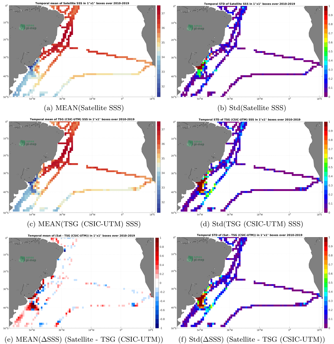
Figure 6: Temporal mean (left) and Std (right) of SSS from CCI SSS L4 Merged-OI v3.2 - 30-day running (ESA) (top), TSG (CSIC-UTM) ( in situ ) dataset (middle), and of \Delta SSS (Satellite - TSG (CSIC-UTM)). Only match-up pairs are used to generate these maps.
