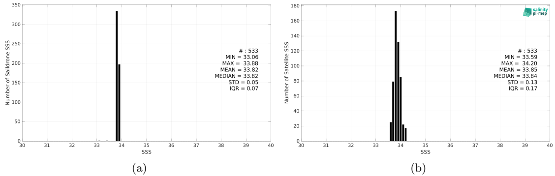
Figure 2: Histograms of SSS from Saildrone (a) and CCI SSS L4 Merged-OI v3.2 - 30-day running (ESA) (b) considering all match-up pairs per bins of 0.1 over the South Atlantic Ocean Pi-MEP region and for the full satellite product period.
