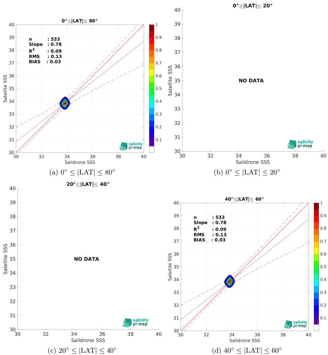
Figure 9: Contour maps of the concentration of CCI SSS L4 Merged-OI v3.2 - 30-day running (ESA) SSS (y-axis) versus Saildrone SSS (x-axis) at match-up pairs for different latitude bands. For each plot, the red line shows x=y . The black thin and dashed lines indicate a linear fit through the data cloud and the \pm 95\% confidence levels, respectively. The number match-up pairs n , the slope and R^2 coefficient of the linear fit, the root mean square (RMS) and the mean bias between satellite and in situ data are indicated for each latitude band in each plots.
