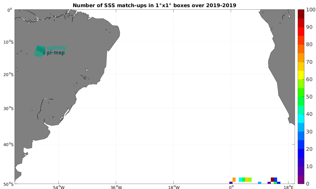
Figure 4: Number of SSS match-ups between Saildrone SSS and the CCI SSS L4 Merged-OI v3.2 - 30-day running (ESA) SSS product for the South Atlantic Ocean Pi-MEP region over 1^\circ \times 1^\circ boxes and for the full satellite product period.
