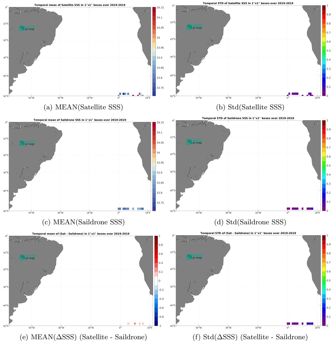
Figure 6: Temporal mean (left) and Std (right) of SSS from CCI SSS L4 Merged-OI v3.2 - 30-day running (ESA) (top), Saildrone (middle), and of \Delta SSS (Satellite - Saildrone). Only match-up pairs are used to generate these maps.
