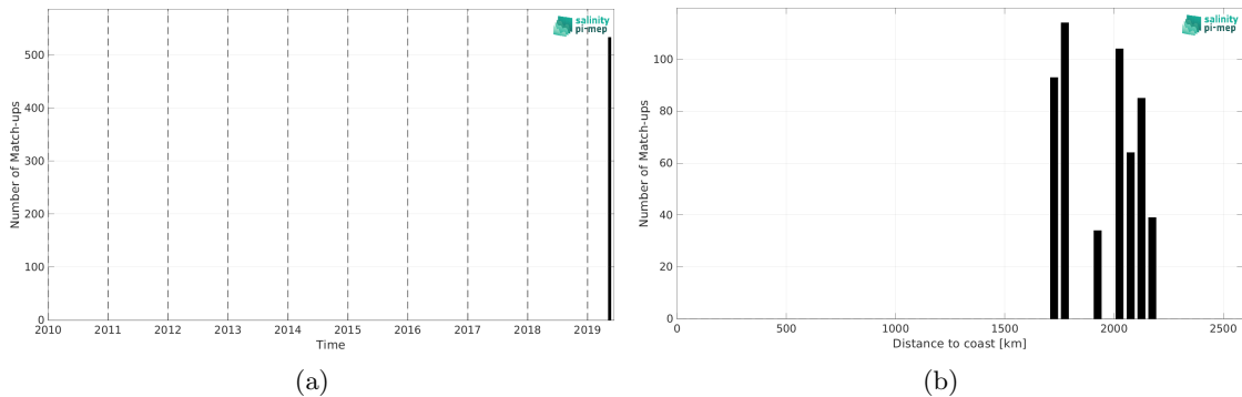
Figure 1: Number of match-ups between Saildrone and CCI SSS L4 Merged-OI v3.2 - 30-day running (ESA) SSS as a function of time (a) and as function of the distance to coast (b) over the South Atlantic Ocean Pi-MEP region and for the full satellite product period.
