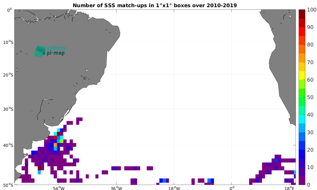
Figure 4: Number of SSS match-ups between Marine mammals SSS and the CCI SSS L4 Merged-OI v3.2 - 30-day running (ESA) SSS product for the South Atlantic Ocean Pi-MEP region over 1^\circ \times 1^\circ boxes and for the full satellite product period.
