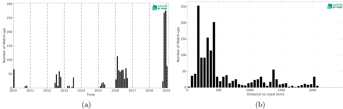
Figure 1: Number of match-ups between Marine mammals and CCI SSS L4 Merged-OI v3.2 - 30-day running (ESA) SSS as a function of time (a) and as function of the distance to the coast (b) over the South Atlantic Ocean Pi-MEP region and for the full satellite product period.
