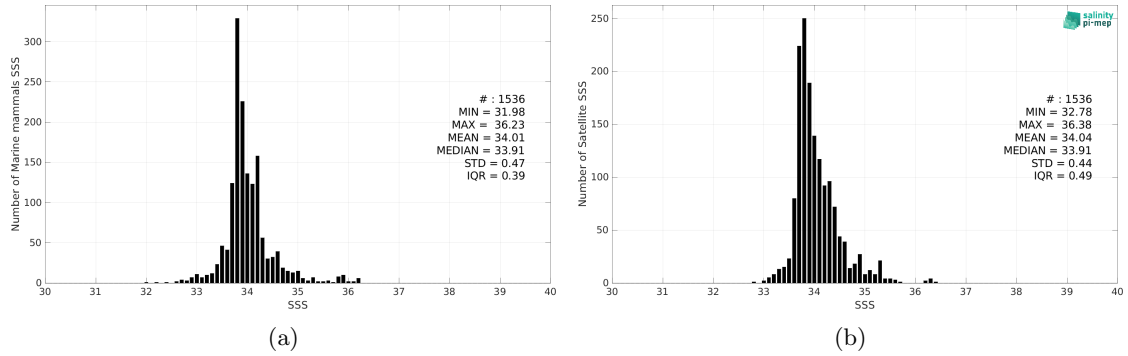
Figure 2: Histograms of SSS from Marine mammals (a) and CCI SSS L4 Merged-OI v3.2 - 30-day running (ESA) (b) considering all match-up pairs per bins of 0.1 over the South Atlantic Ocean Pi-MEP region and for the full satellite product period.
