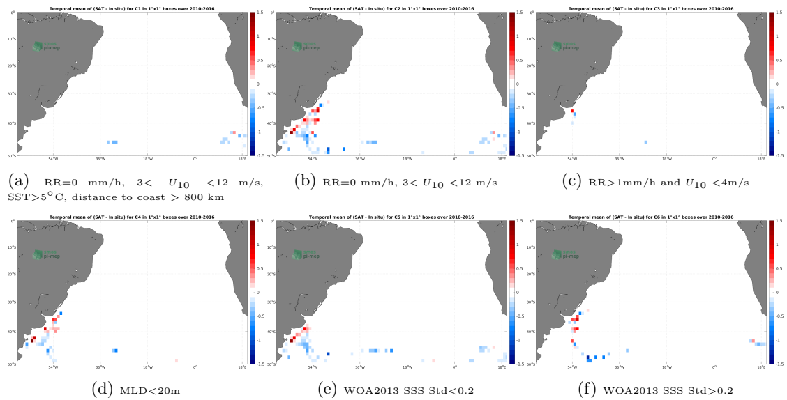
Figure 12: Temporal mean gridded over spatial boxes of size 1^\circ \times 1^\circ of \Delta SSS (CCI SSS L4 Merged-OI v3.2 - 30-day running (ESA) - Marine mammals) for 6 different subdatasets corresponding to:RR=0 mm/h, 3 < U_{10} < 12 m/s, SST > 5^\circ\text{C} , distance to coast > 800 km (a), RR=0 mm/h, 3 < U_{10} < 12 m/s (b), RR > 1 mm/h and U_{10} < 4 m/s (c),MLD < 20 m (d),WOA2013 SSS Std < 0.2 (e),WOA2013 SSS Std > 0.2 (f).
