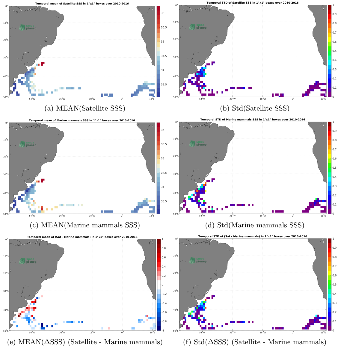
Figure 6: Temporal mean (left) and Std (right) of SSS from CCI SSS L4 Merged-OI v3.2 - 30-day running (ESA) (top), Marine mammals (middle), and of \Delta SSS (Satellite - Marine mammals). Only match-up pairs are used to generate these maps.
