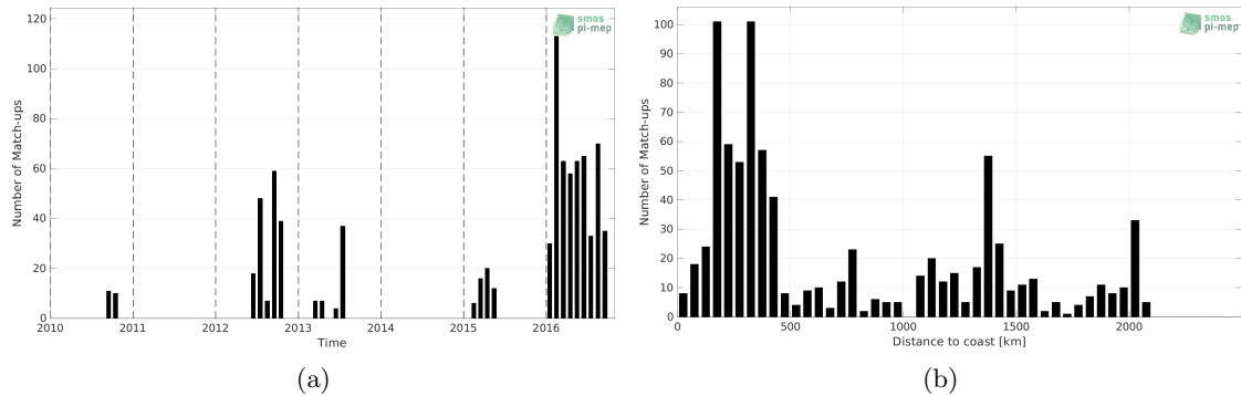
Figure 1: Number of match-ups between Marine mammals and CCI SSS L4 Merged-OI v3.2 - 30-day running (ESA) SSS as a function of time (a) and as function of the distance to coast (b) over the South Atlantic Ocean Pi-MEP region and for the full satellite product period.
