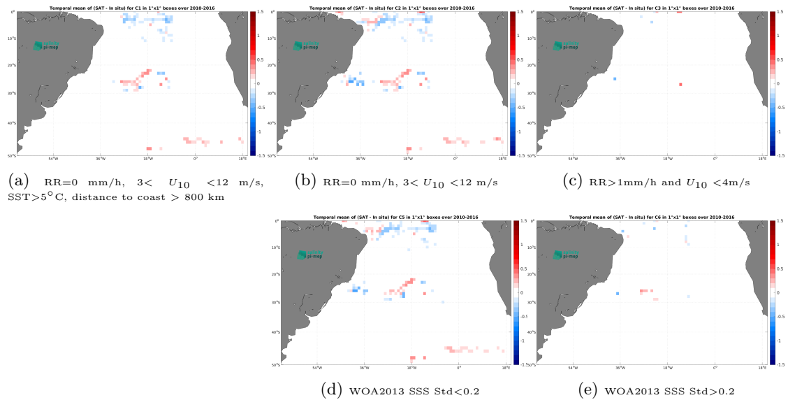
Figure 11: Temporal mean gridded over spatial boxes of size 1^\circ \times 1^\circ of \Delta SSS (CCI SSS L4 Merged-OI v3.2 - 30-day running (ESA) - Surface drifters) for 5 different subdatasets corresponding to:RR=0 mm/h, 3 < U_{10} < 12 m/s, SST >5^\circ C, distance to coast > 800 km (a), RR=0 mm/h, 3 < U_{10} < 12 m/s (b), RR >1 mm/h and U_{10} < 4 m/s (c), WOA2013 SSS Std <0.2 (d), WOA2013 SSS Std >0.2 (e).
