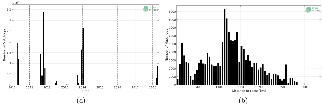
Figure 1: Number of match-ups between TSG (SAMOS) and CCI SSS L4 Merged-OI v2.31 - 30-day running (ESA) SSS as a function of time (a) and as function of the distance to coast (b) over the South Atlantic Ocean Pi-MEP region and for the full satellite product period.
