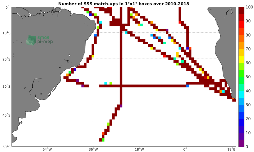
Figure 4: Number of SSS match-ups between TSG (SAMOS) SSS and the CCI SSS L4 Merged-OI v2.31 - 30-day running (ESA) SSS product for the South Atlantic Ocean Pi-MEP region over 1°x1° boxes and for the full satellite product period.
