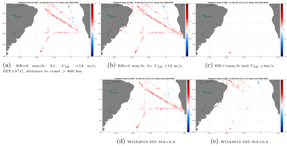
Figure 12: Temporal mean gridded over spatial boxes of size 1^\circ \times 1^\circ of \Delta SSS (CCI L4 Merged-OI v2.31 - 30-day running (ESA) - TSG (SAMOS)) for 5 different subdatasets corresponding to: RR=0 mm/h, 3 < U_{10} < 12 m/s, SST >5^\circ\text{C} , distance to coast > 800 km (a), RR=0 mm/h, 3 < U_{10} < 12 m/s (b), RR >1 mm/h and U_{10} < 4 m/s (c), WOA2013 SSS Std <0.2 (d), WOA2013 SSS Std >0.2 (e).
