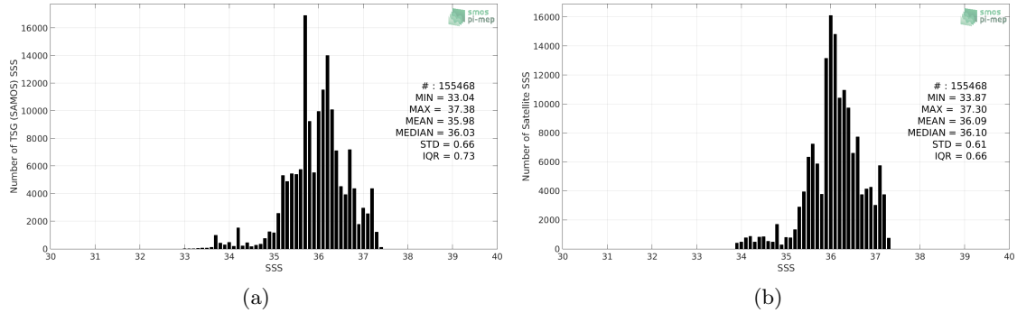
Figure 2: Histograms of SSS from TSG (SAMOS) (a) and CCI L4 Merged-OI v2.31 - 30-day running (ESA) (b) considering all match-up pairs per bins of 0.1 over the South Atlantic Ocean Pi-MEP region and for the full satellite product period.
