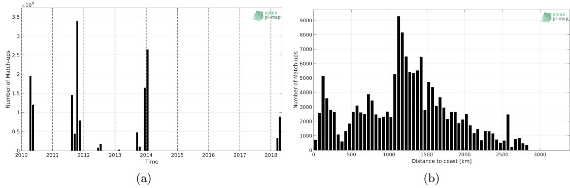
Figure 1: Number of match-ups between TSG (SAMOS) and CCI L4 Merged-OI v2.31 - 30-day running (ESA) SSS as a function of time (a) and as function of the distance to coast (b) over the South Atlantic Ocean Pi-MEP region and for the full satellite product period.
