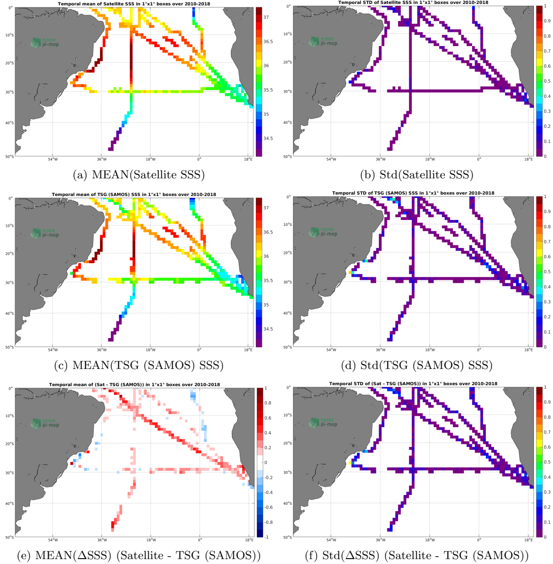
Figure 6: Temporal mean (left) and Std (right) of SSS from CCI L4 Merged-OI v2.31 - 30-day running (ESA) (top), TSG (SAMOS) (middle), and of \Delta SSS (Satellite - TSG (SAMOS)). Only match-up pairs are used to generate these maps.
