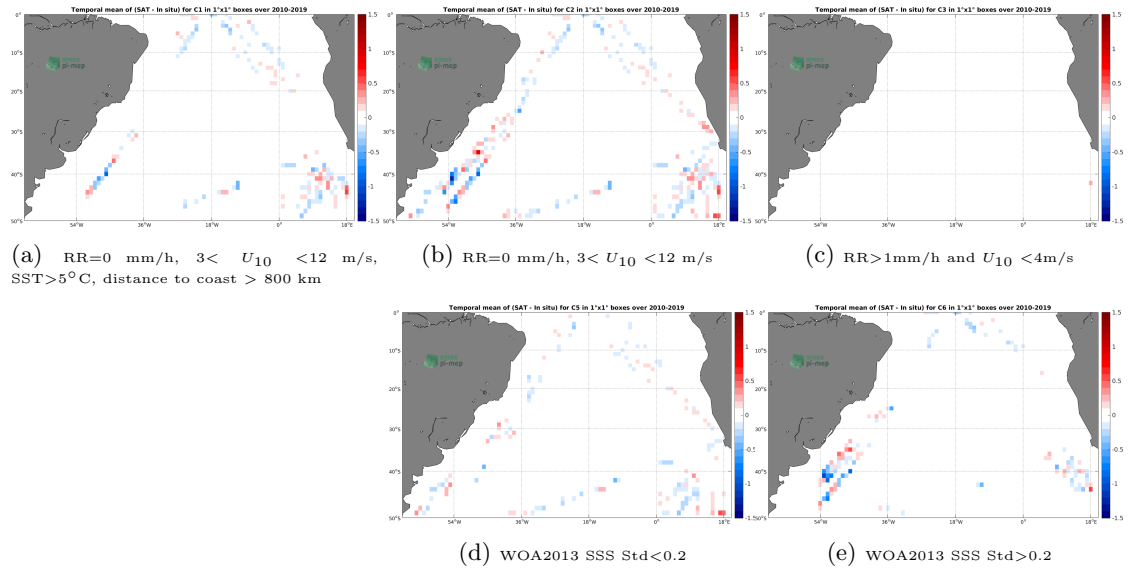
Figure 12: Temporal mean gridded over spatial boxes of size 1^\circ \times 1^\circ of \Delta SSS (CCI SSS L4 Merged-OI v2.31 - 30-day running (ESA) - TSG (Polarstern)) for 5 different subdatasets corresponding to:RR=0 mm/h, 3 < U_{10} < 12 m/s, SST >5^\circ\text{C} , distance to coast > 800 km (a), RR=0 mm/h, 3 < U_{10} < 12 m/s (b), RR >1 mm/h and U_{10} < 4 m/s (c), WOA2013 SSS Std <0.2 (d), WOA2013 SSS Std >0.2 (e).
