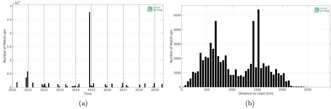
Figure 1: Number of match-ups between TSG (Polarstern) and CCI SSS L4 Merged-OI v2.31 - 30-day running (ESA) SSS as a function of time (a) and as function of the distance to coast (b) over the South Atlantic Ocean Pi-MEP region and for the full satellite product period.
