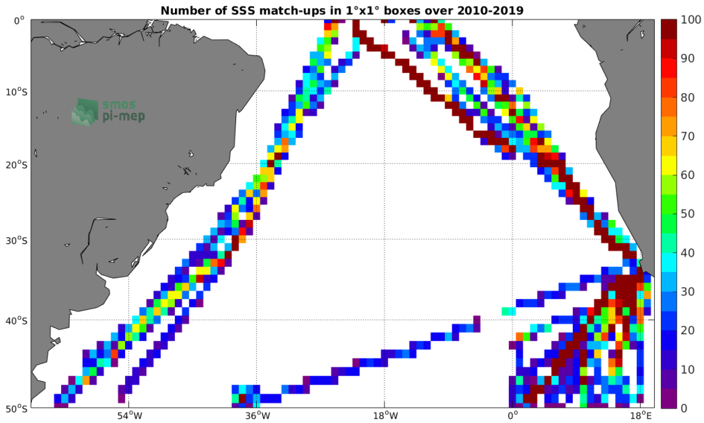
Figure 4: Number of SSS match-ups between TSG (Polarstern) SSS and the CCI SSS L4 Merged-OI v2.31 - 30-day running (ESA) SSS product for the South Atlantic Ocean Pi-MEP region over 1^\circ \times 1^\circ boxes and for the full satellite product period.
