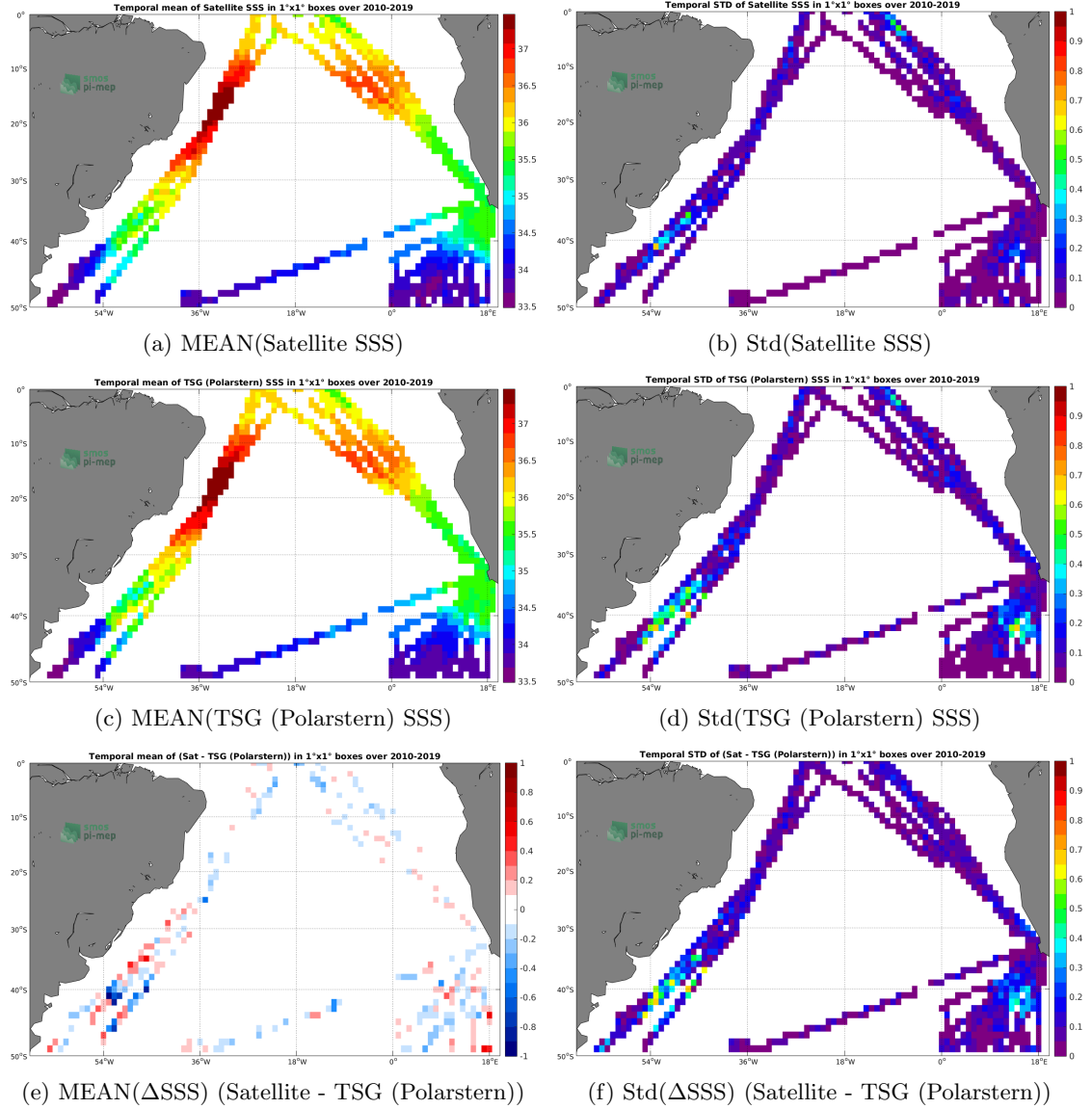
Figure 6: Temporal mean (left) and Std (right) of SSS from CCI SSS L4 Merged-OI v2.31 - 30-day running (ESA) (top), TSG (Polarstern) (middle), and of \Delta SSS (Satellite - TSG (Polarstern)). Only match-up pairs are used to generate these maps.
