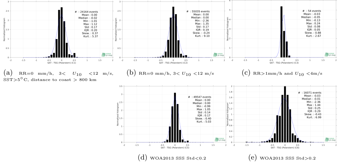
Figure 13: Normalized histogram of \Delta\text{SSS} (CCI SSS L4 Merged-OI v2.31 - 30-day running (ESA) - TSG (Polarstern)) for 5 different subdatasets corresponding to: RR=0 mm/h, 3 < U_{10} < 12 m/s, SST>5°C, distance to coast > 800 km (a), RR=0 mm/h, 3 < U_{10} < 12 m/s (b), RR>1mm/h and U_{10} < 4 m/s (c), WOA2013 SSS Std<0.2 (d), WOA2013 SSS Std>0.2 (e).
