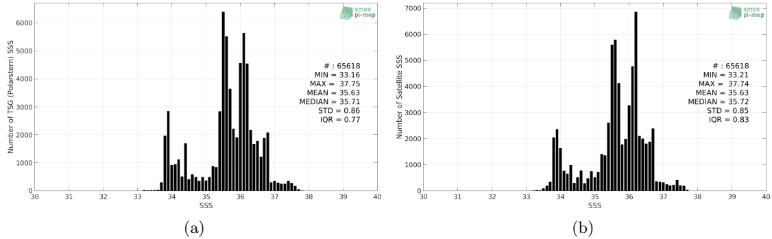
Figure 2: Histograms of SSS from TSG (Polarstern) (a) and CCI SSS L4 Merged-OI v2.31 - 30-day running (ESA) (b) considering all match-up pairs per bins of 0.1 over the South Atlantic Ocean Pi-MEP region and for the full satellite product period.
