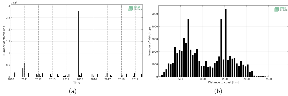
Figure 1: Number of match-ups between TSG (Polarstern) and CCI L4 Merged-OI v2.31 - 30-day running (ESA) SSS as a function of time (a) and as function of the distance to coast (b) over the South Atlantic Ocean Pi-MEP region and for the full satellite product period.
