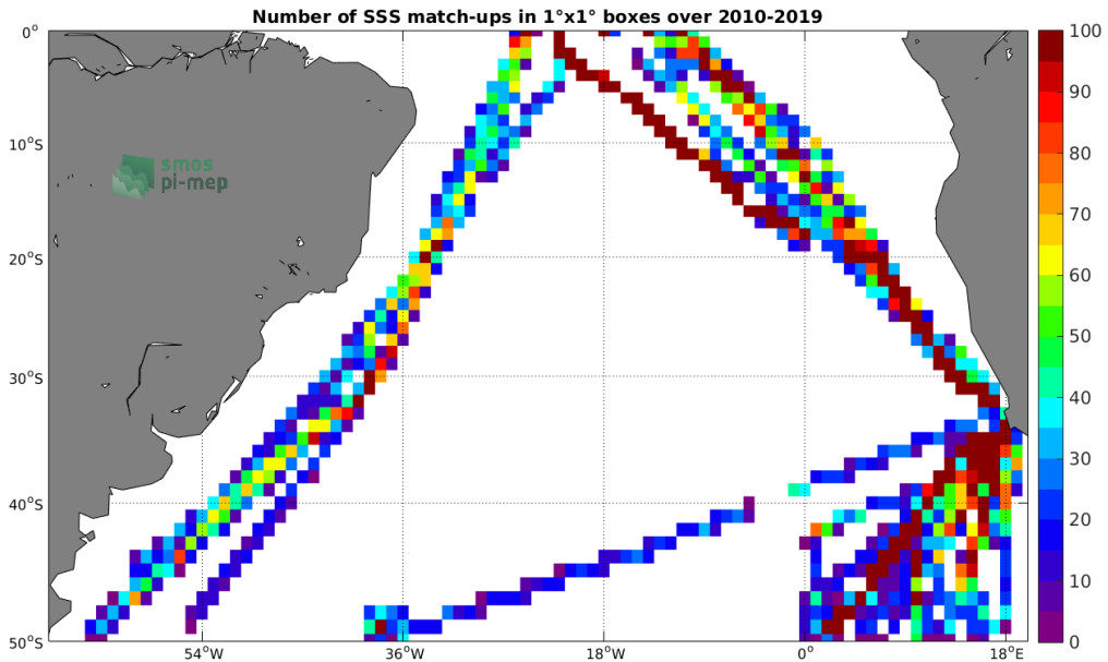
Figure 4: Number of SSS match-ups between TSG (Polarstern) SSS and the CCI L4 Merged-OI v2.31 - 30-day running (ESA) SSS product for the South Atlantic Ocean Pi-MEP region over 1°x1° boxes and for the full satellite product period.
