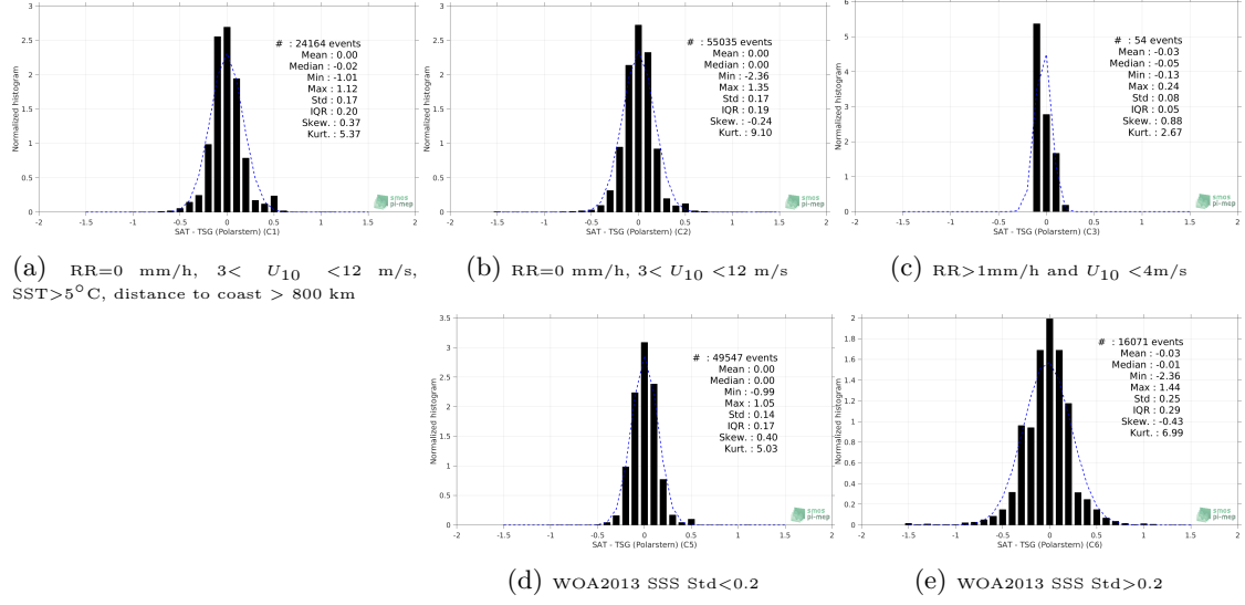
Figure 13: Normalized histogram of \Delta\text{SSS} (CCI L4 Merged-OI v2.31 - 30-day running (ESA) - TSG (Polarstern)) for 5 different subdatasets corresponding to: RR=0 mm/h, 3 < U_{10} < 12 m/s, SST > 5^{\circ}\text{C} , distance to coast > 800 km (a), RR=0 mm/h, 3 < U_{10} < 12 m/s (b), RR > 1\text{mm/h} and U_{10} < 4\text{m/s} (c), WOA2013 SSS Std < 0.2 (d), WOA2013 SSS Std > 0.2 (e).
