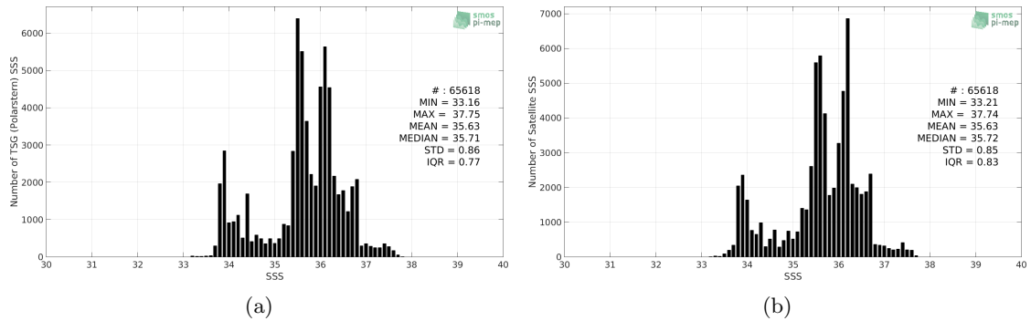
Figure 2: Histograms of SSS from TSG (Polarstern) (a) and CCI L4 Merged-OI v2.31 - 30-day running (ESA) (b) considering all match-up pairs per bins of 0.1 over the South Atlantic Ocean Pi-MEP region and for the full satellite product period.
