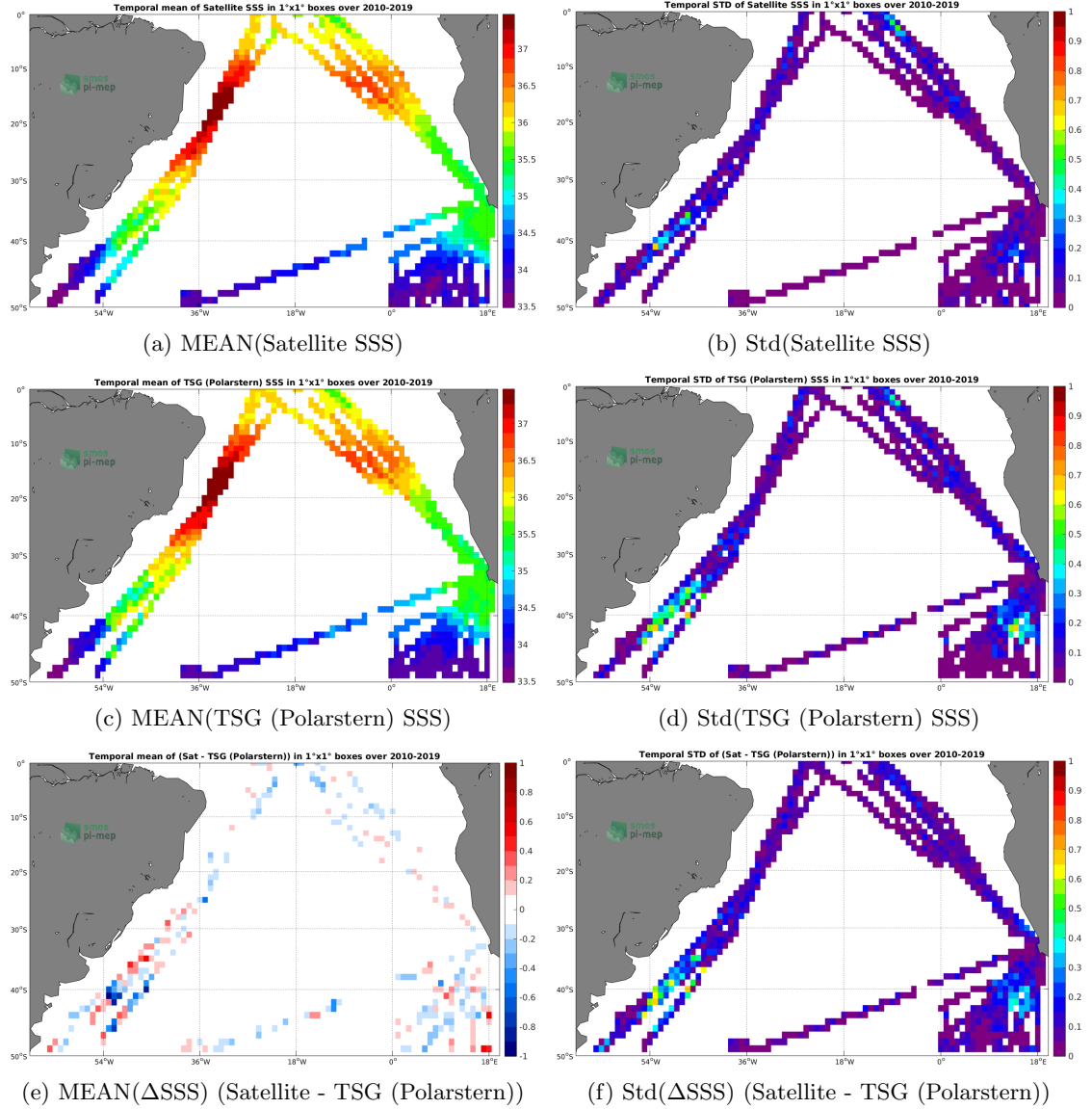
Figure 6: Temporal mean (left) and Std (right) of SSS from CCI L4 Merged-OI v2.31 - 30-day running (ESA) (top), TSG (Polarstern) (middle), and of \Delta SSS (Satellite - TSG (Polarstern)). Only match-up pairs are used to generate these maps.
