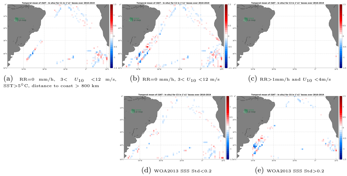
Figure 12: Temporal mean gridded over spatial boxes of size 1^\circ \times 1^\circ of \Delta SSS (CCI L4 Merged-OI v2.31 - 30-day running (ESA) - TSG (Polarstern)) for 5 different subdatasets corresponding to: RR=0 mm/h, 3 < U_{10} < 12 m/s, SST > 5^\circ\text{C} , distance to coast > 800 km (a), RR=0 mm/h, 3 < U_{10} < 12 m/s (b), RR > 1 mm/h and U_{10} < 4 m/s (c), WOA2013 SSS Std < 0.2 (d), WOA2013 SSS Std > 0.2 (e).
