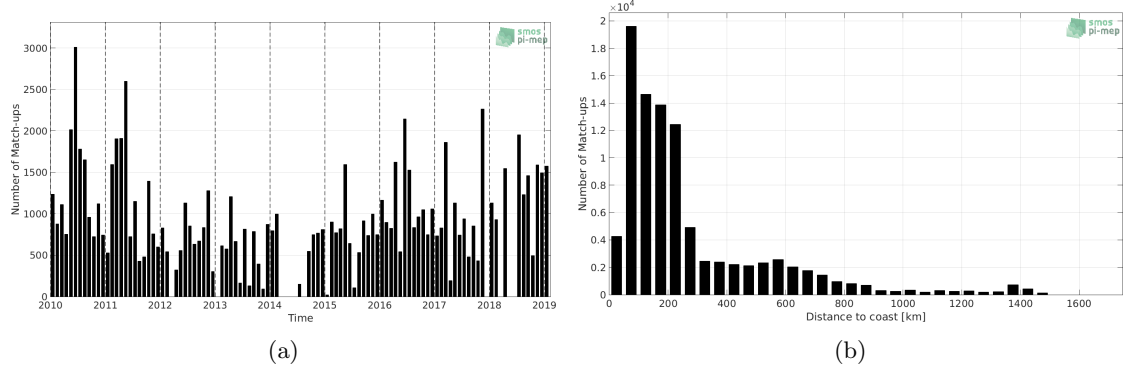
Figure 1: Number of match-ups between TSG (LEGOS-DM) and CCI SSS L4 Merged-OI v2.31 - 30-day running (ESA) SSS as a function of time (a) and as function of the distance to coast (b) over the South Atlantic Ocean Pi-MEP region and for the full satellite product period.
