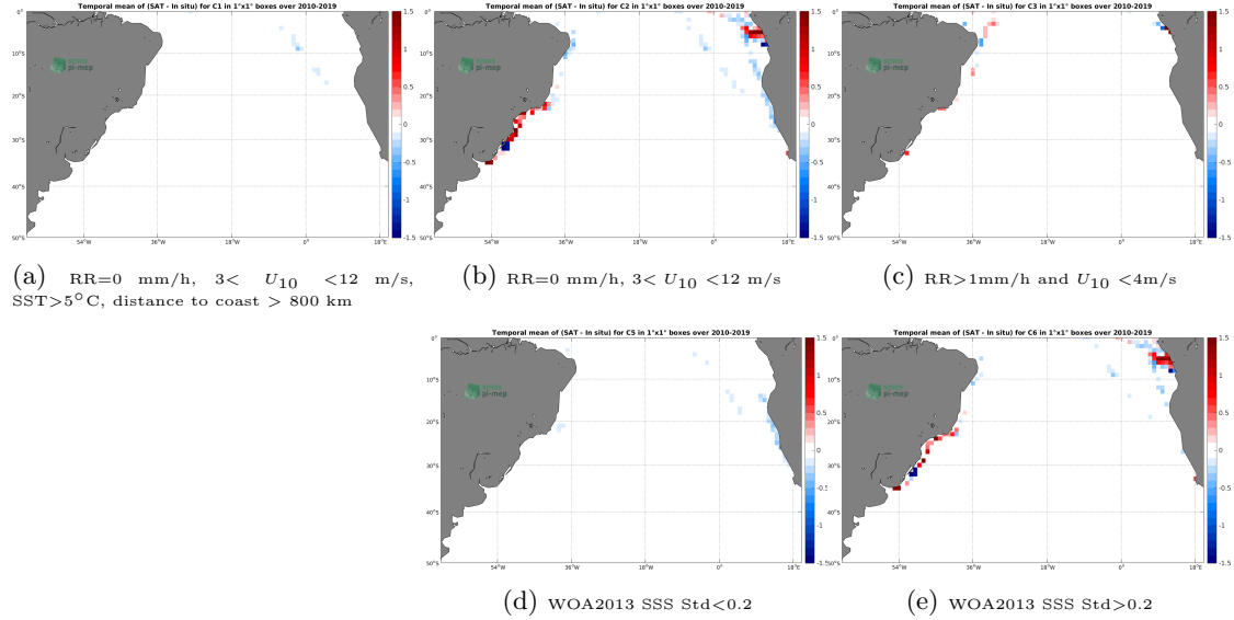
Figure 12: Temporal mean gridded over spatial boxes of size 1^{\circ}\times 1^{\circ} of \Delta\text{SSS} (CCI SSS L4 Merged-OI v2.31 - 30-day running (ESA) - TSG (LEGOS-DM)) for 5 different subdatasets corresponding to:RR=0 mm/h, 3 < U_{10} < 12 m/s, SST >5^{\circ}\text{C} , distance to coast > 800 km (a), RR=0 mm/h, 3 < U_{10} < 12 m/s (b), RR >1 mm/h and U_{10} < 4 m/s (c), WOA2013 SSS Std <0.2 (d), WOA2013 SSS Std >0.2 (e).
