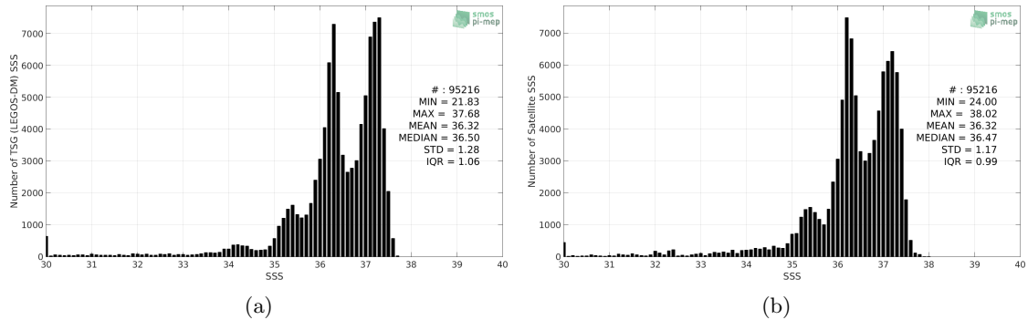
Figure 2: Histograms of SSS from TSG (LEGOS-DM) (a) and CCI SSS L4 Merged-OI v2.31 - 30-day running (ESA) (b) considering all match-up pairs per bins of 0.1 over the South Atlantic Ocean Pi-MEP region and for the full satellite product period.
