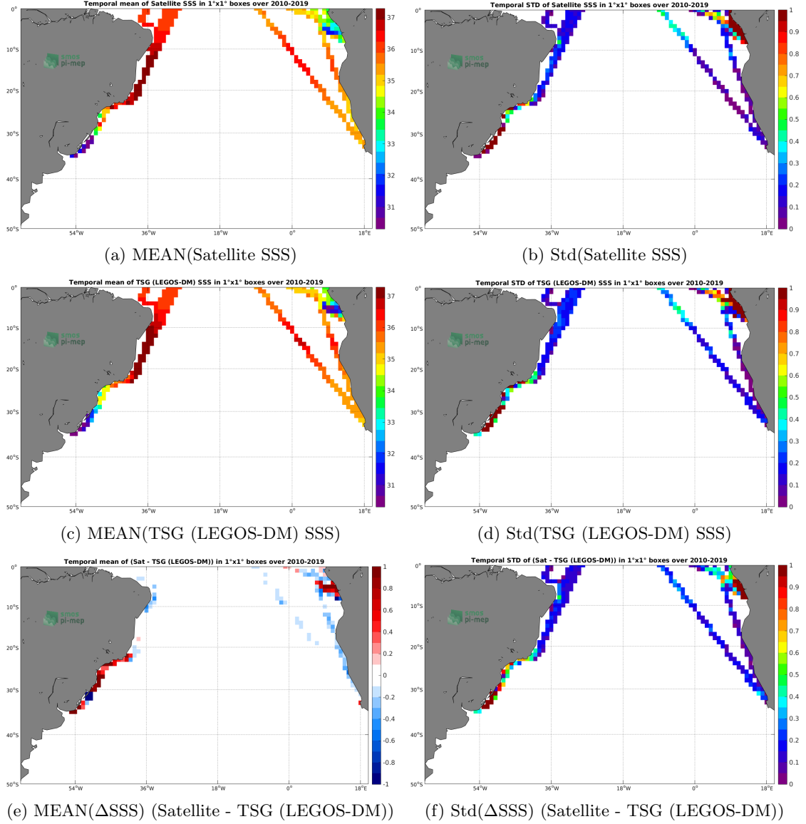
Figure 6: Temporal mean (left) and Std (right) of SSS from CCI SSS L4 Merged-OI v2.31 - 30-day running (ESA) (top), TSG (LEGOS-DM) (middle), and of \Delta SSS (Satellite - TSG (LEGOS-DM)). Only match-up pairs are used to generate these maps.
