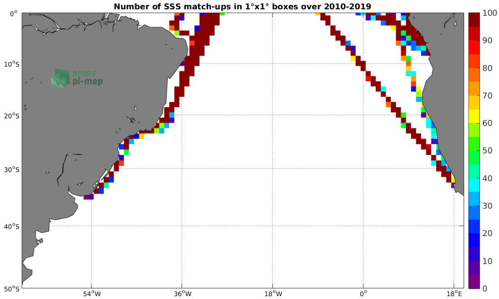
Figure 4: Number of SSS match-ups between TSG (LEGOS-DM) SSS and the CCI L4 Merged-OI v2.31 - 30-day running (ESA) SSS product for the South Atlantic Ocean Pi-MEP region over 1^\circ \times 1^\circ boxes and for the full satellite product period.
