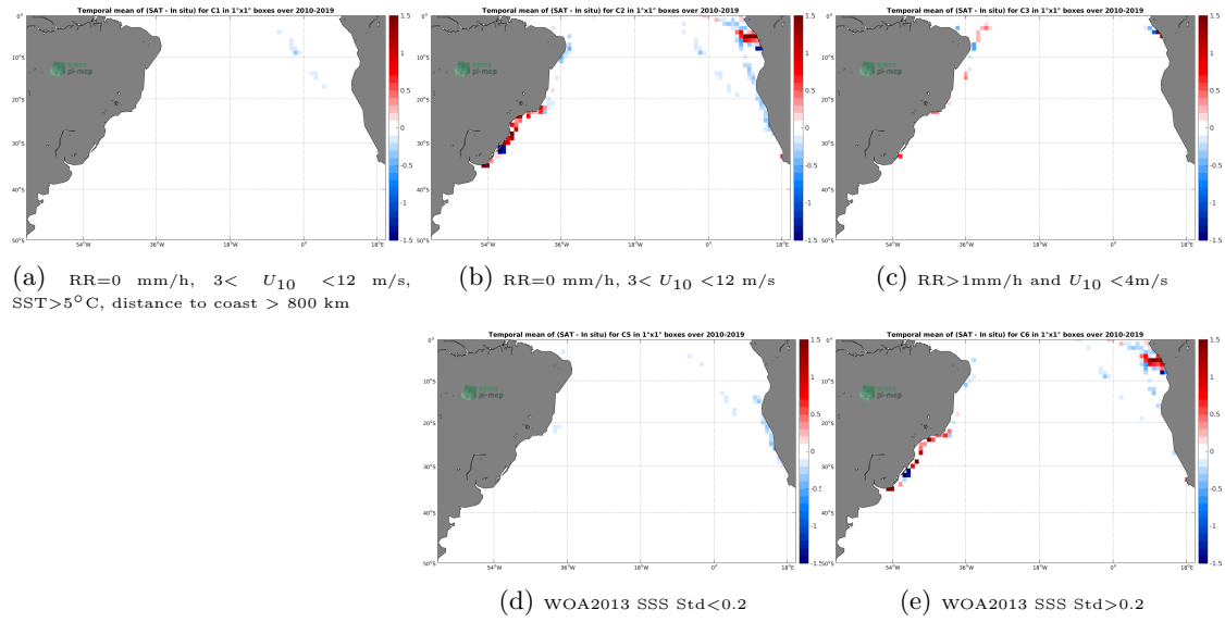
Figure 12: Temporal mean gridded over spatial boxes of size 1^\circ \times 1^\circ of \Delta SSS (CCI L4 Merged-OI v2.31 - 30-day running (ESA) - TSG (LEGOS-DM)) for 5 different subdatasets corresponding to: RR=0 mm/h, 3 < U_{10} < 12 m/s, SST >5^\circ\text{C} , distance to coast > 800 km (a), RR=0 mm/h, 3 < U_{10} < 12 m/s (b), RR >1 mm/h and U_{10} < 4 m/s (c), WOA2013 SSS Std <0.2 (d), WOA2013 SSS Std >0.2 (e).
