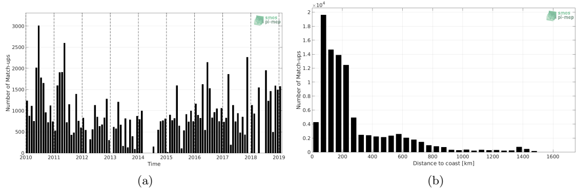
Figure 1: Number of match-ups between TSG (LEGOS-DM) and CCI L4 Merged-OI v2.31 - 30-day running (ESA) SSS as a function of time (a) and as function of the distance to coast (b) over the South Atlantic Ocean Pi-MEP region and for the full satellite product period.
