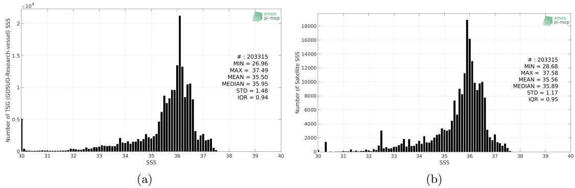
Figure 2: Histograms of SSS from TSG (GOSUD-Research-vessel) (a) and CCI SSS L4 Merged-OI v2.31 - 30-day running (ESA) (b) considering all match-up pairs per bins of 0.1 over the South Atlantic Ocean Pi-MEP region and for the full satellite product period.
