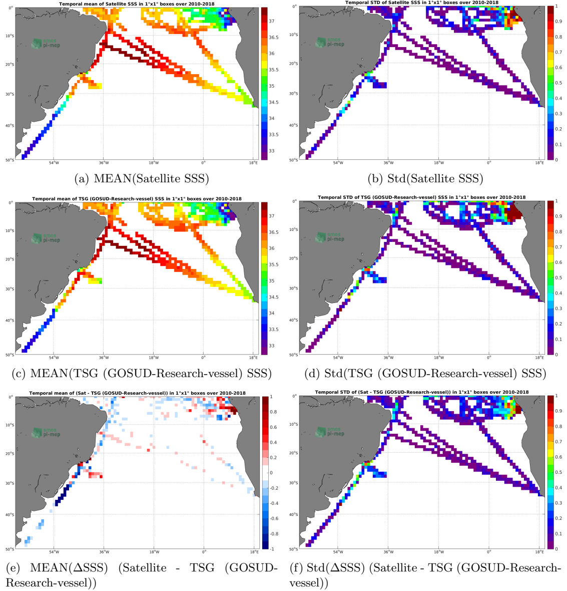
Figure 6: Temporal mean (left) and Std (right) of SSS from CCI SSS L4 Merged-OI v2.31 - 30-day running (ESA) (top), TSG (GOSUD-Research-vessel) (middle), and of \Delta SSS (Satellite - TSG (GOSUD-Research-vessel)). Only match-up pairs are used to generate these maps.
