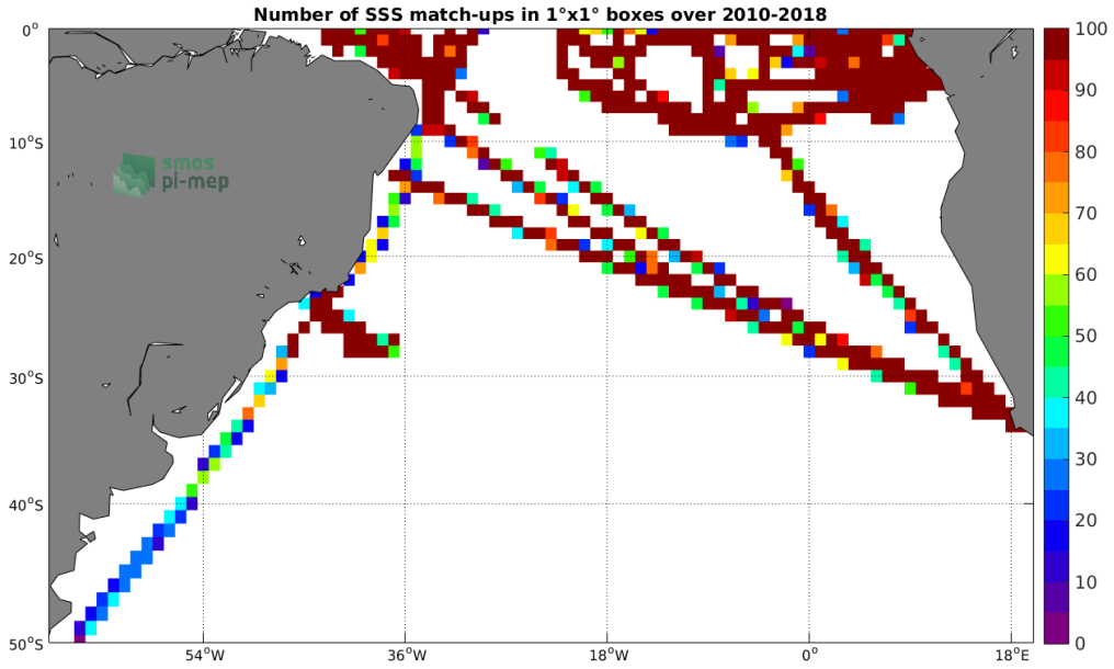
Figure 4: Number of SSS match-ups between TSG (GOSUD-Research-vessel) SSS and the CCI SSS L4 Merged-OI v2.31 - 30-day running (ESA) SSS product for the South Atlantic Ocean Pi-MEP region over 1^\circ \times 1^\circ boxes and for the full satellite product period.
