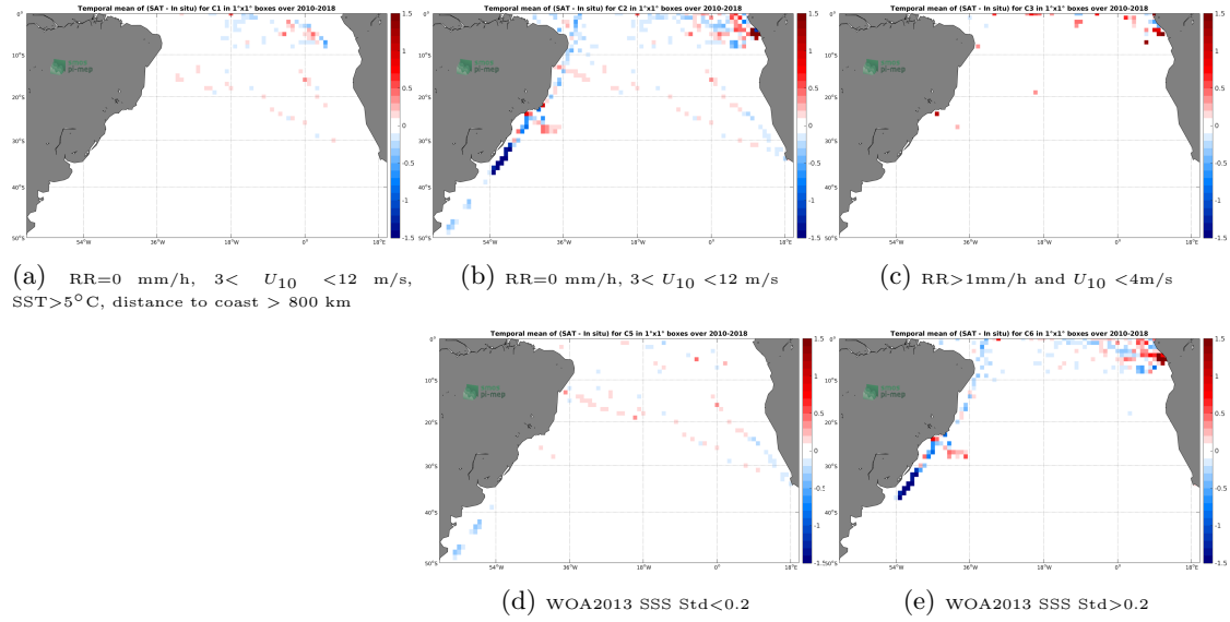
Figure 12: Temporal mean gridded over spatial boxes of size 1^\circ \times 1^\circ of \Delta SSS (CCI SSS L4 Merged-OI v2.31 - 30-day running (ESA) - TSG (GOSUD-Research-vessel)) for 5 different subdatasets corresponding to: RR=0 mm/h, 3 < U_{10} < 12 m/s, SST > 5^\circ C , distance to coast > 800 km (a), RR=0 mm/h, 3 < U_{10} < 12 m/s (b), RR > 1 mm/h and U_{10} < 4 m/s (c), WOA2013 SSS Std < 0.2 (d), WOA2013 SSS Std > 0.2 (e).
