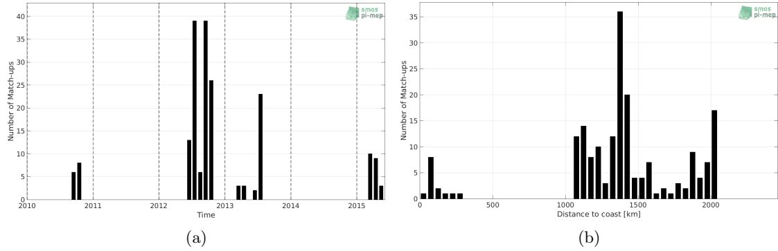
Figure 1: Number of match-ups between Sea mammals and CCI L4 Merged-OI v2.31 - 30-day running (ESA) SSS as a function of time (a) and as function of the distance to coast (b) over the South Atlantic Ocean Pi-MEP region and for the full satellite product period.
