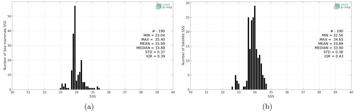
Figure 2: Histograms of SSS from Sea mammals (a) and CCI L4 Merged-OI v2.31 - 30-day running (ESA) (b) considering all match-up pairs per bins of 0.1 over the South Atlantic Ocean Pi-MEP region and for the full satellite product period.
