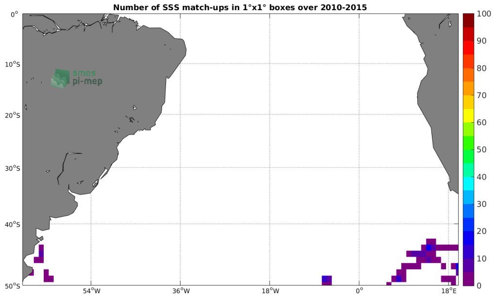
Figure 4: Number of SSS match-ups between Sea mammals SSS and the CCI L4 Merged-OI v2.31 - 30-day running (ESA) SSS product for the South Atlantic Ocean Pi-MEP region over 1^\circ \times 1^\circ boxes and for the full satellite product period.
