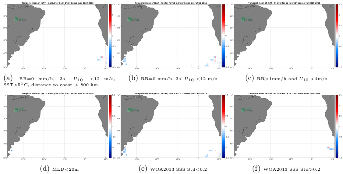
Figure 12: Temporal mean gridded over spatial boxes of size 1^{\circ}\times 1^{\circ} of \Delta\text{SSS} (CCI L4 Merged-OI v2.31 - 30-day running (ESA) - Sea mammals) for 6 different subdatasets corresponding to: \text{RR}=0 mm/h, 3 < U_{10} < 12 m/s, \text{SST} > 5^{\circ}\text{C} , distance to coast > 800 km (a), \text{RR}=0 mm/h, 3 < U_{10} < 12 m/s (b), \text{RR} > 1\text{mm/h} and U_{10} < 4\text{m/s} (c), \text{MLD} < 20\text{m} (d), \text{WOA2013 SSS Std} < 0.2 (e), \text{WOA2013 SSS Std} > 0.2 (f).
