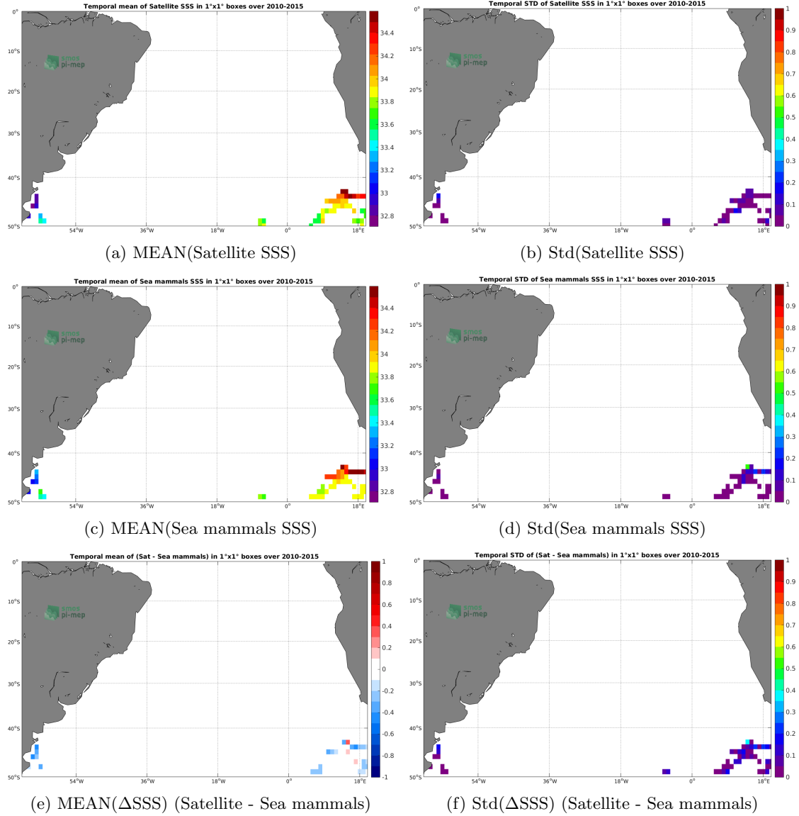
Figure 6: Temporal mean (left) and Std (right) of SSS from CCI L4 Merged-OI v2.31 - 30-day running (ESA) (top), Sea mammals (middle), and of \Delta SSS (Satellite - Sea mammals). Only match-up pairs are used to generate these maps.
