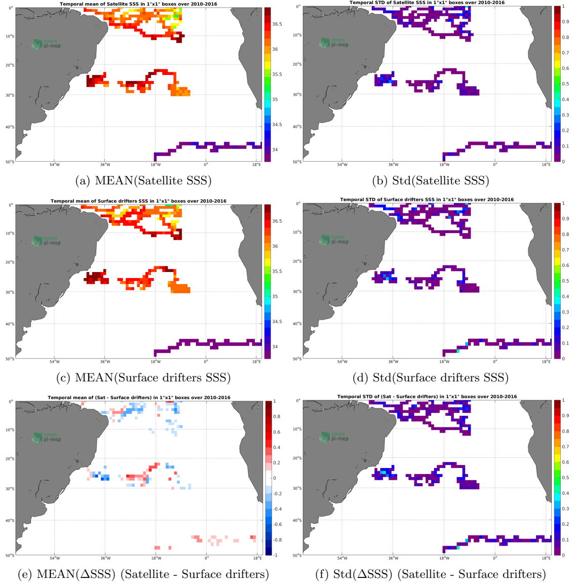
Figure 5: Temporal mean (left) and Std (right) of SSS from CCI SSS L4 Merged-OI v2.31 - 30-day running (ESA) (top), Surface drifters (middle), and of \Delta SSS (Satellite - Surface drifters). Only match-up pairs are used to generate these maps.
