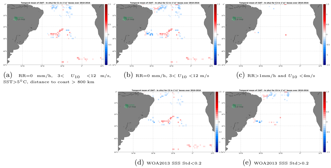
Figure 11: Temporal mean gridded over spatial boxes of size 1^\circ \times 1^\circ of \Delta SSS (CCI SSS L4 Merged-OI v2.31 - 30-day running (ESA) - Surface drifters) for 5 different subdatasets corresponding to:RR=0 mm/h, 3 < U_{10} < 12 m/s, SST >5^\circ\text{C} , distance to coast > 800 km (a), RR=0 mm/h, 3 < U_{10} < 12 m/s (b), RR >1 mm/h and U_{10} < 4 m/s (c), WOA2013 SSS Std <0.2 (d), WOA2013 SSS Std >0.2 (e).
