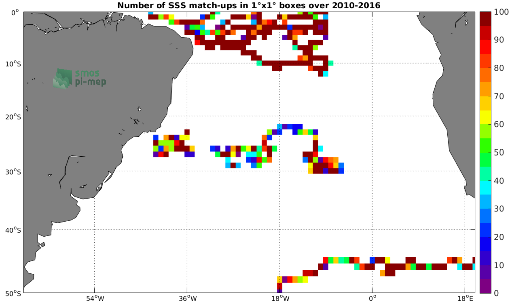
Figure 3: Number of SSS match-ups between Surface drifters SSS and the CCI SSS L4 Merged-OI v2.31 - 30-day running (ESA) SSS product for the South Atlantic Ocean Pi-MEP region over 1^\circ \times 1^\circ boxes and for the full satellite product period.
