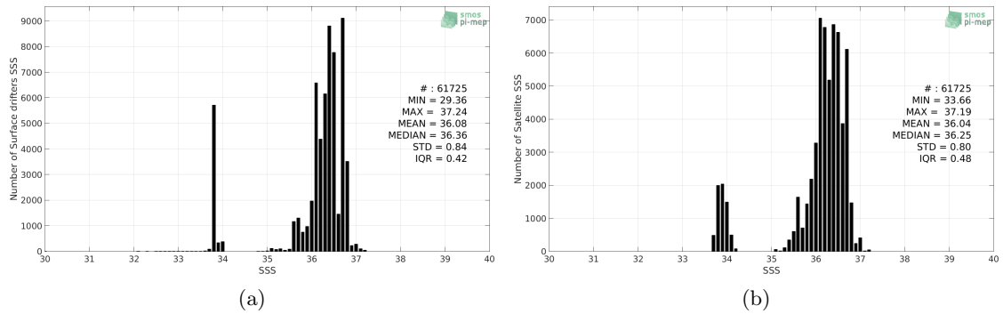
Figure 2: Histograms of SSS from Surface drifters (a) and CCI SSS L4 Merged-OI v2.31 - 30-day running (ESA) (b) considering all match-up pairs per bins of 0.1 over the South Atlantic Ocean Pi-MEP region and for the full satellite product period.
