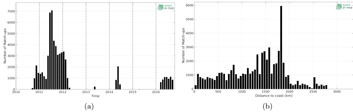
Figure 1: Number of match-ups between Surface drifters and CCI L4 Merged-OI v2.31 - 30-day running (ESA) SSS as a function of time (a) and as function of the distance to coast (b) over the South Atlantic Ocean Pi-MEP region and for the full satellite product period.
