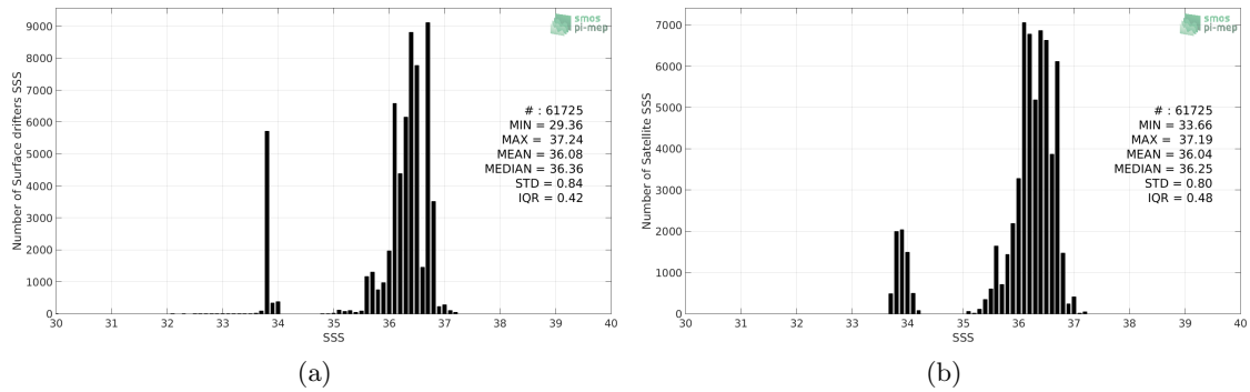
Figure 2: Histograms of SSS from Surface drifters (a) and CCI L4 Merged-OI v2.31 - 30-day running (ESA) (b) considering all match-up pairs per bins of 0.1 over the South Atlantic Ocean Pi-MEP region and for the full satellite product period.
