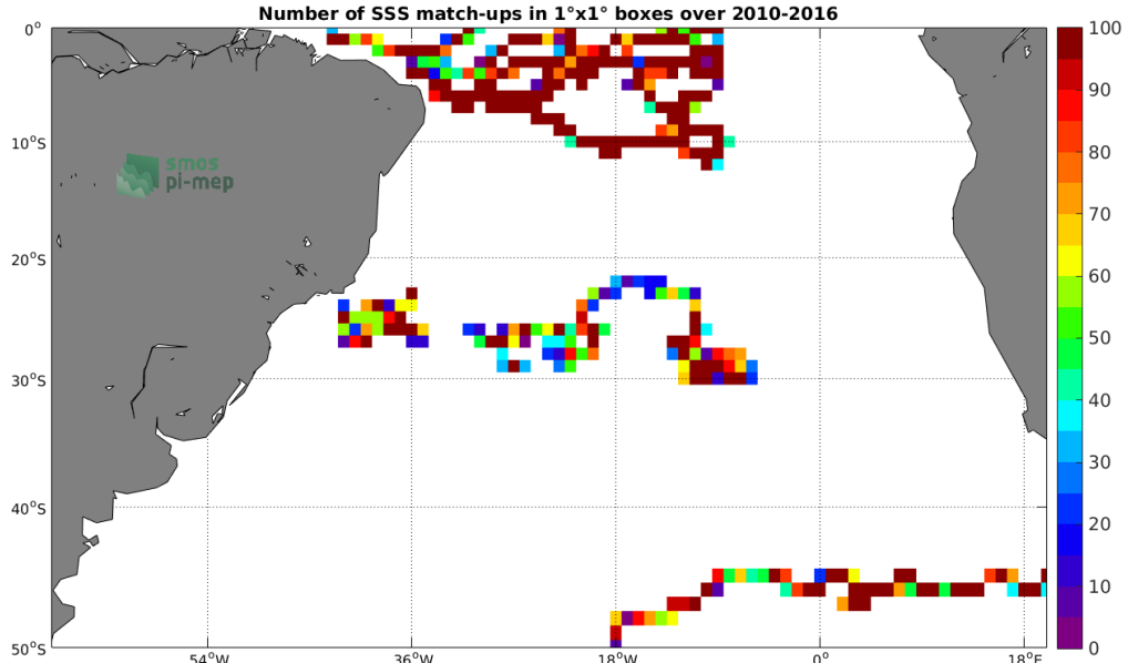
Figure 3: Number of SSS match-ups between Surface drifters SSS and the CCI L4 Merged-OI v2.31 - 30-day running (ESA) SSS product for the South Atlantic Ocean Pi-MEP region over 1^\circ \times 1^\circ boxes and for the full satellite product period.
