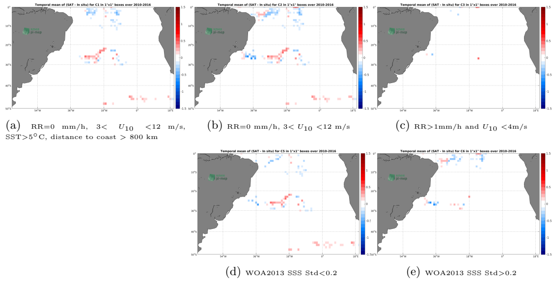
Figure 11: Temporal mean gridded over spatial boxes of size 1^\circ \times 1^\circ of \Delta SSS (CCI L4 Merged-OI v2.31 - 30-day running (ESA) - Surface drifters) for 5 different subdatasets corresponding to: RR=0 mm/h, 3 < U_{10} < 12 m/s, SST >5^\circ\text{C} , distance to coast > 800 km (a), RR=0 mm/h, 3 < U_{10} < 12 m/s (b), RR >1 mm/h and U_{10} < 4 m/s (c), WOA2013 SSS Std <0.2 (d), WOA2013 SSS Std >0.2 (e).
