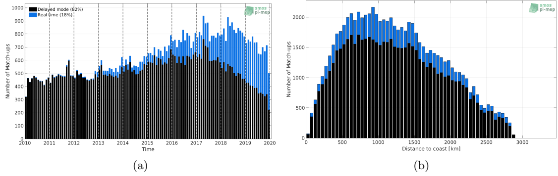
Figure 1: Number of match-ups between Argo and CCI L4 Merged-OI v2.31 - 30-day running (ESA) SSS as a function of time (a) and as function of the distance to coast (b) over the South Atlantic Ocean Pi-MEP region and for the full satellite product period.
