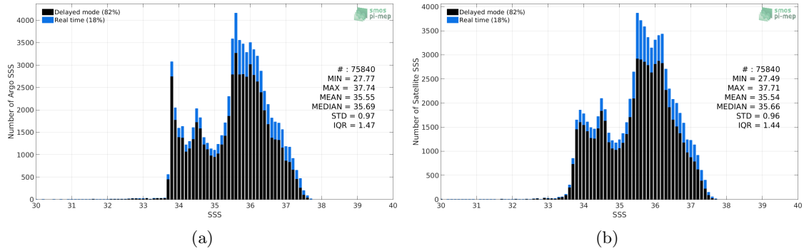
Figure 2: Histograms of SSS from Argo (a) and CCI L4 Merged-OI v2.31 - 30-day running (ESA) (b) considering all match-up pairs per bins of 0.1 over the South Atlantic Ocean Pi-MEP region and for the full satellite product period.
