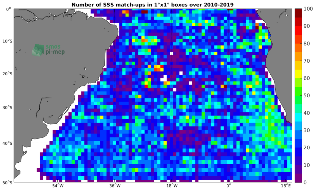
Figure 4: Number of SSS match-ups between Argos SSS and the CCI L4 Merged-OI v2.31 - 30-day running (ESA) SSS product for the South Atlantic Ocean Pi-MEP region over 1°x1° boxes and for the full satellite product period.
