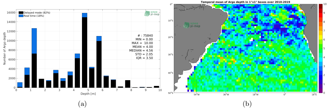
Figure 3: Histograms of the depth of the upper level SSS measurements from Argos in the Match-up DataBase for the South Atlantic Ocean Pi-MEP region (a) and temporal mean spatial distribution of pressure of the in situ SSS data over 1°x1° boxes and for the full satellite product period (b).
