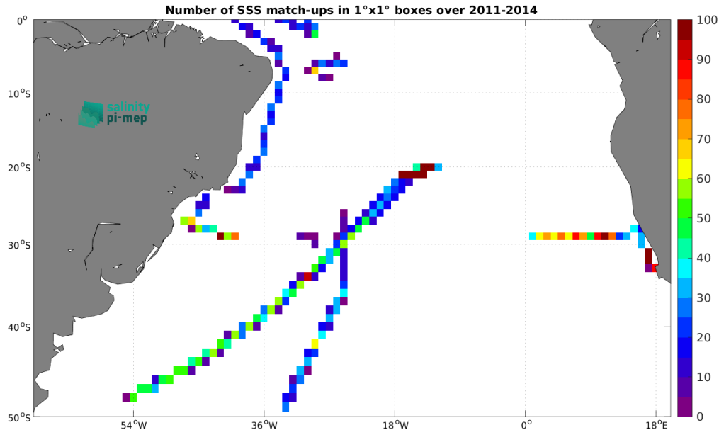
Figure 5: Number of SSS match-ups between TSG (SAMOS) SSS and the Aquarius SSS L4 OI v5 - Weekly (IPRC) SSS product for the South Atlantic Ocean Pi-MEP region over 1^\circ \times 1^\circ boxes and for the full satellite product period.
