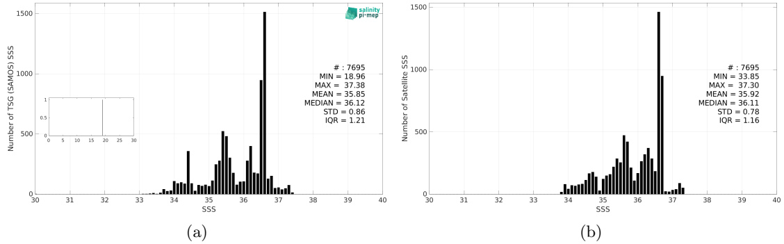
Figure 3: Histograms of SSS from TSG (SAMOS) (a) and Aquarius SSS L4 OI v5 - Weekly (IPRC) (b) considering all match-up pairs per bins of 0.1 over the South Atlantic Ocean Pi-MEP region and for the full satellite product period.
