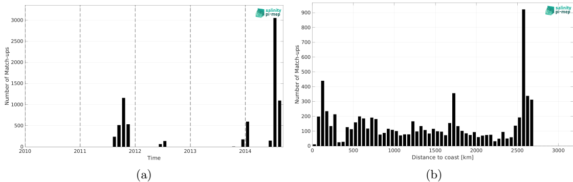
Figure 2: Number of match-ups between TSG (SAMOS) and Aquarius SSS L4 OI v5 - Weekly (IPRC) SSS as a function of time (a) and as function of the distance to coast (b) over the South Atlantic Ocean Pi-MEP region and for the full satellite product period.
