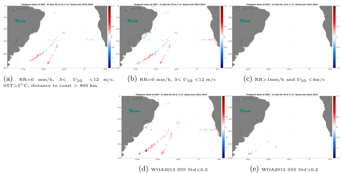
Figure 14: Temporal mean gridded over spatial boxes of size 1^\circ \times 1^\circ of \Delta SSS (Aquarius SSS L4 OI v5 - Weekly (IPRC) - TSG (SAMOS)) for 5 different subdatasets corresponding to:RR=0 mm/h, 3 < U_{10} < 12 m/s, SST >5^\circ\text{C} , distance to coast > 800 km (a), RR=0 mm/h, 3 < U_{10} < 12 m/s (b), RR >1 mm/h and U_{10} < 4 m/s (c), WOA2013 SSS Std <0.2 (d), WOA2013 SSS Std >0.2 (e).
