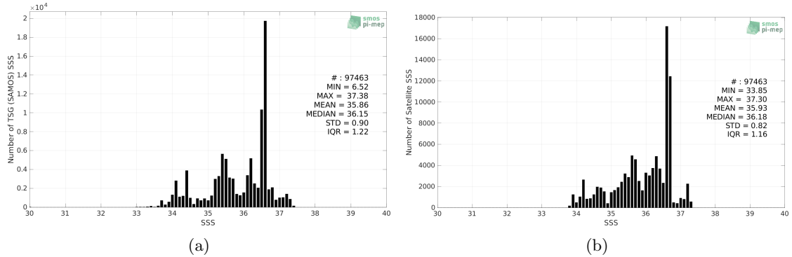
Figure 2: Histograms of SSS from TSG (SAMOS) (a) and Aquarius SSS L4 OI v5 - Weekly (IPRC) (b) considering all match-up pairs per bins of 0.1 over the South Atlantic Ocean Pi-MEP region and for the full satellite product period.
