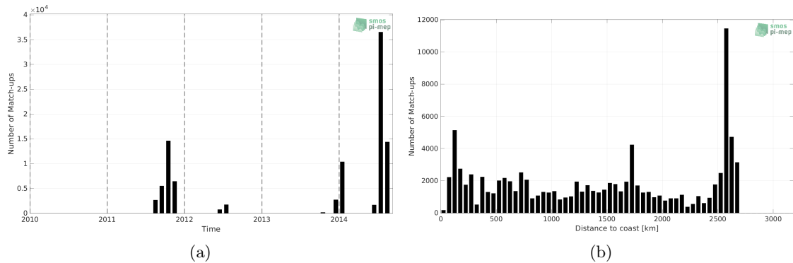
Figure 1: Number of match-ups between TSG (SAMOS) and Aquarius SSS L4 OI v5 - Weekly (IPRC) SSS as a function of time (a) and as function of the distance to coast (b) over the South Atlantic Ocean Pi-MEP region and for the full satellite product period.
