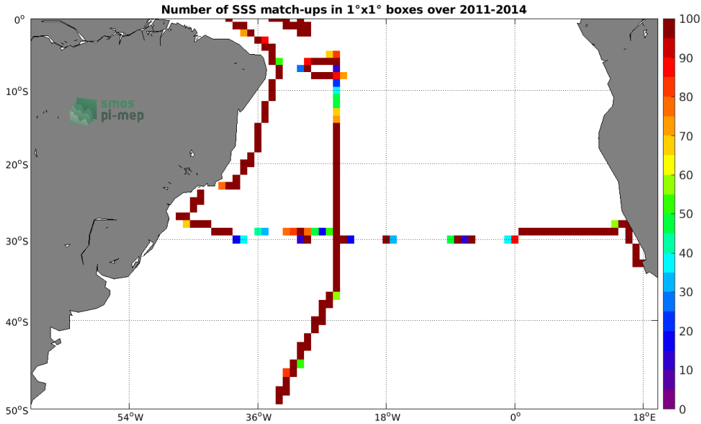
Figure 4: Number of SSS match-ups between TSG (SAMOS) SSS and the Aquarius SSS L4 OI v5 - Weekly (IPRC) SSS product for the South Atlantic Ocean Pi-MEP region over 1^\circ \times 1^\circ boxes and for the full satellite product period.
