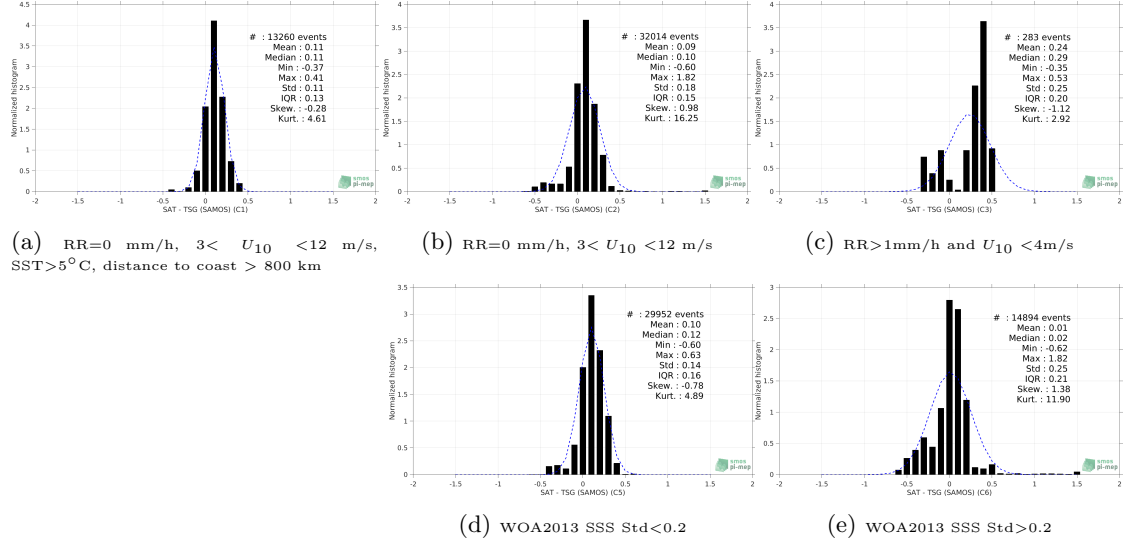
Figure 13: Normalized histogram of \Delta SSS (Aquarius SSS L4 OI v5 - Weekly (IPRC) - TSG (SAMOS)) for 5 different subdatasets corresponding to: RR=0 mm/h, 3 < U_{10} < 12 m/s, SST > 5^\circ\text{C} , distance to coast > 800 km (a), RR=0 mm/h, 3 < U_{10} < 12 m/s (b), RR > 1 mm/h and U_{10} < 4 m/s (c), WOA2013 SSS Std < 0.2 (d), WOA2013 SSS Std > 0.2 (e).
