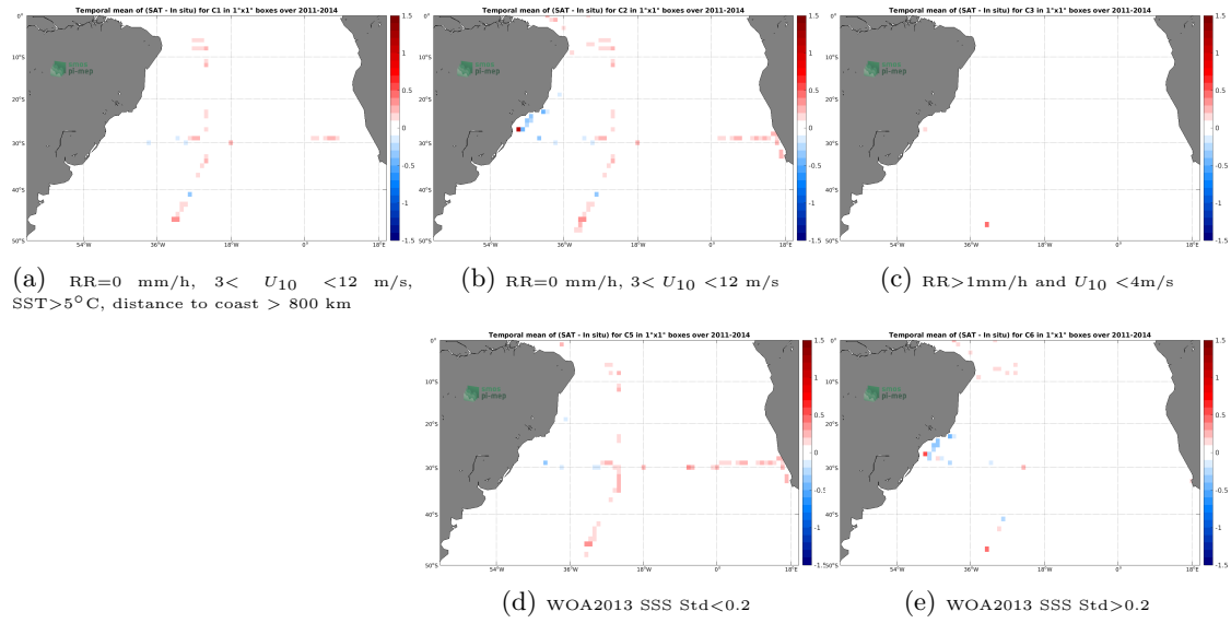
Figure 12: Temporal mean gridded over spatial boxes of size 1^\circ \times 1^\circ of \Delta SSS (Aquarius SSS L4 OI v5 - Weekly (IPRC) - TSG (SAMOS)) for 5 different subdatasets corresponding to: RR=0 mm/h, 3 < U_{10} < 12 m/s, SST>5°C, distance to coast > 800 km (a), RR=0 mm/h, 3 < U_{10} < 12 m/s (b), RR>1mm/h and U_{10} < 4 m/s (c), WOA2013 SSS Std<0.2 (d), WOA2013 SSS Std>0.2 (e).
