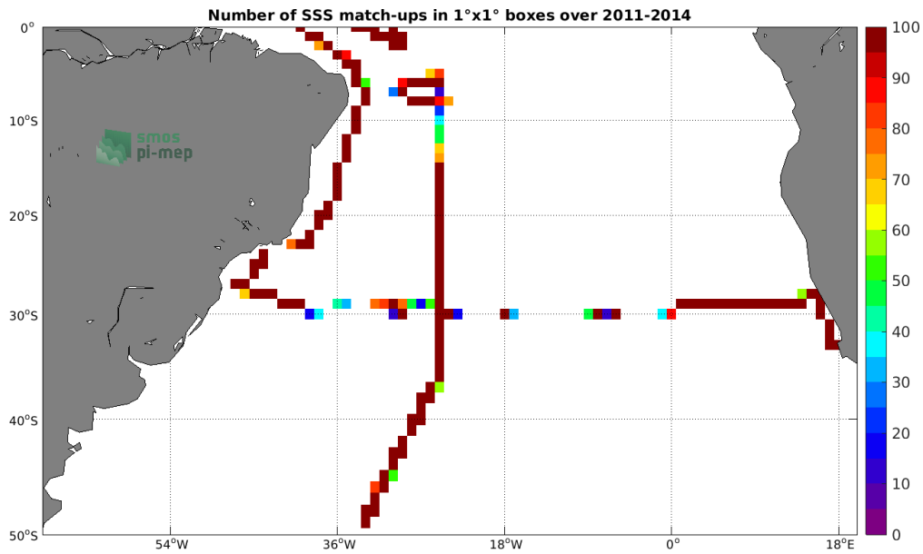
Figure 4: Number of SSS match-ups between TSG (SAMOS) SSS and the Aquarius SSS L4 OI v5 - Weekly (IPRC) SSS product for the South Atlantic Ocean Pi-MEP region over 1°x1° boxes and for the full satellite product period.
