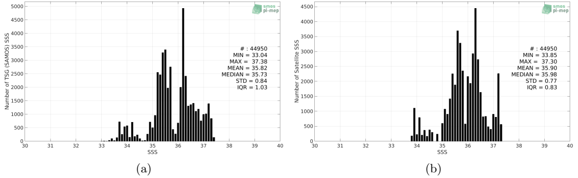
Figure 2: Histograms of SSS from TSG (SAMOS) (a) and Aquarius SSS L4 OI v5 - Weekly (IPRC) (b) considering all match-up pairs per bins of 0.1 over the South Atlantic Ocean Pi-MEP region and for the full satellite product period.
