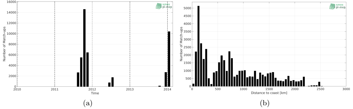
Figure 1: Number of match-ups between TSG (SAMOS) and Aquarius SSS L4 OI v5 - Weekly (IPRC) SSS as a function of time (a) and as function of the distance to coast (b) over the South Atlantic Ocean Pi-MEP region and for the full satellite product period.
