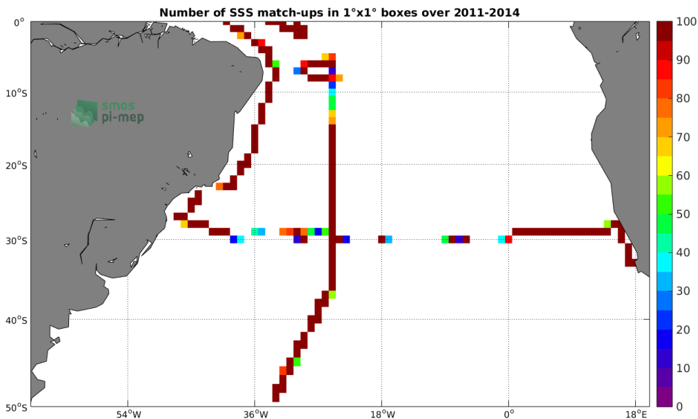
Figure 4: Number of SSS match-ups between TSG-SAMOS SSS and the Aquarius-L4-IPRC-V5-WEEKLY SSS product for the South Atlantic Ocean Pi-MEP region over 1^\circ \times 1^\circ boxes and for the full satellite product period.
