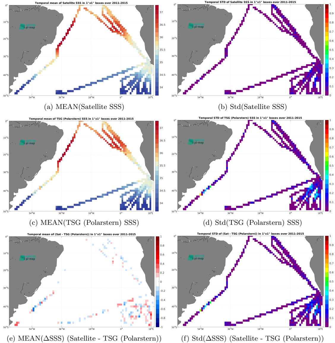
Figure 7: Temporal mean (left) and Std (right) of SSS from Aquarius SSS L4 OI v5 - Weekly (IPRC) (top), TSG (Polarstern) (middle), and of \Delta SSS (Satellite - TSG (Polarstern)). Only match-up pairs are used to generate these maps.
